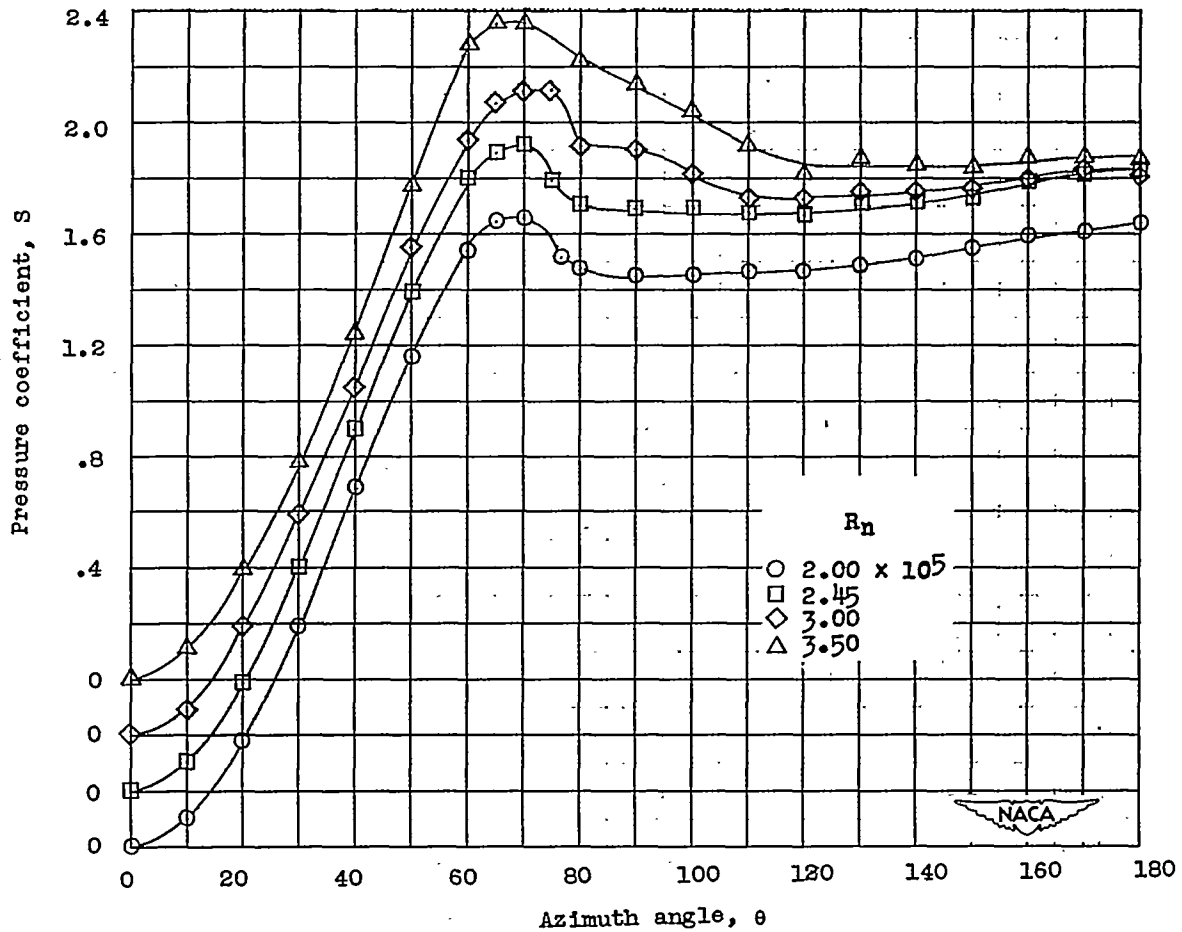
(a) R_n = 2.00 \times 10^5 to R_n = 3.50 \times 10^5 .
