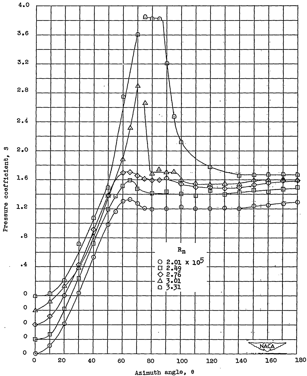
(a) R_n = 2.01 \times 10^5 to R_n = 3.31 \times 10^5 .
