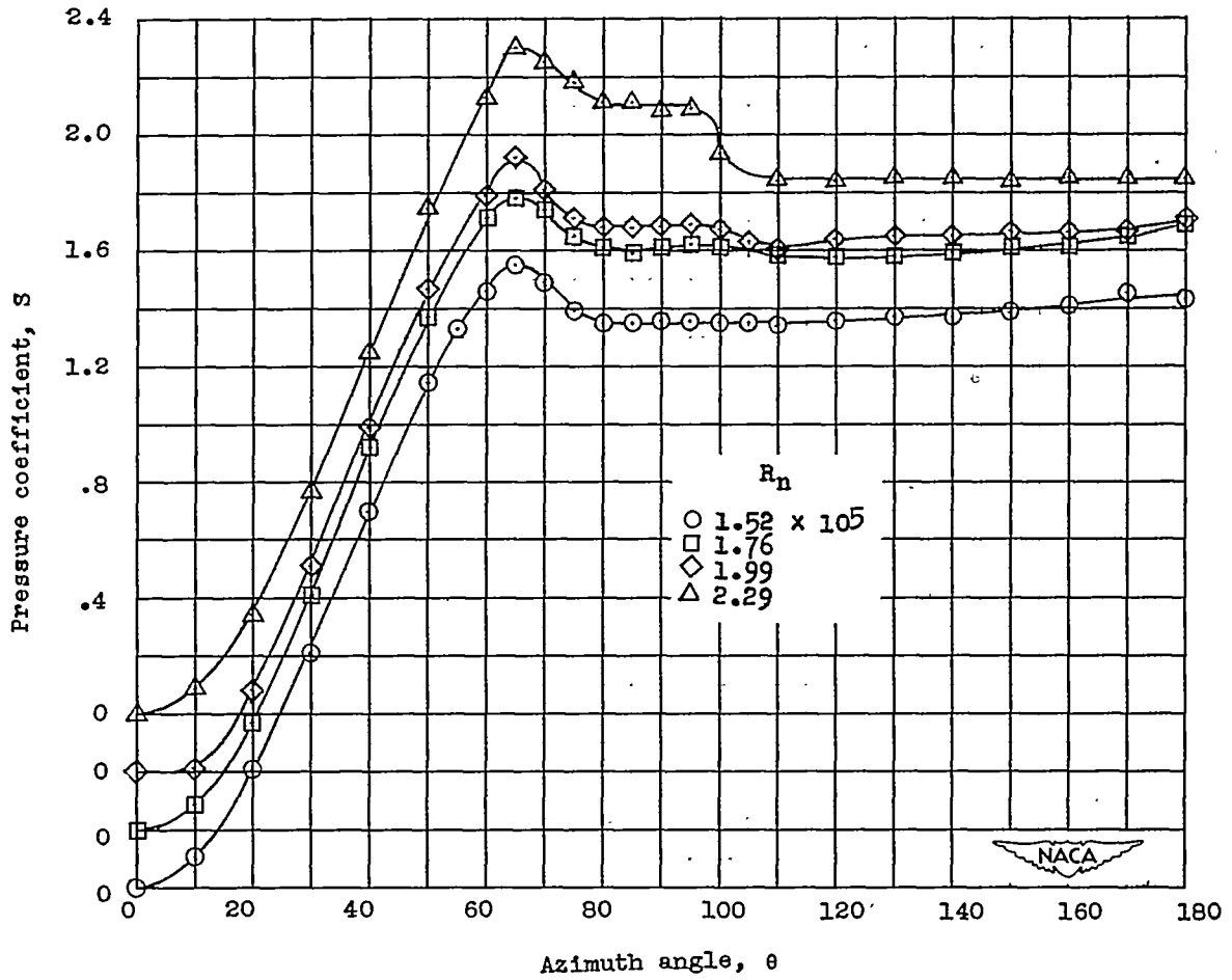
(a) R_n = 1.52 \times 10^5 to R_n = 2.29 \times 10^5 .
