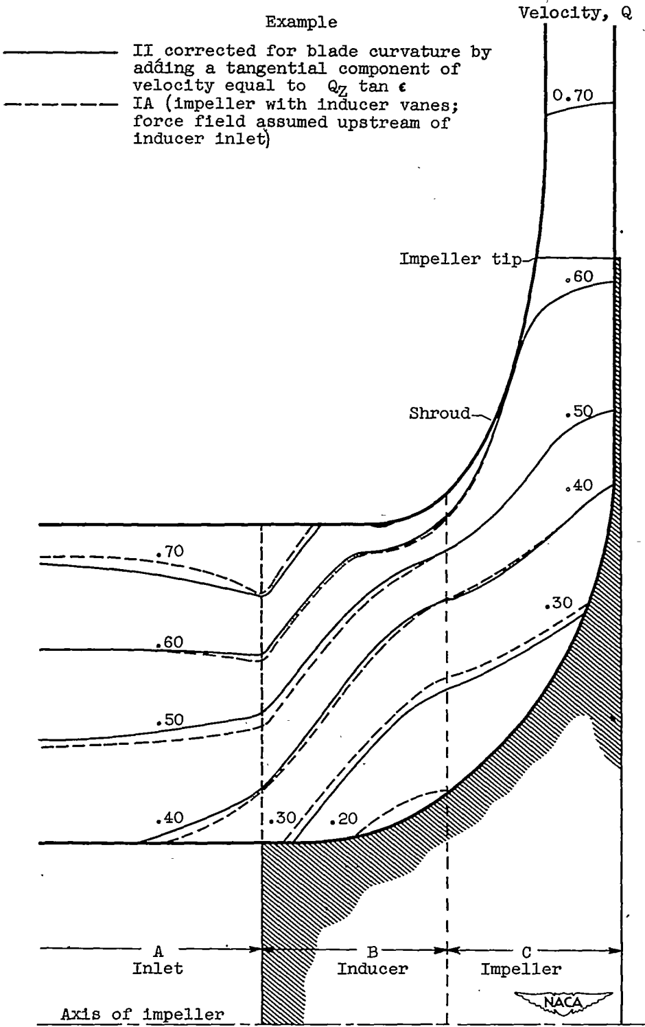
Figure 7. - Relative velocities in impeller without blade curvature corrected for impeller having blade curvature. Incompressible flow; Q_z equal to 0.3429 far upstream of impeller.
