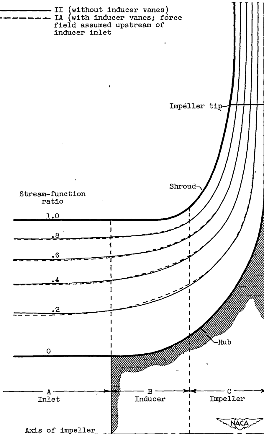
Figure 4. - Comparison of streamlines in meridional plane for axial-symmetry solutions of examples IA and II. Streamline designation indicates percentage of flow through compressor between streamline and impeller hub. Incompressible flow; Q_2 equal to 0.3429 far upstream of impeller.
