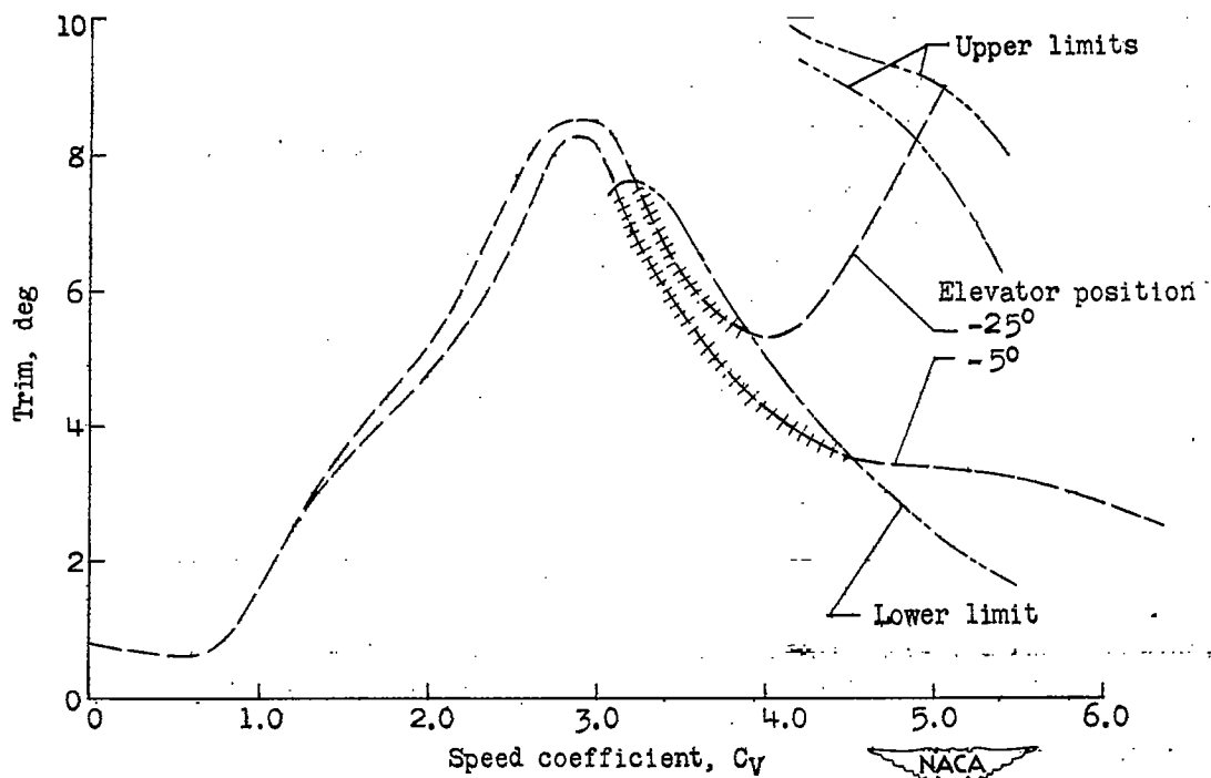
Figure 13.- Variation of trim with speed for conventional-hull model. Gross load coefficient, 0.94; center of gravity, 30 percent mean aerodynamic chord; full power.
