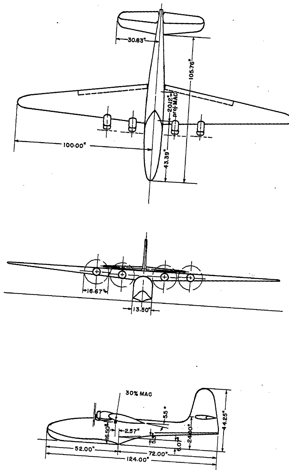
Figure 2.- General arrangement of the planing-tail model.
