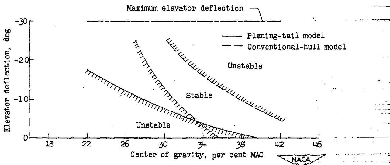
Figure 6.- Center-of-gravity limits of stability. Gross load coefficient, 0.94; full power.
