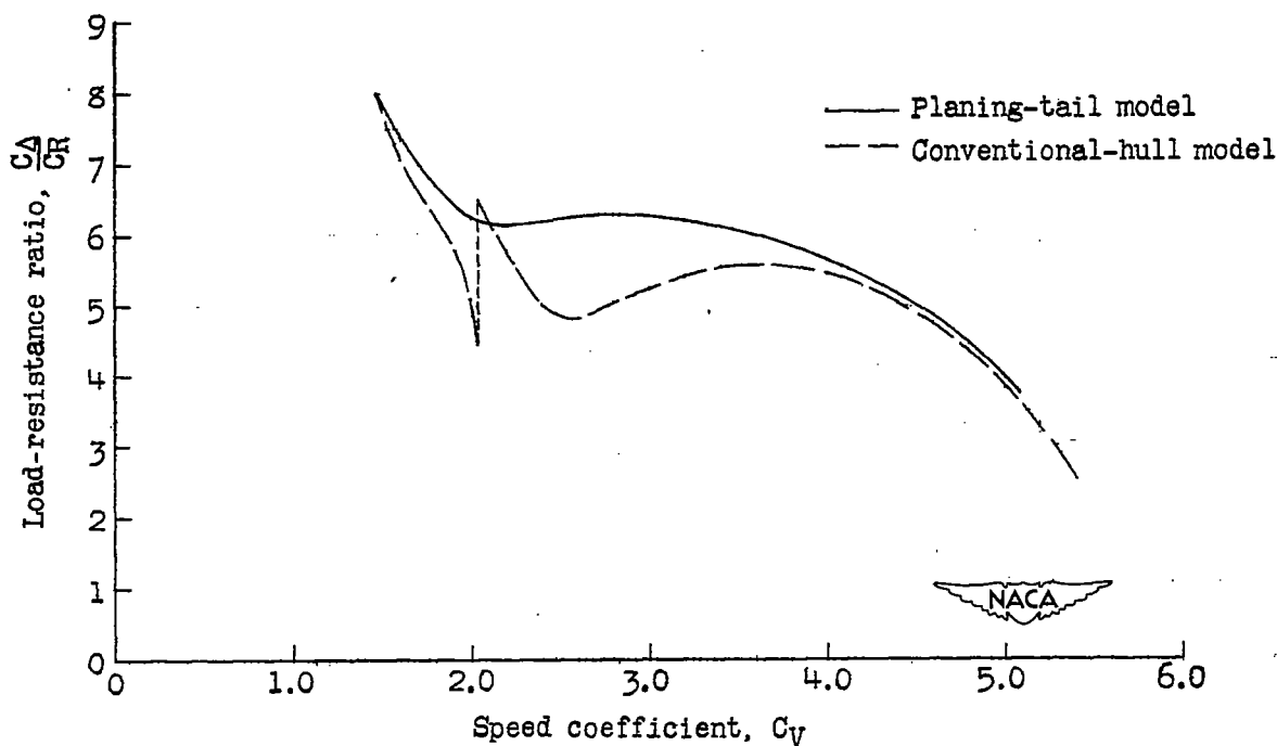
Figure 11.- Variation of load-resistance ratio with speed. Gross load coefficient, 0.94.
