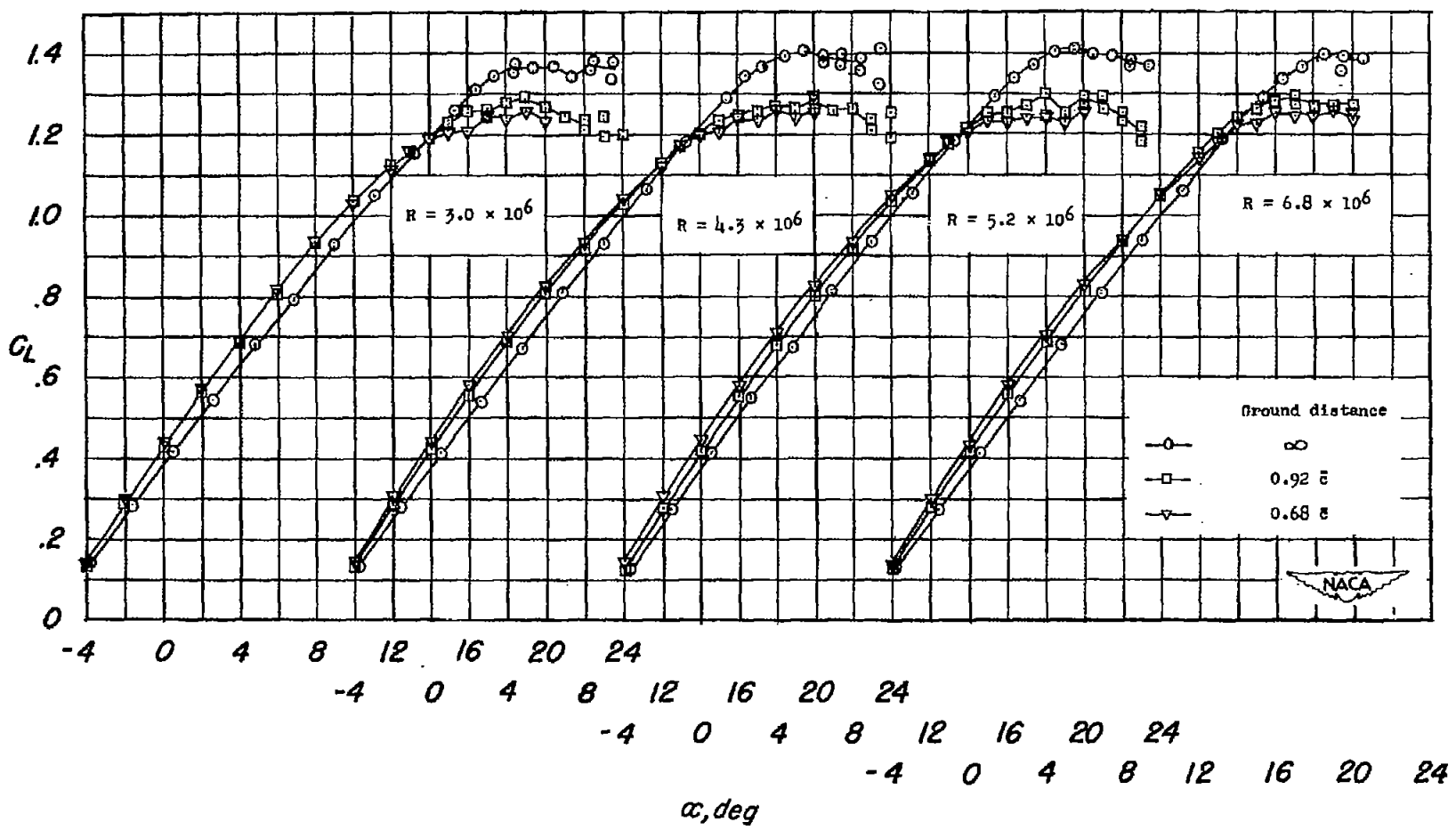
(a) Lift.
