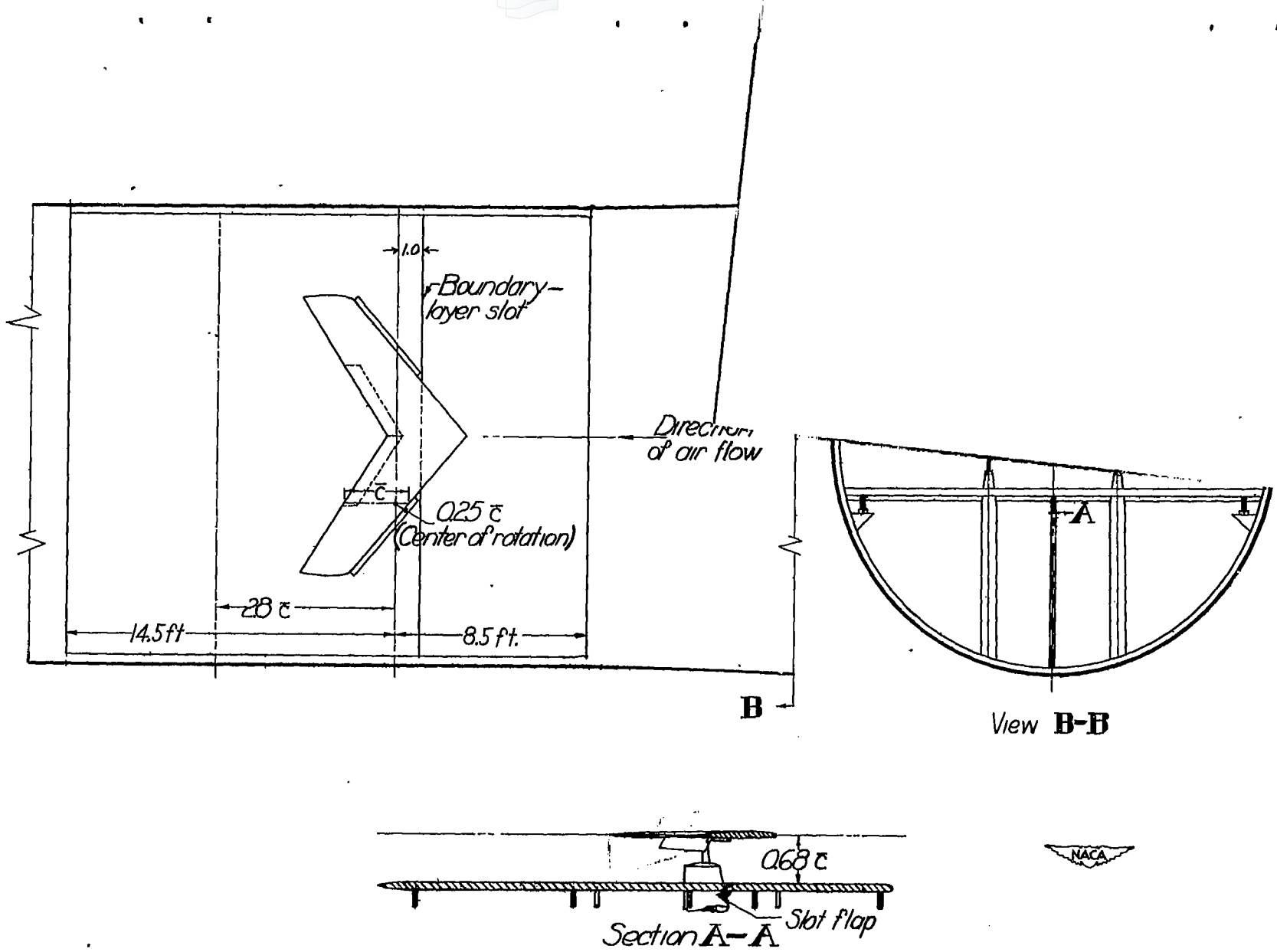
Figure 3.- Sketch of 42° sweptback wing and ground board used in the 19-foot pressure tunnel. Ground distance 0.68c.
