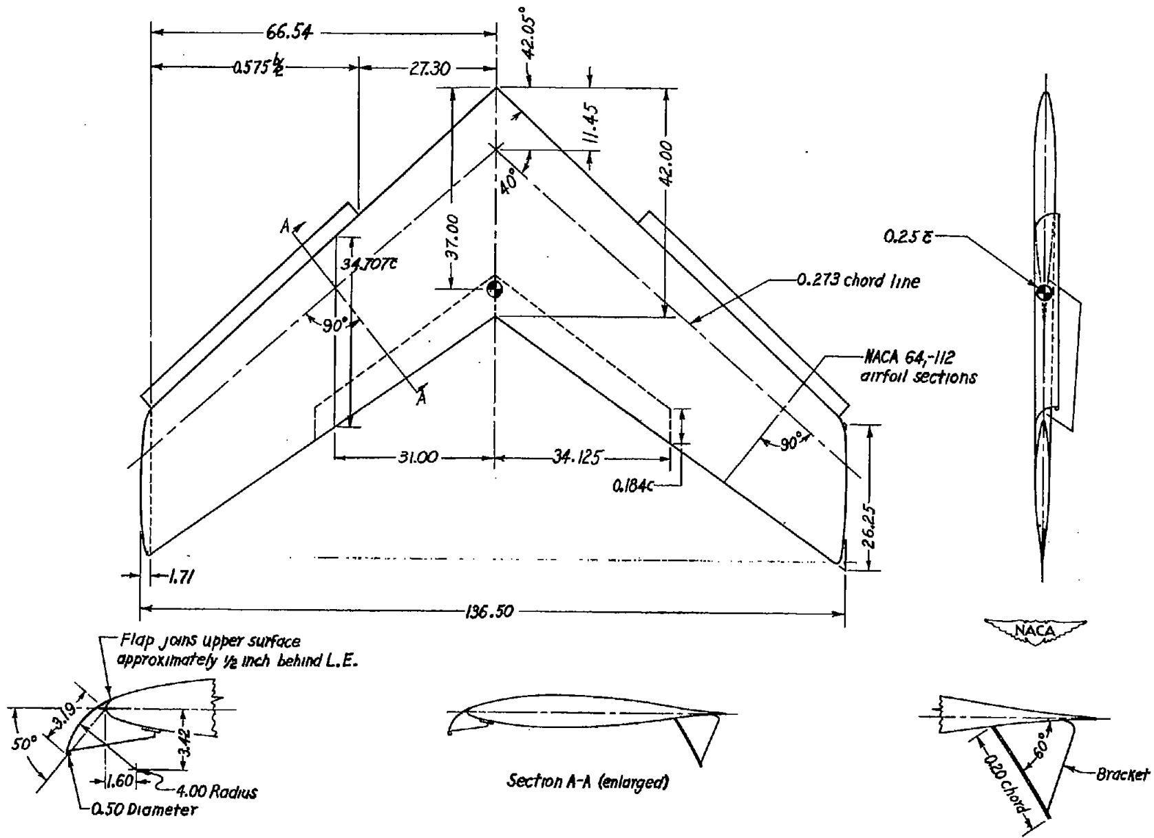
Figure 2.- Layout of 42° sweptback wing. (All dimensions are in inches.)
