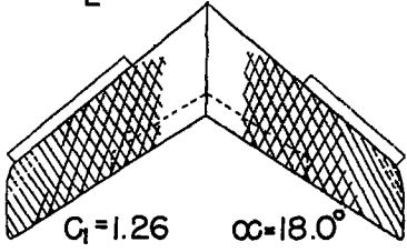
Figure 8.- Effect of ground on the stalling characteristics of a 42^\circ sweptback wing. Reynolds number = 6.8 \times 10^6 ; flaps deflected.
