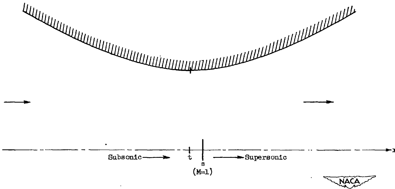
Figure 4. - Hyperbolic nozzle.
