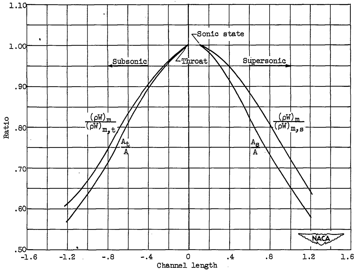
Figure 11. - Comparison of variation in mean specific mass flow and area ratio of nozzle with supersonic flow throughout divergent section.
