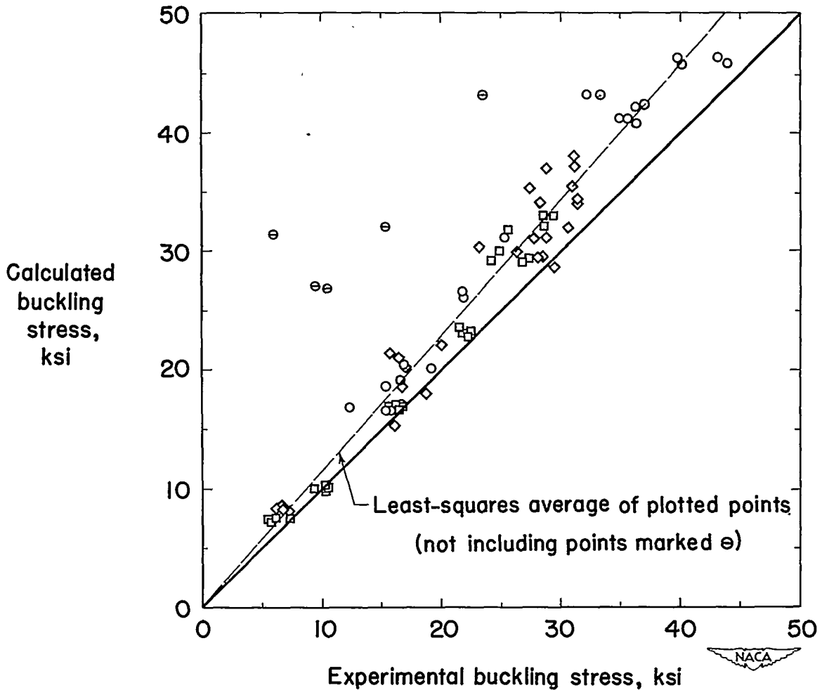
Figure 6.- Comparison of experimental buckling stresses of balsa-core sandwich plates with alclad 24S-T aluminum-alloy faces of reference 15 with calculated buckling stresses from theory of reference 13. (Dimensions shown are nominal thickness.)
