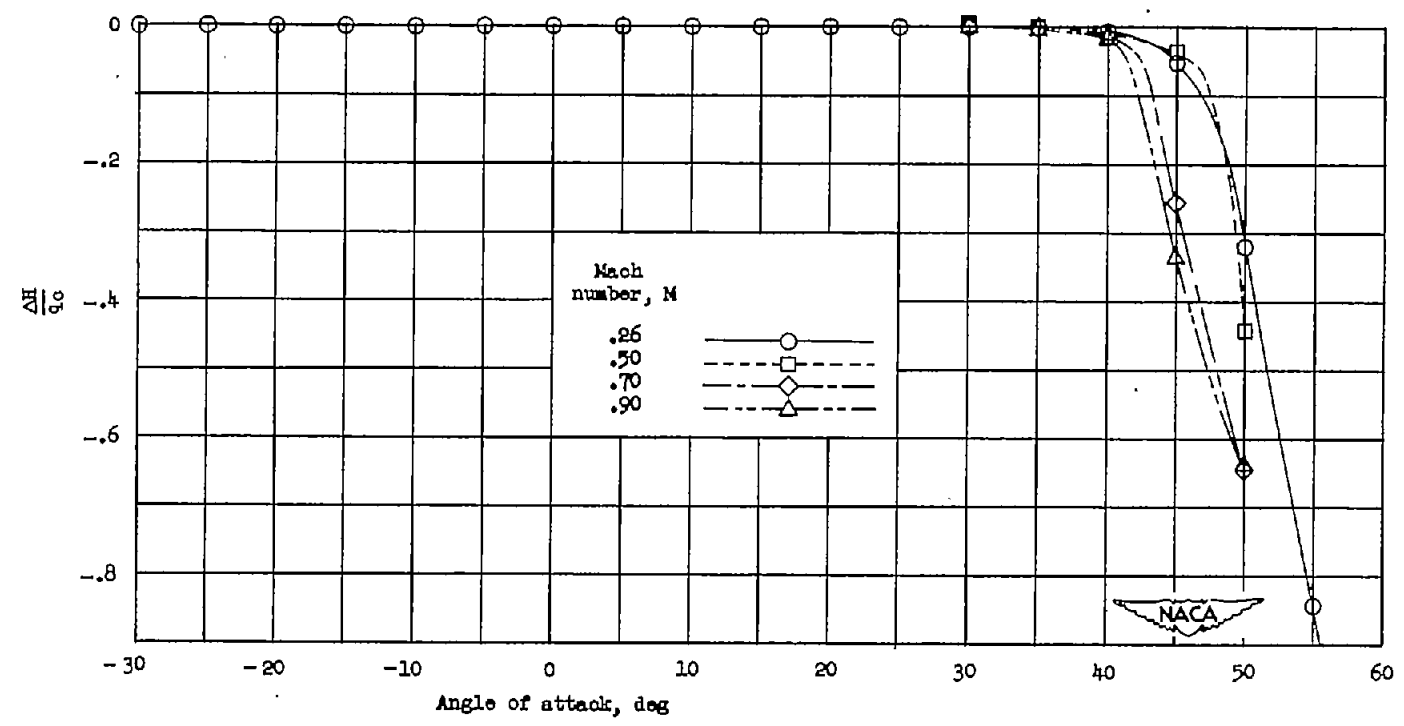
Figure 5.- Variation of total-pressure error with angle of attack. M = 0.26, 0.50, 0.70, and 0.90. Tube 1-a.
