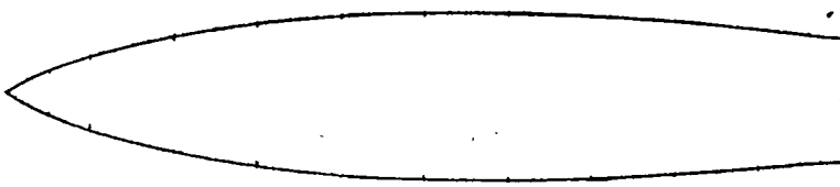
Figure 4.- Typical optimum body profiles which have given length, volume, and base diameter defined by equation (24). Thickness, 20 percent.
