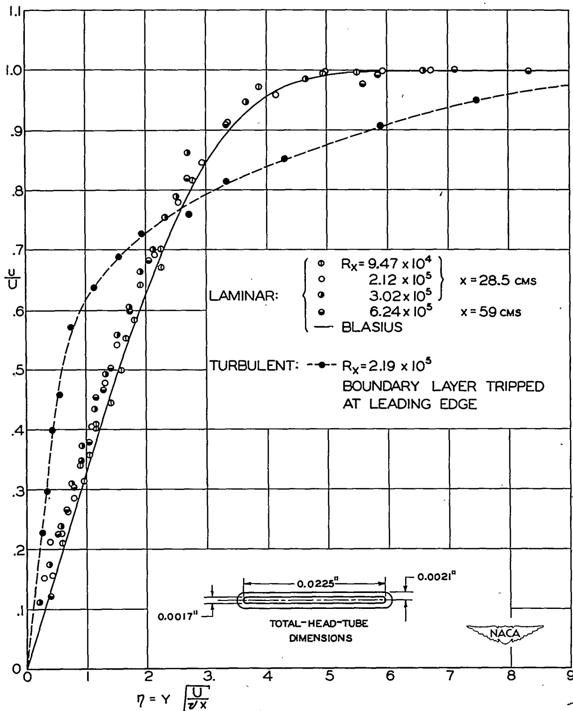
Figure 12.- Boundary-layer profiles on flat plate. Incompressible flow.
