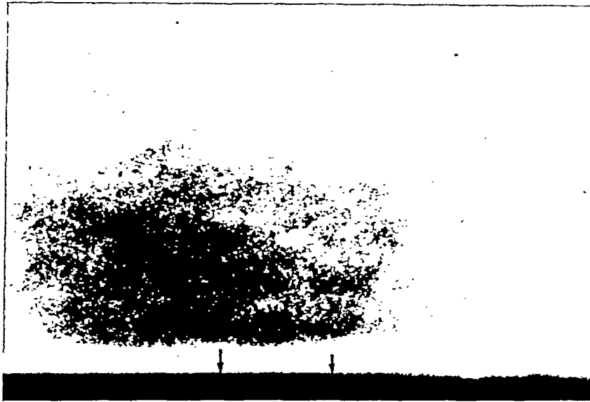
Figure 1.- Effect of slots in plate. Laminar boundary layer; M \approx 1.4 ; flow from left to right; arrows indicate position of slots.
