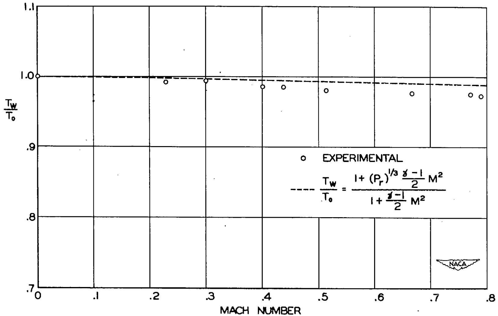
Figure 19.- Temperature recovery on flat plate with turbulent boundary layer. Zero heat transfer.
