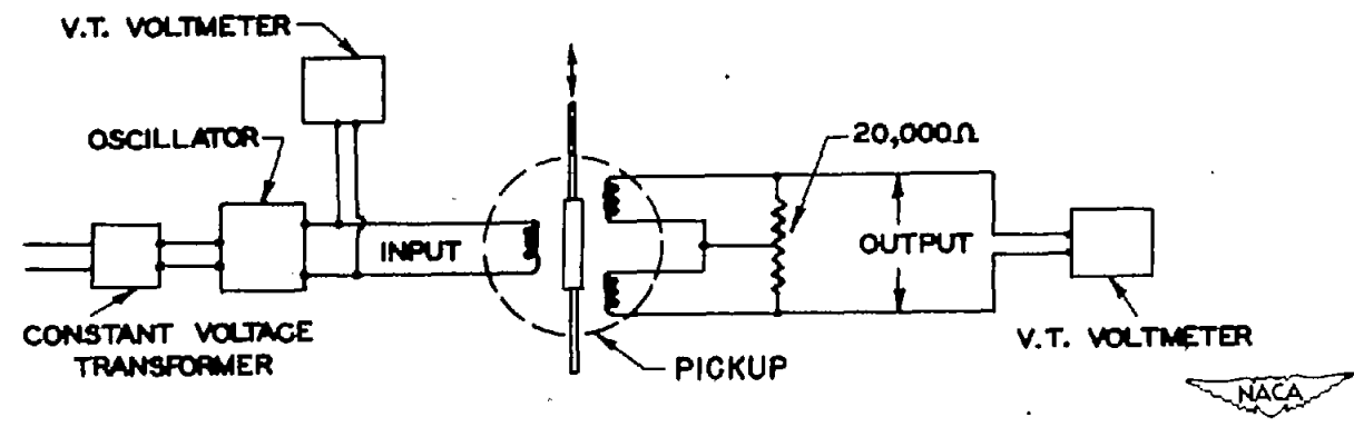
Figure 10.- Circuit used for skin-friction instrument.
