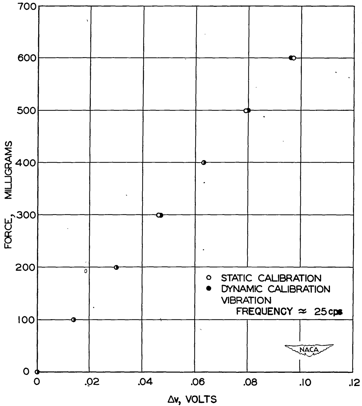
Figure 7.- Effect of vibrations on calibration of skin-friction instrument
