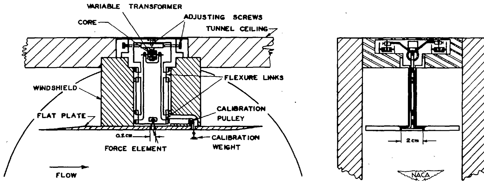
Figure 6.- Sketch of instrument for direct measurement of skin friction.
