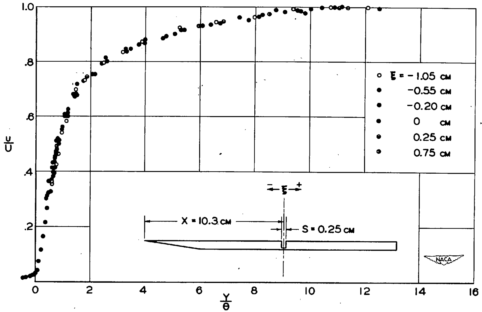
Figure 3.- Velocity profiles on flat plate with turbulent boundary layer and slot. R_x \approx 4 \times 10^4 ; R_s \approx 1000 .
