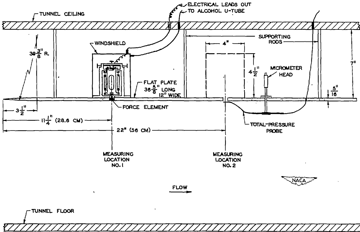
Figure 11.- Sketch of flat-plate installation in GALCIT 2 1/2 - by 2 1/2 - foot correlation tunnel.
