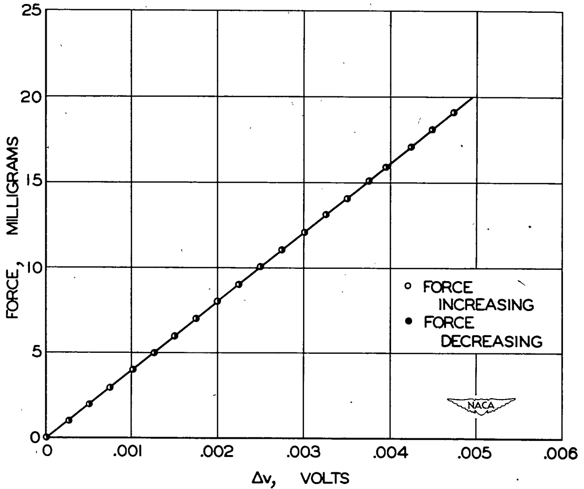
Figure 8.- Calibration of skin-friction instrument. Input, 5 volts at 20 kilocycles; 0.0005- by 1/4-inch links; \tau_o , 39.25 \times \Delta v dynes per square centimeter.
