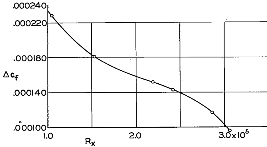
(a) Correction for pressure gradient; laminar boundary layer.
