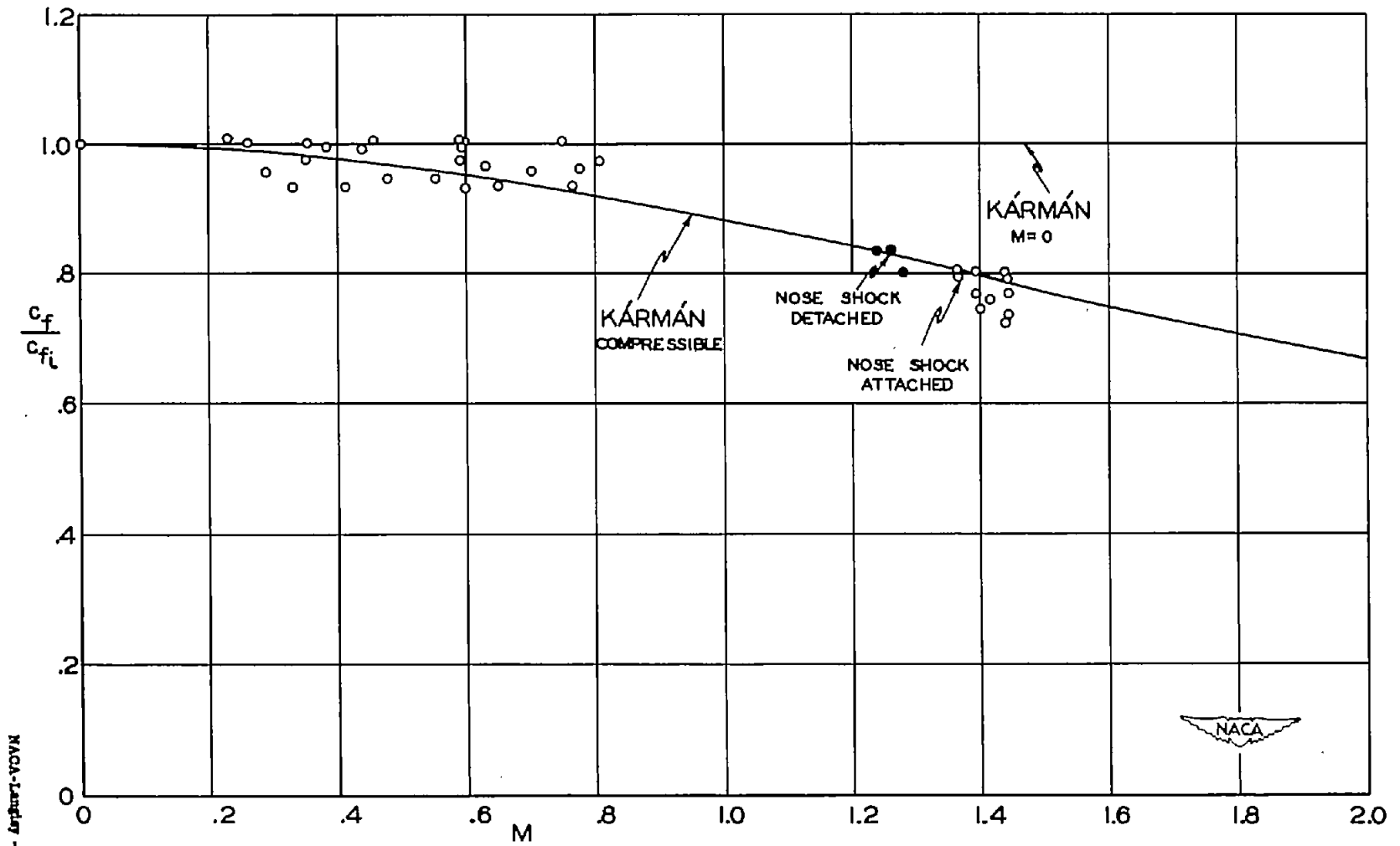
Figure 23.- Effect of compressibility on local skin friction on flat plate. Turbulent boundary layer; Reynolds number, R \approx 10^6 .
