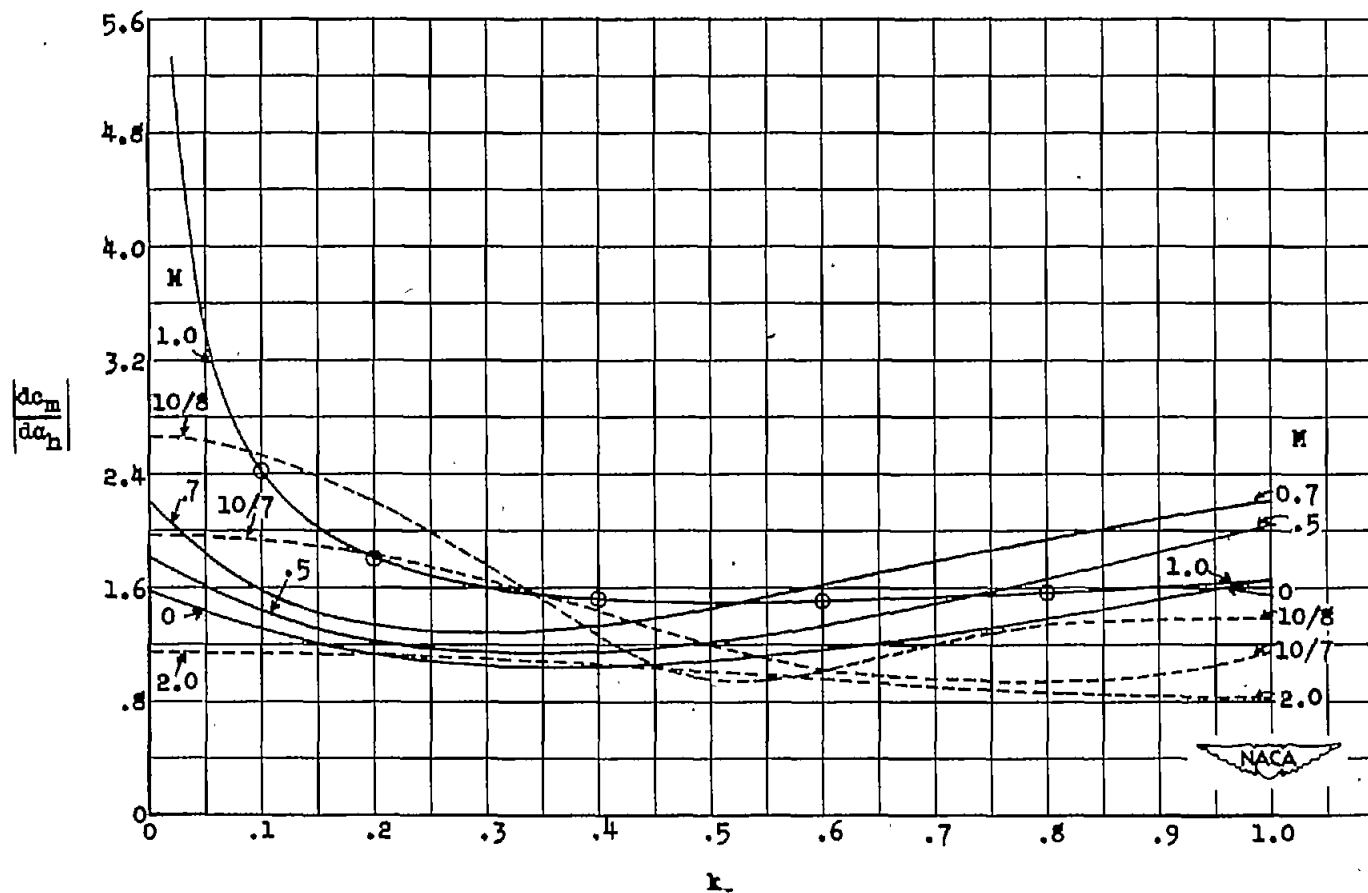
(c) Moment-curve slope associated with vertical translation.
