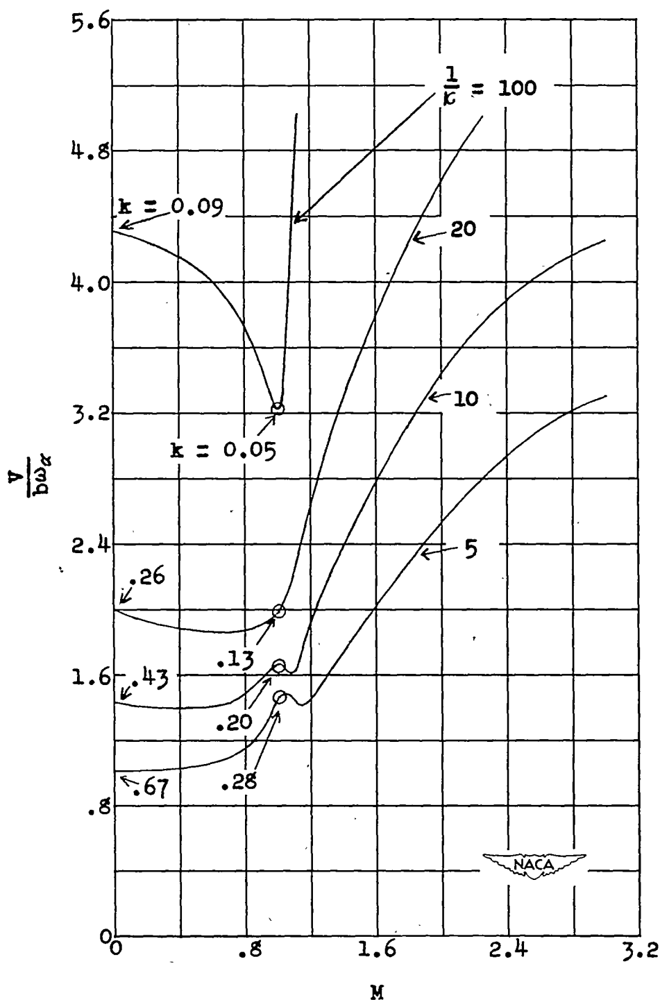
Figure 5.- Flutter-speed coefficient against Mach number for several values of 1/\kappa when \frac{\omega_h}{\omega_\alpha} = 0 , x_\alpha = 0.2 , and a = 0 . (Figure 18 of reference 5 modified to include calculated values indicated by circles.)
