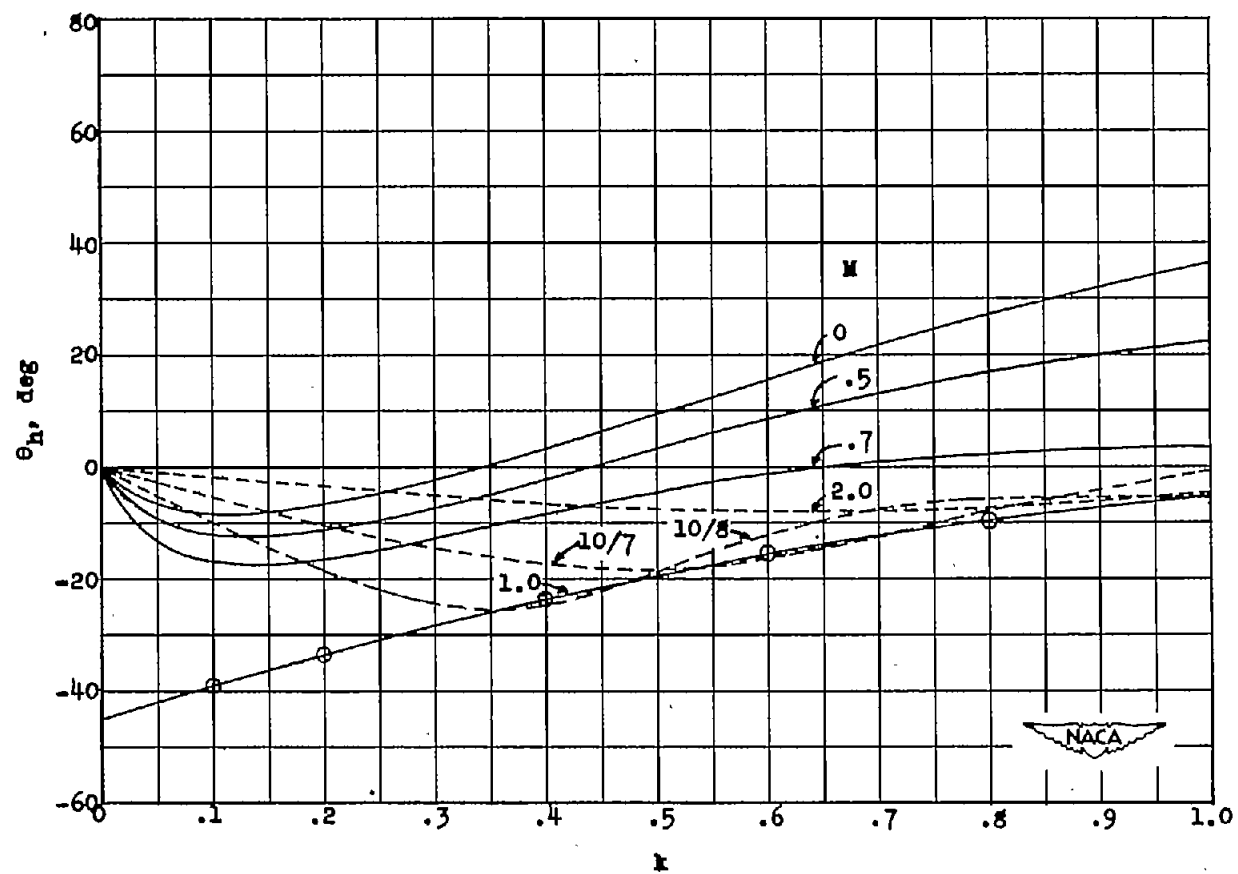
(a) Phase angle between lift vector due to vertical translation and vertical velocity vector \dot{h} .
