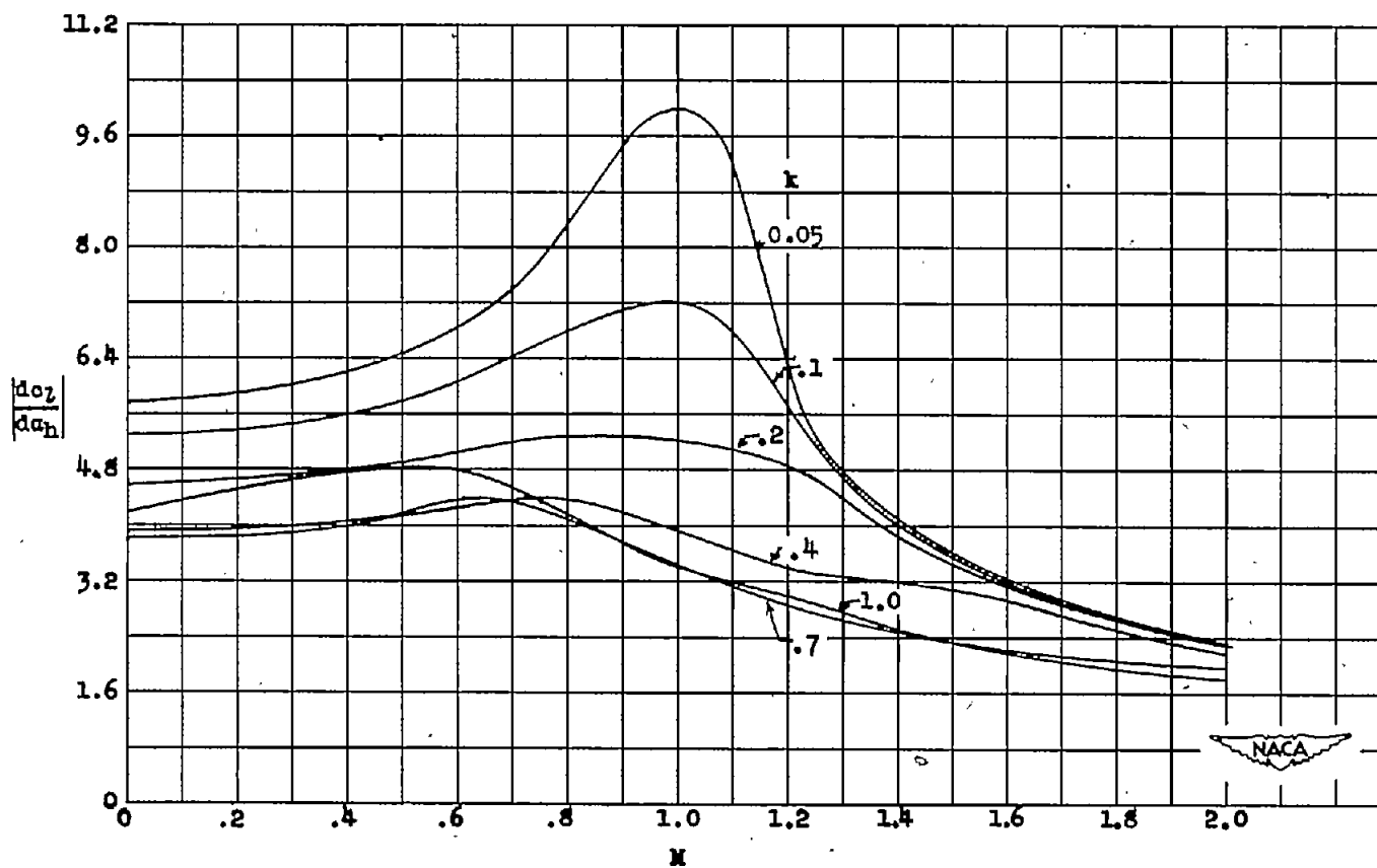
Figure 4.- Magnitude of lift-curve slope associated with vertical translation of wing against Mach number for several values of reduced frequency. \left| \frac{dc_l}{d\alpha_h} \right| = 4k \sqrt{L_1'^2 + L_2'^2} .
