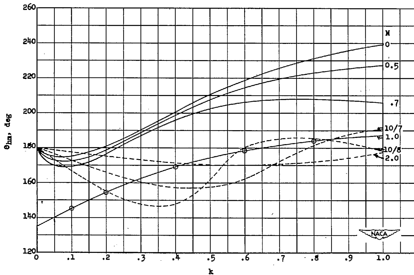
(c) Phase angle between moment vector due to vertical translation and vertical velocity vector \dot{h} .
