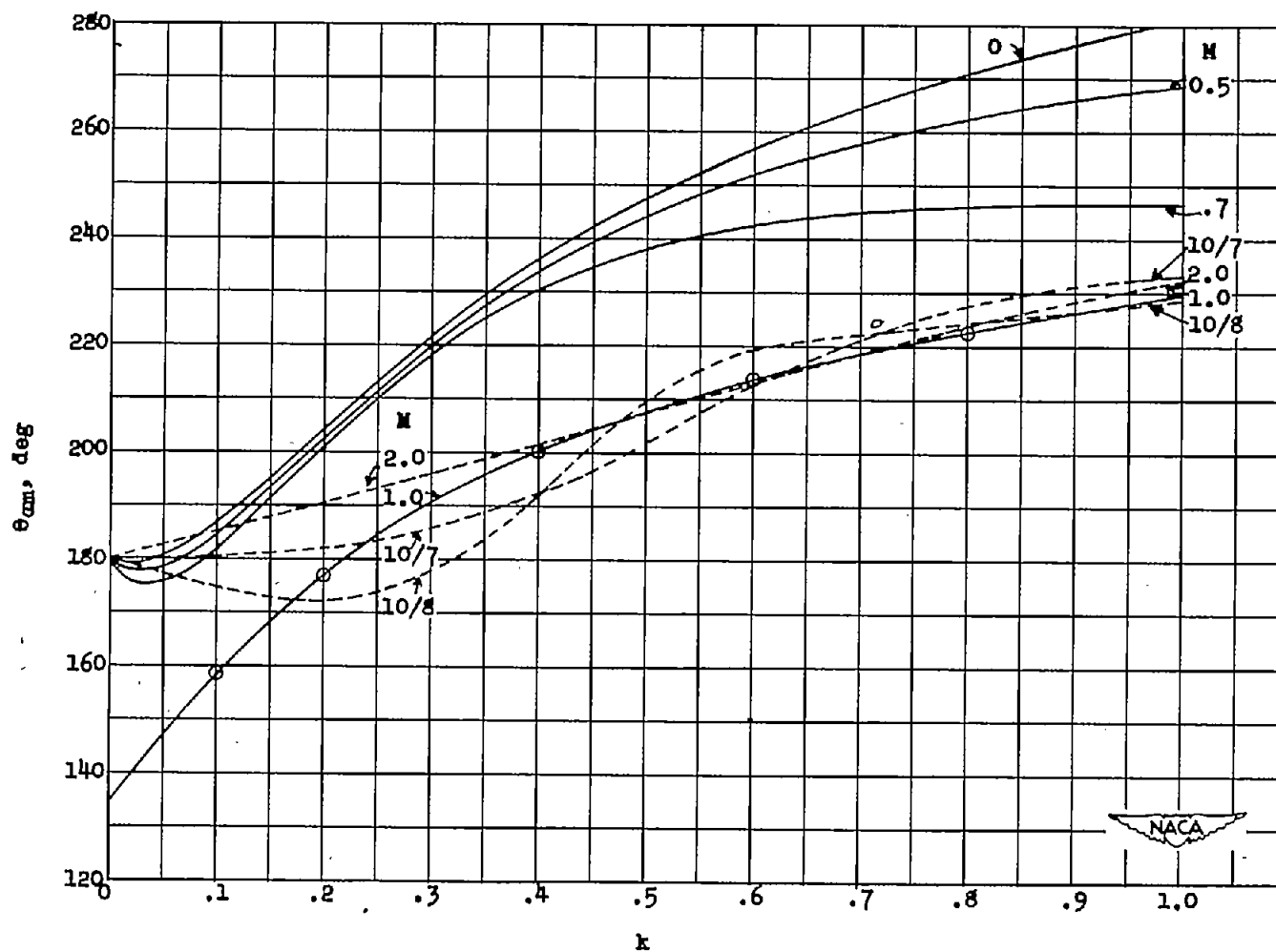
(d) Phase angle between moment vector due to pitching and angular displacement vector \alpha .
