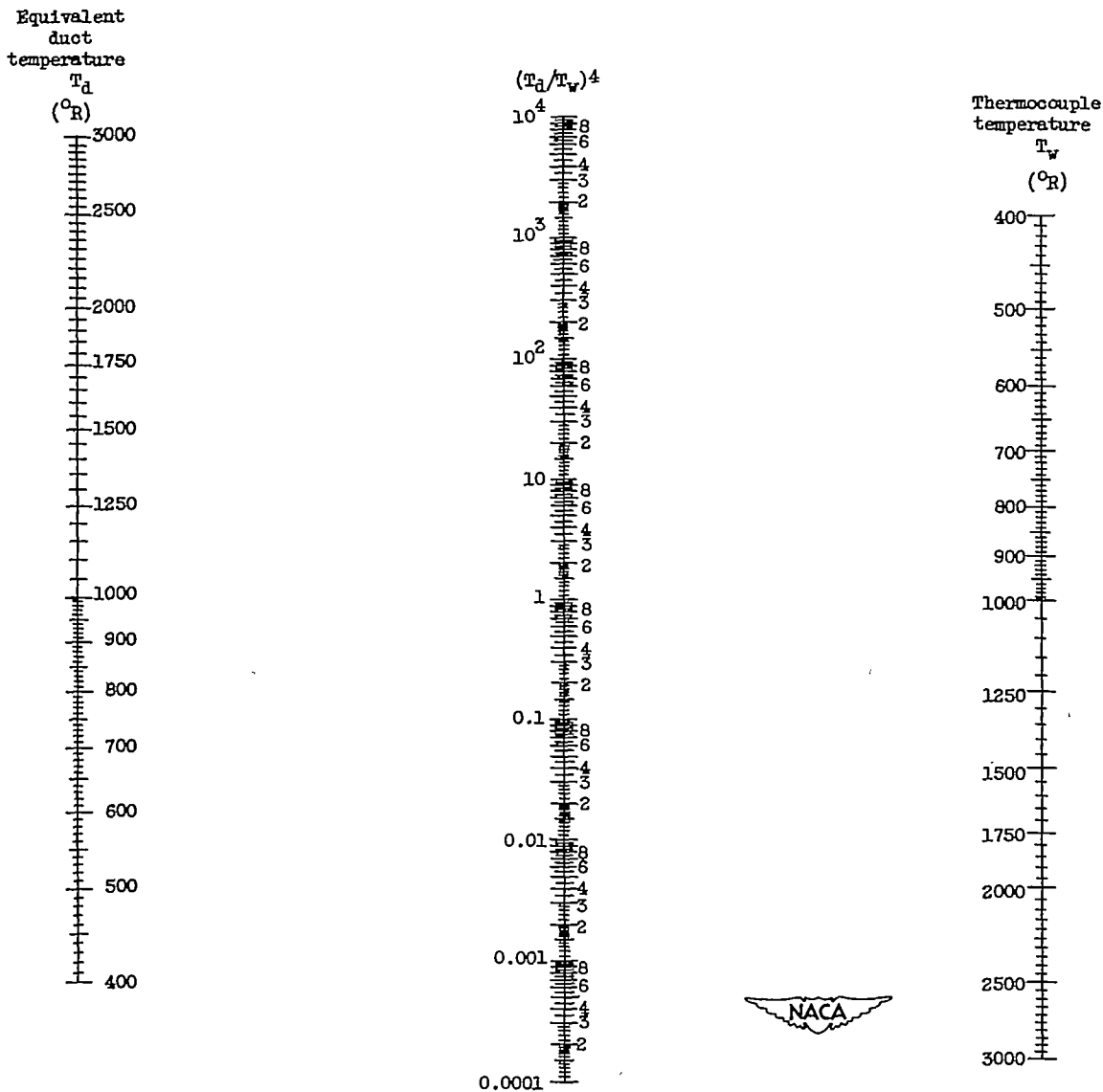
(b) Nomograph for computing (T_d/T_w)^4 .
