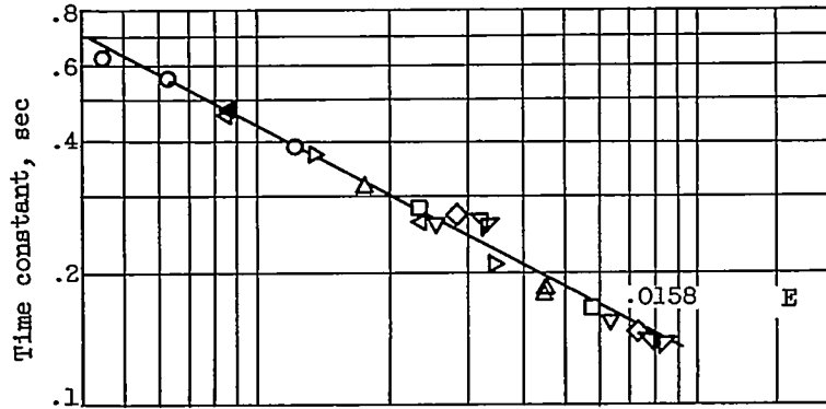
(c) Chromel-alumel.
