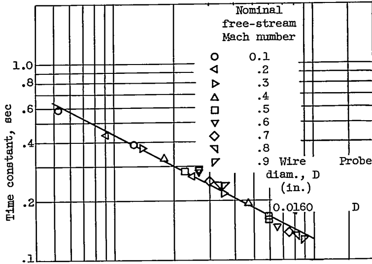
(b) Iron-constantan.
