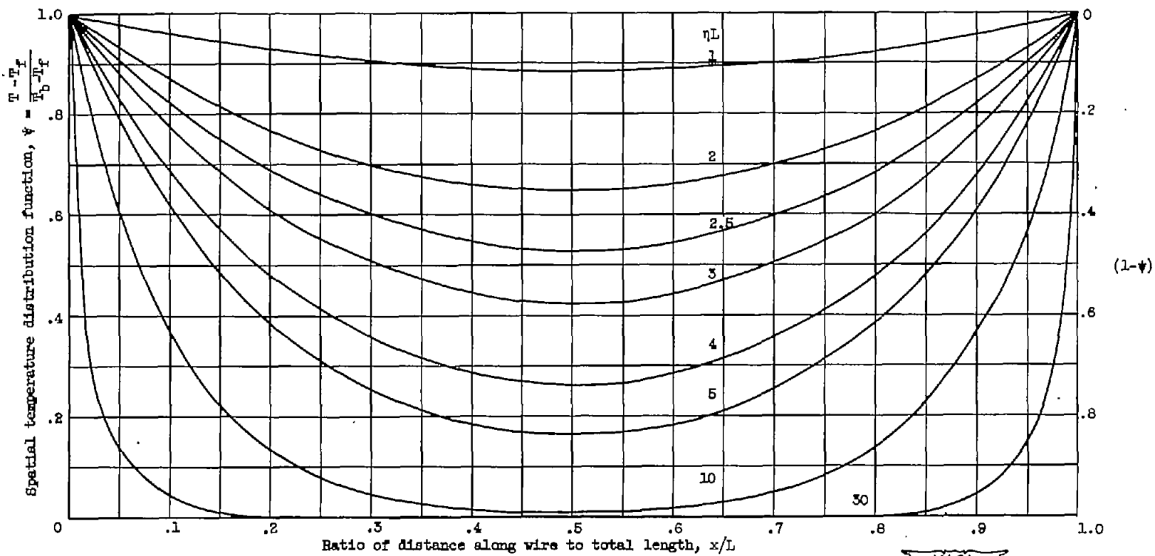
Figure 4. - Temperature distribution along simple wire in steady state.
