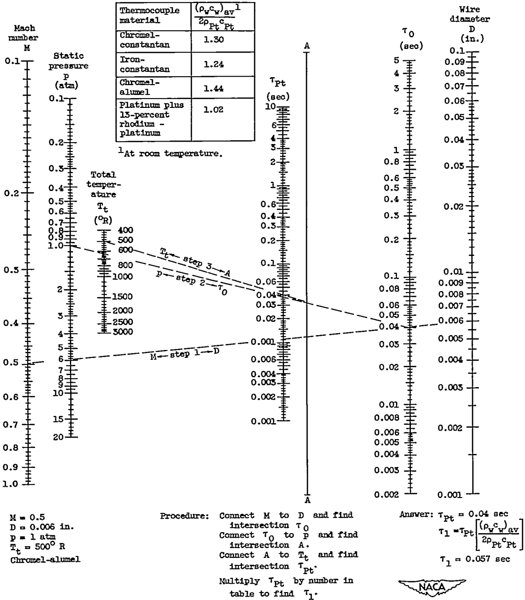
Figure 17. - Nomograph for computing T_1 . (A 11- by 12-in. print of this fig. is attached.)
