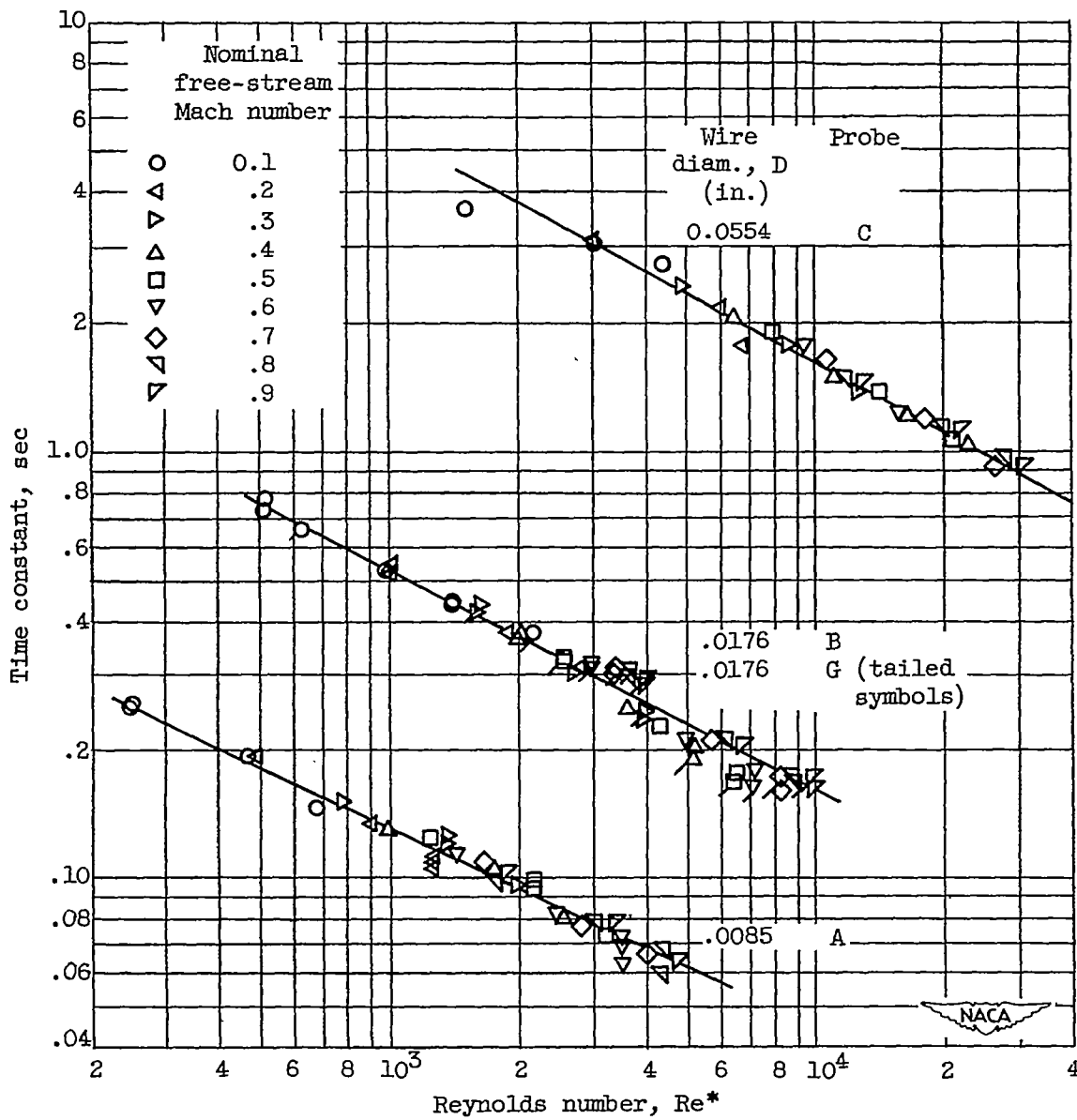
(a) Chromel-constantan.
