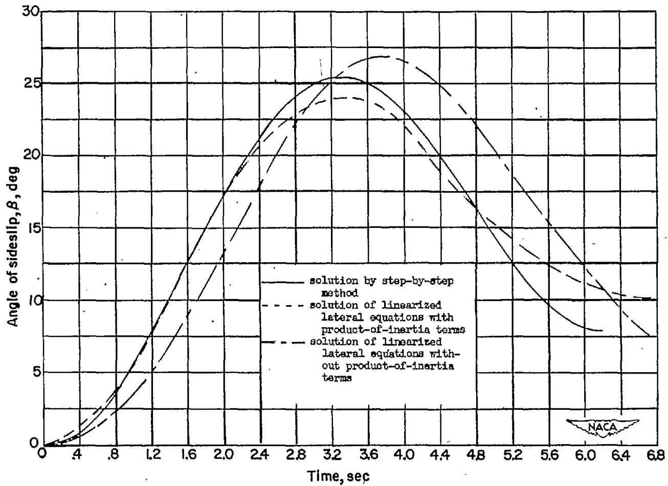
Figure 10.- Comparison of a solution by step-by-step method and a solution of linearized lateral equations of the variation of angle of sideslip with time for airplane B, loading 1, when rolled from trimmed flight at an angle of attack of 12^\circ .
