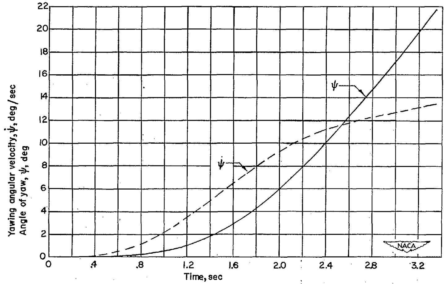
(c) \psi and \dot{\psi} .
