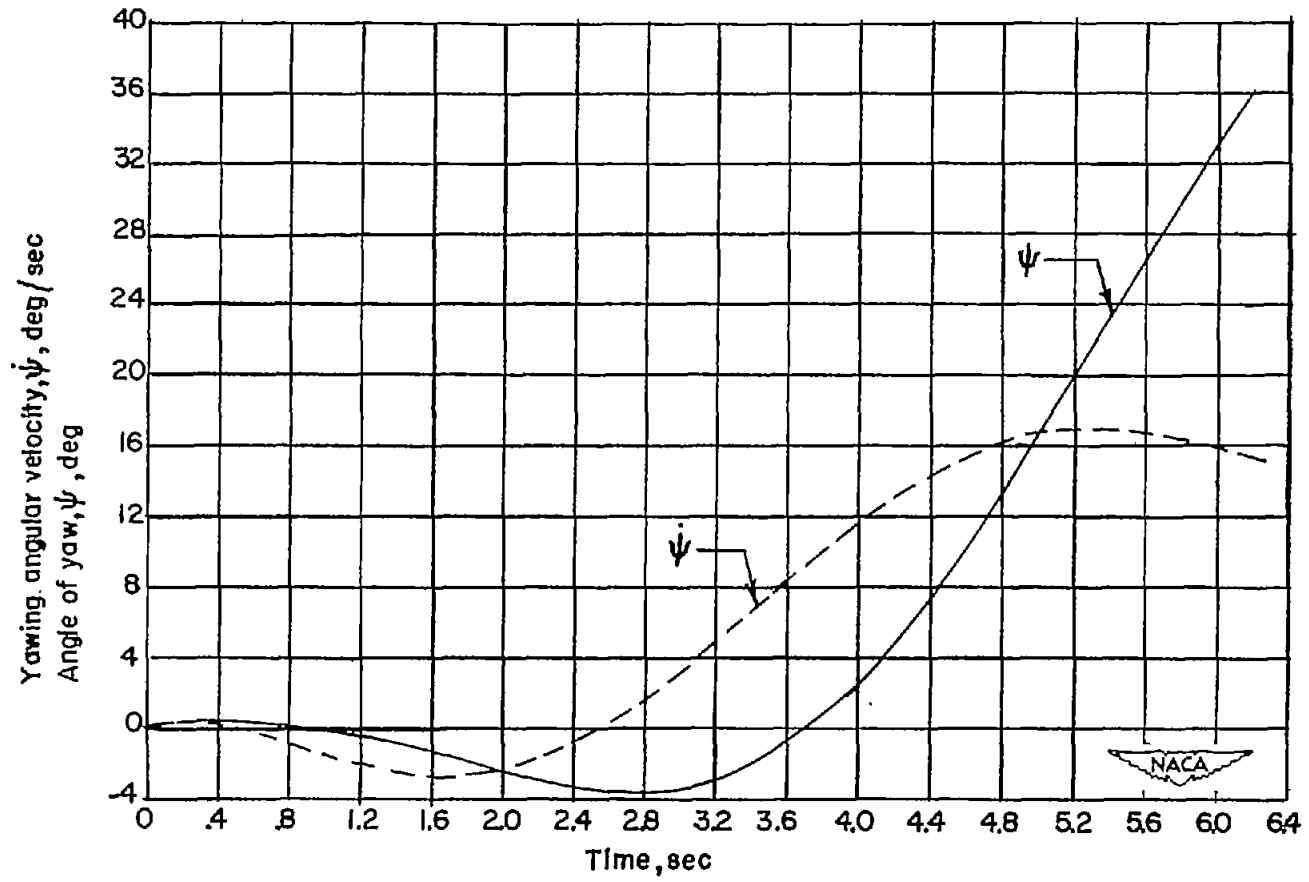
(c) \dot{\psi} and \psi .
