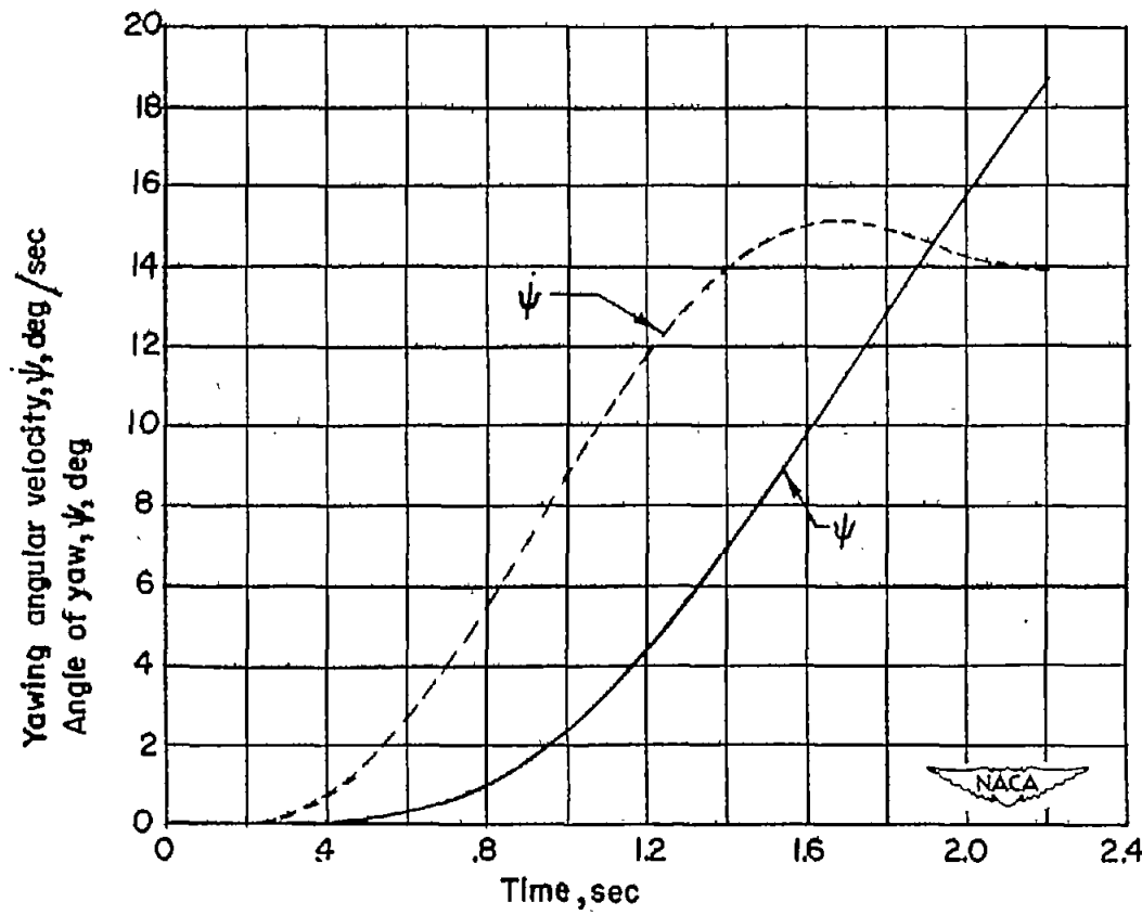
(c) \dot{\psi} and \psi .
