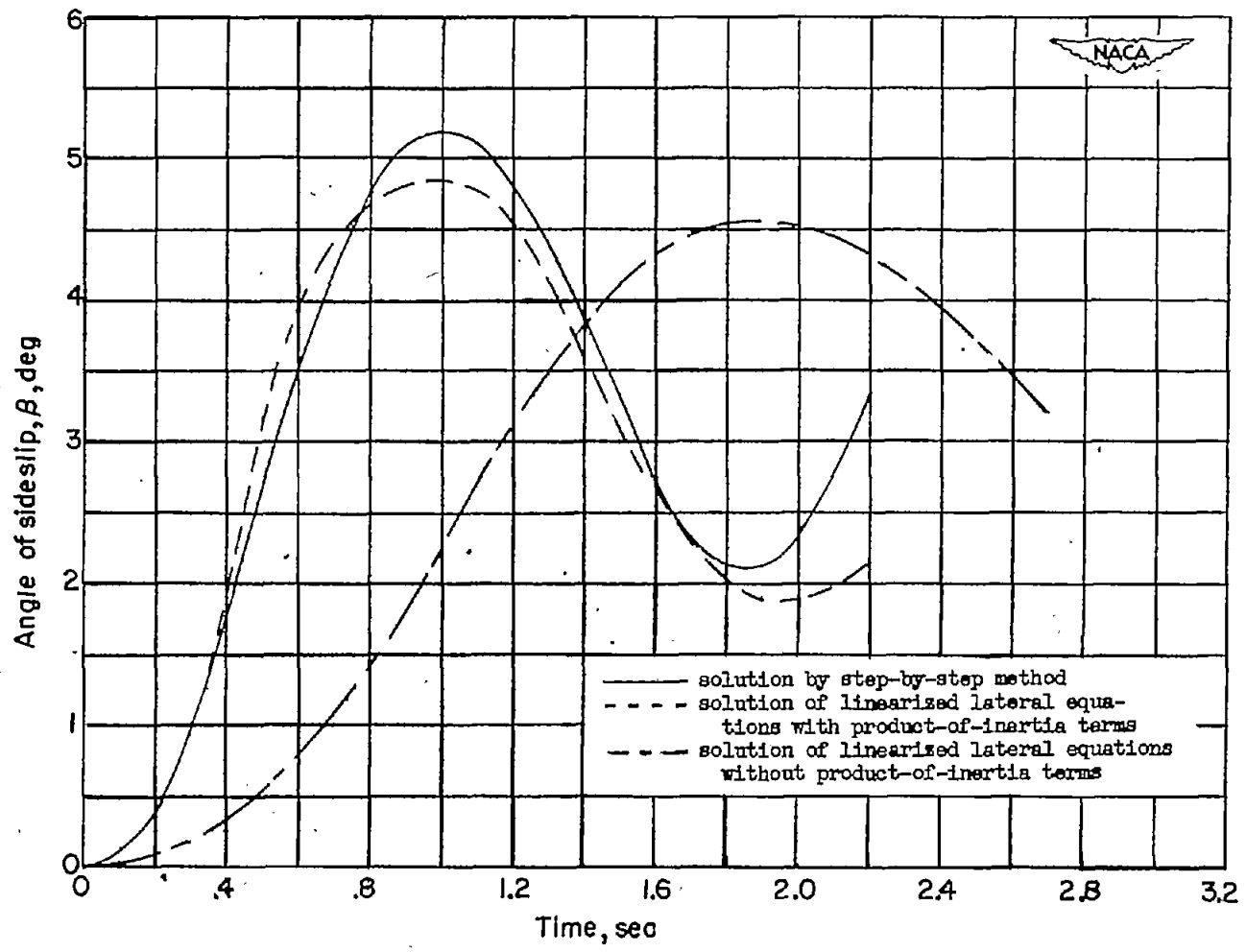
Figure 7.- Comparison of a solution by step-by-step method and a solution of linearized lateral equations of the variation of angle of sideslip with time for airplane A, loading 1, when rolled from trimmed flight at an angle of attack of 10^\circ .
