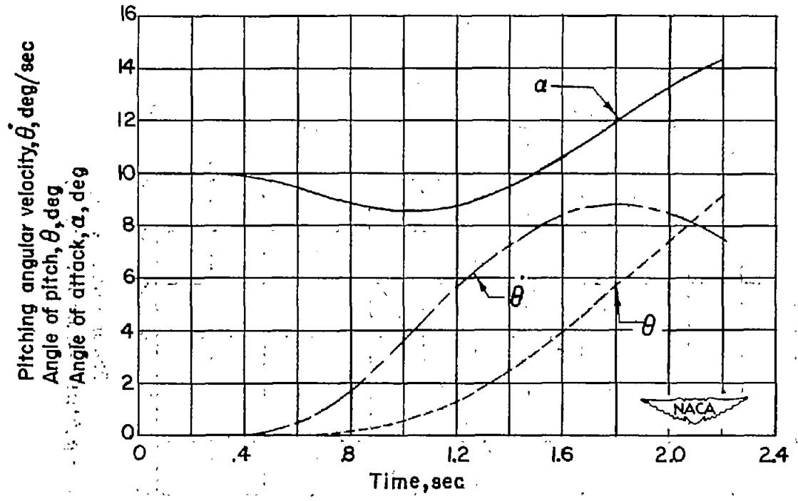
(b) \alpha , \theta , and \dot{\theta} .
