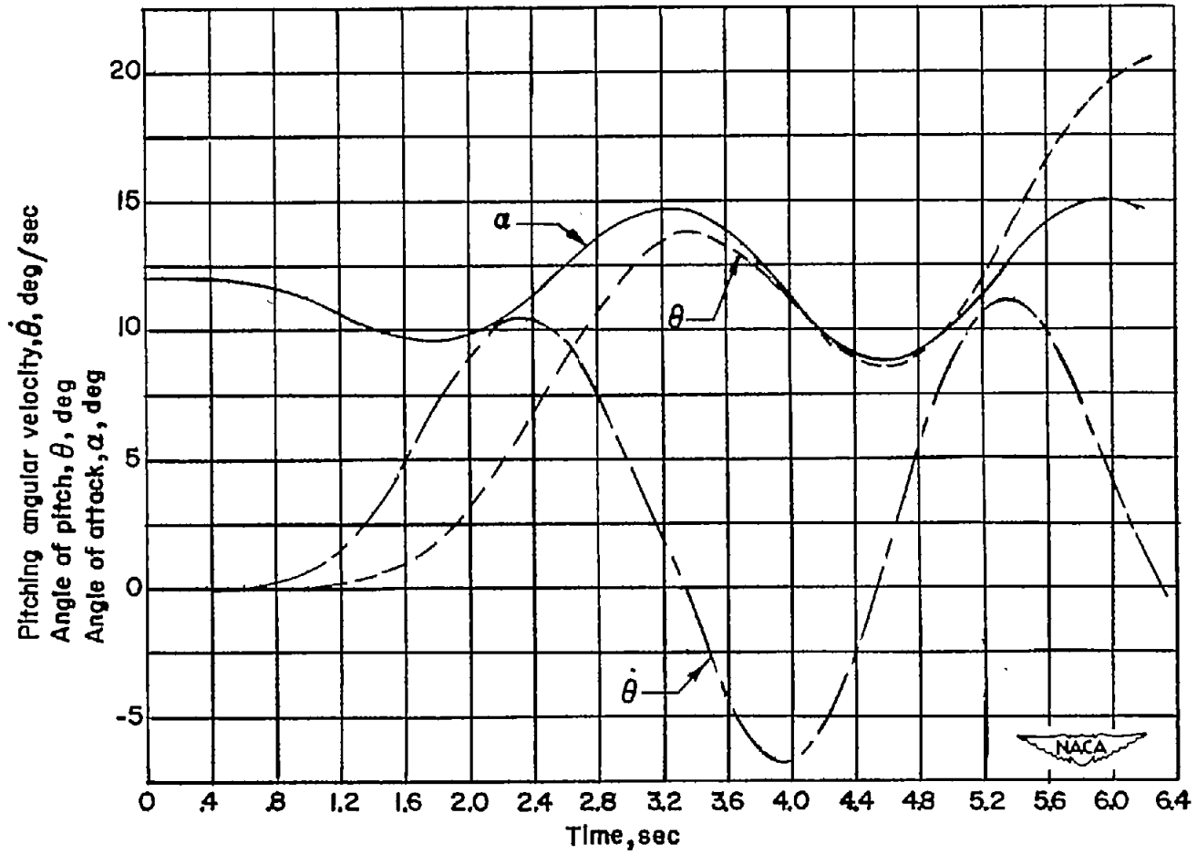
(b) \alpha , \theta , and \dot{\theta} .
