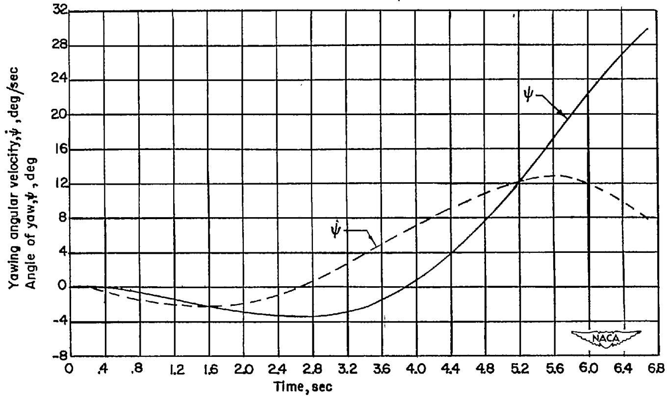
(c) \psi and \dot{\psi} .
