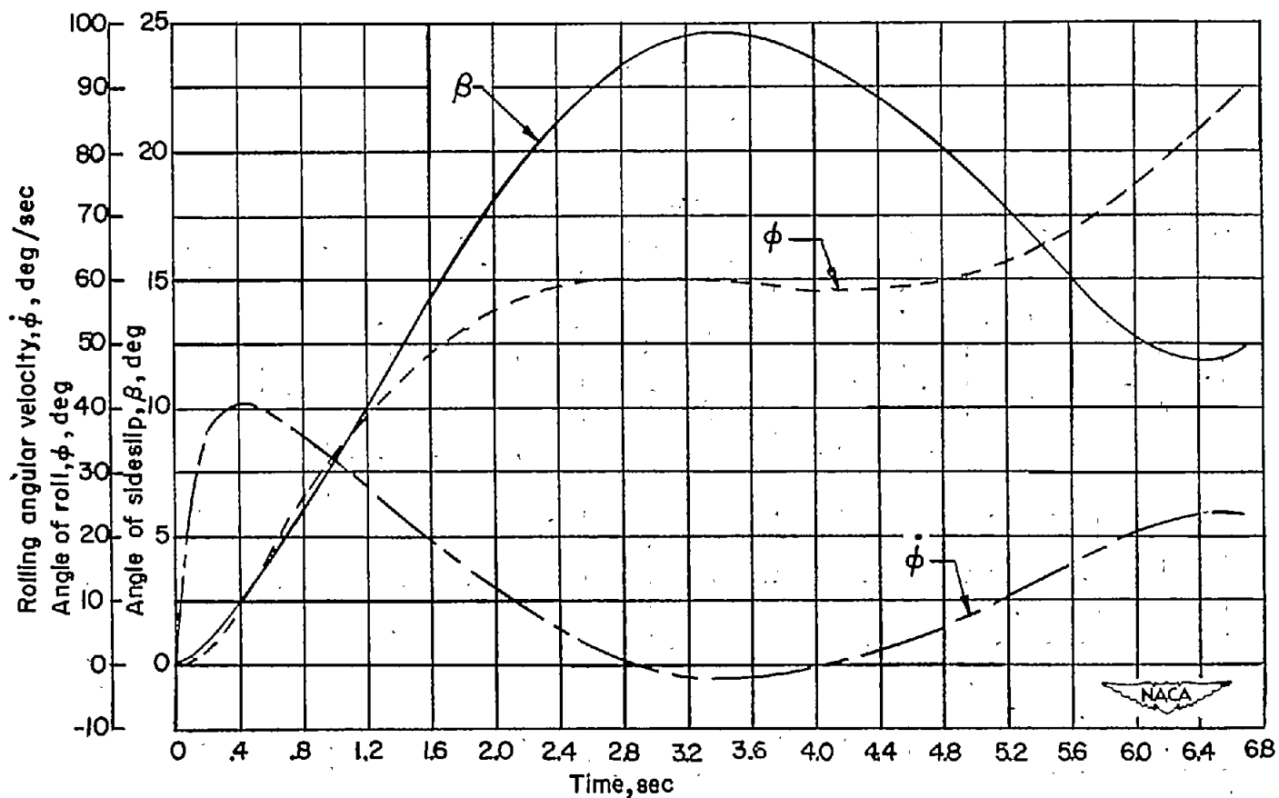
(a) \beta , \phi , and \dot{\phi} .
