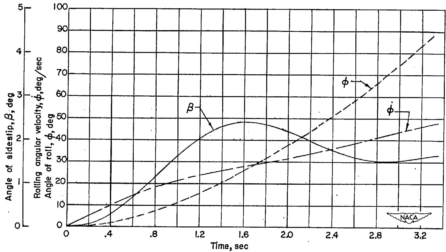
(a) \beta , \phi , and \dot{\phi} .
