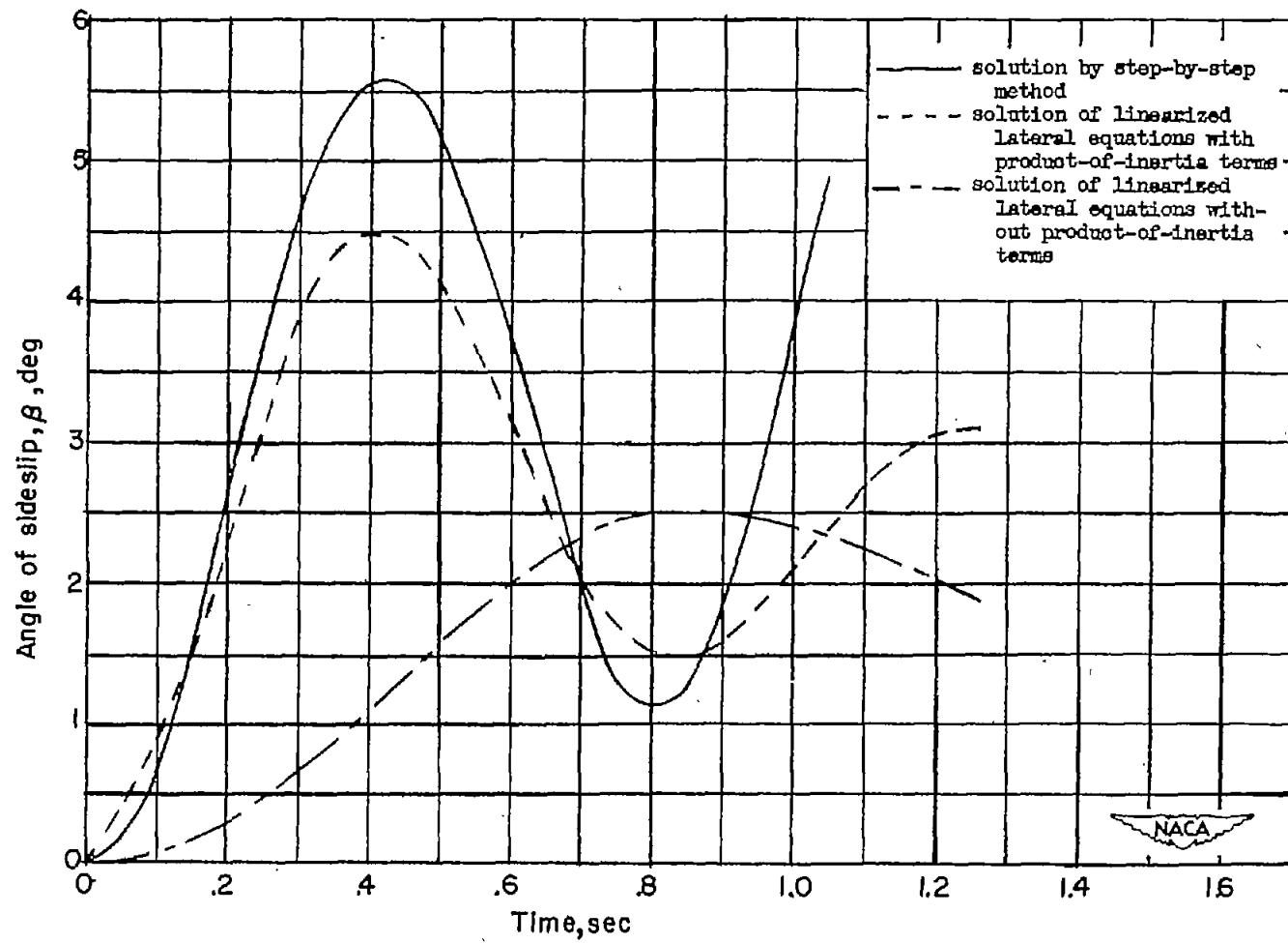
Figure 9.- Comparison of a solution by step-by-step method and a solution of linearized lateral equations of the variation of angle of sideslip with time for airplane A, loading 1, when rolled in a 6g pull-out.
