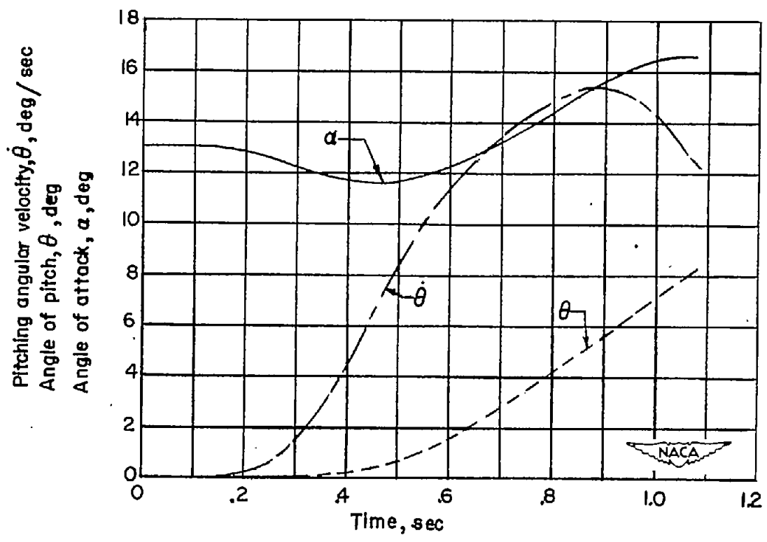
(b) \alpha , \theta , and \dot{\theta} , where \dot{\theta} is an increment added to the initial pitching velocity.
