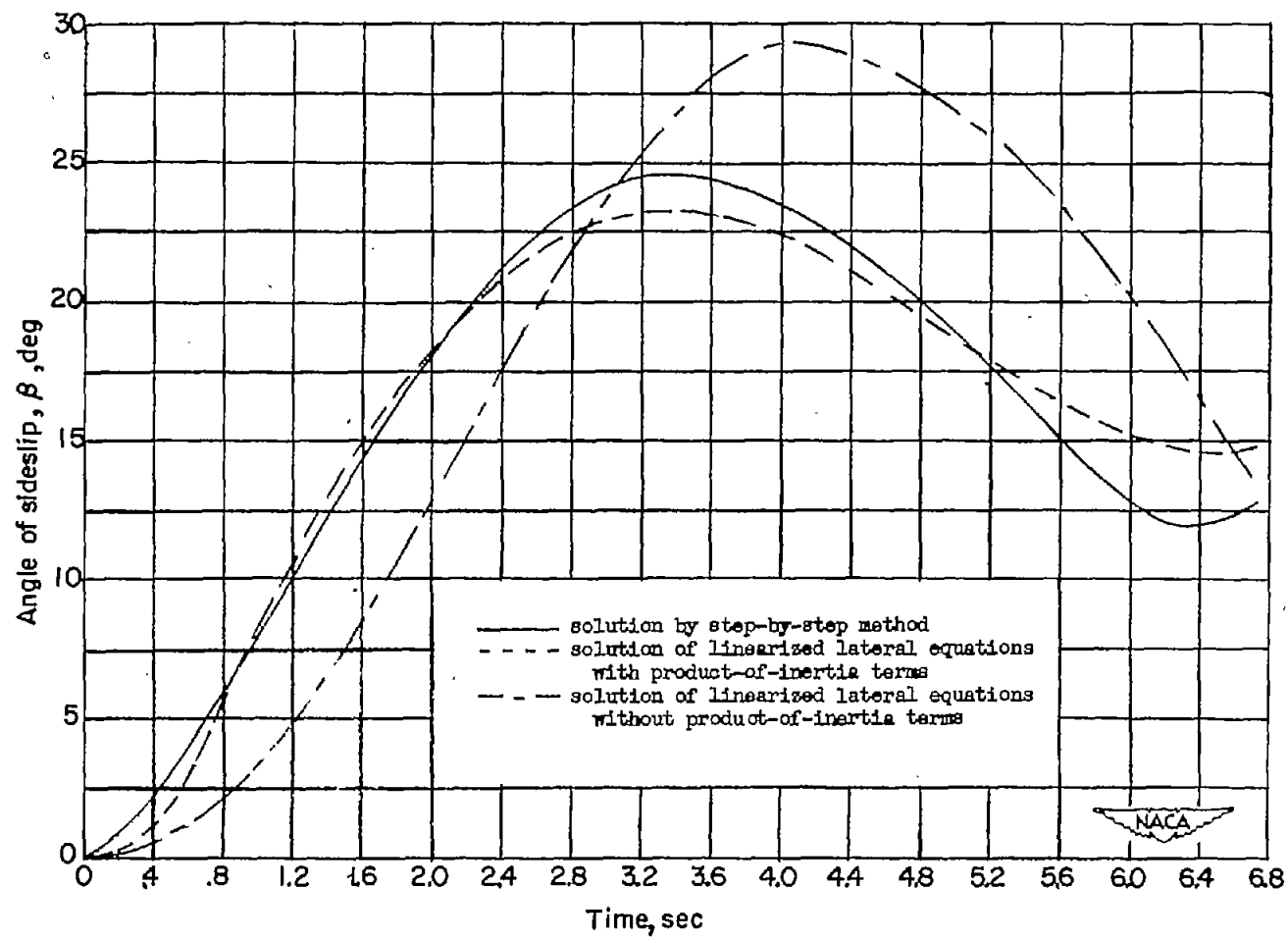
Figure 11.- Comparison of a solution by step-by-step method and a solution of linearized lateral equations of the variation of angle of sideslip with time for airplane B, loading 2, when rolled from trimmed flight at an angle of attack of 12^\circ .
