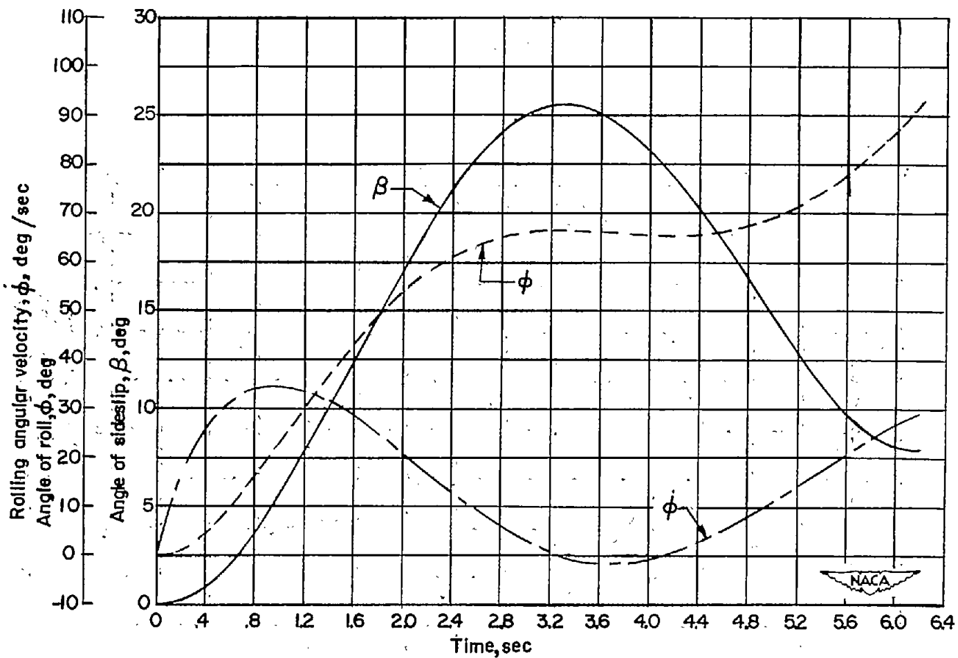
(a) \beta , \phi , and \dot{\phi} .
