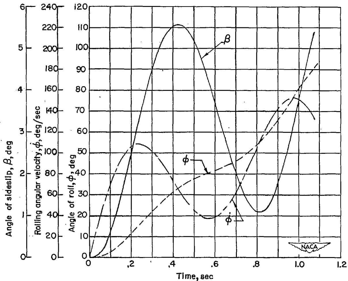
(a) \beta , \phi , and \dot{\phi} .
