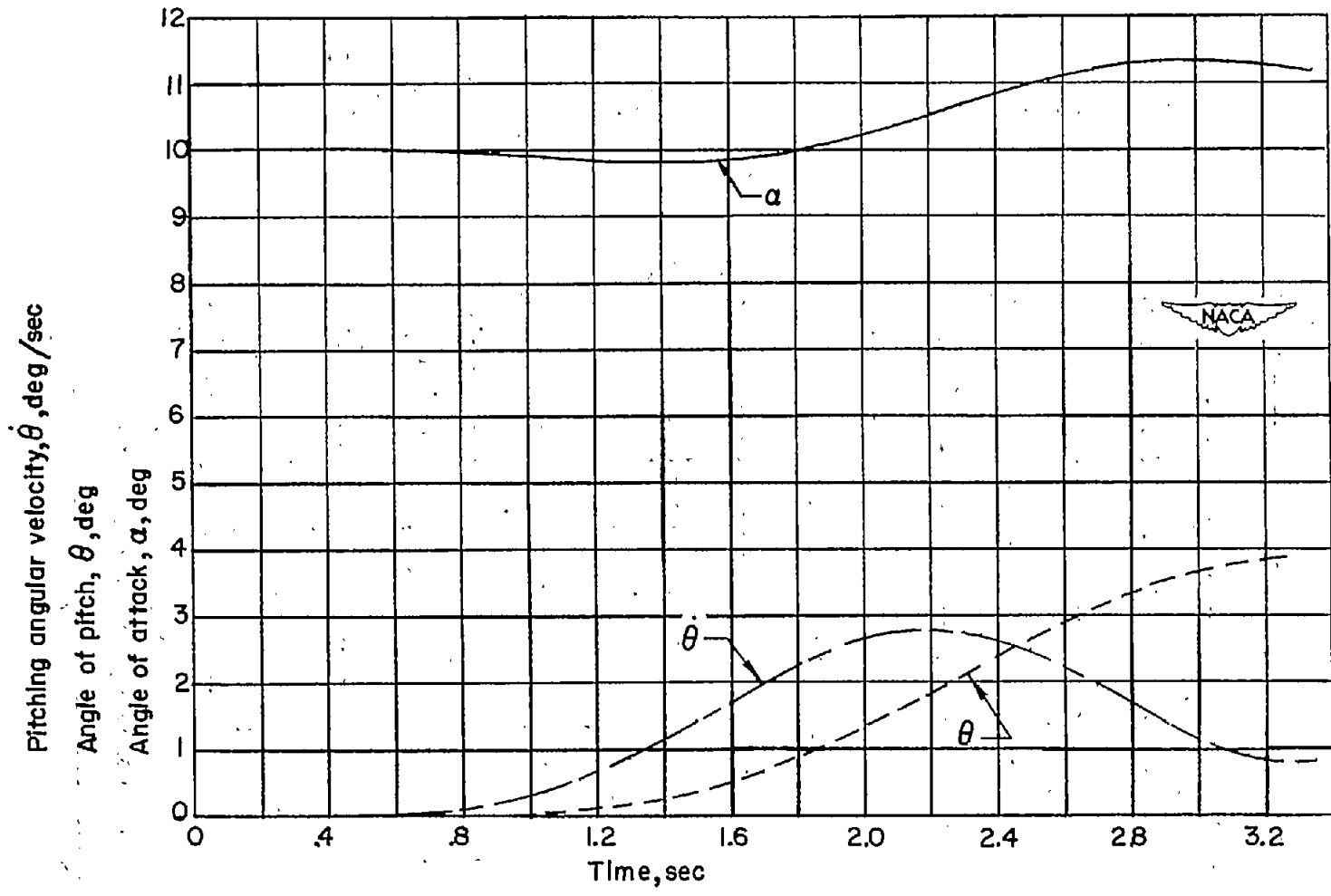
(b) \alpha , \theta , and \dot{\theta} . Figure 3.- Continued.
