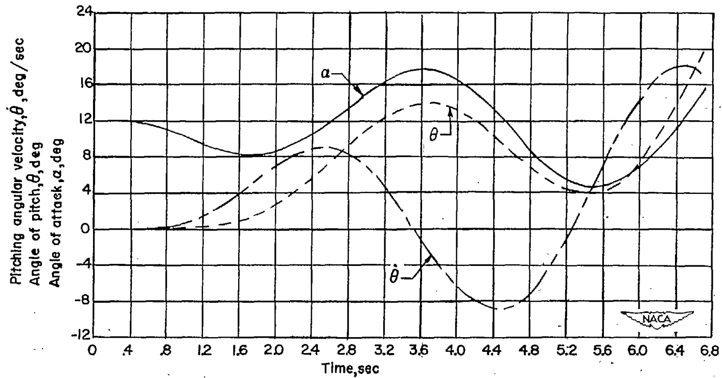
(b) \alpha , \theta , and \dot{\theta} .
