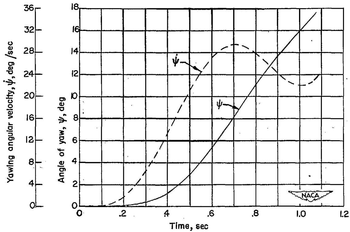
(c) \psi and \dot{\psi} .
