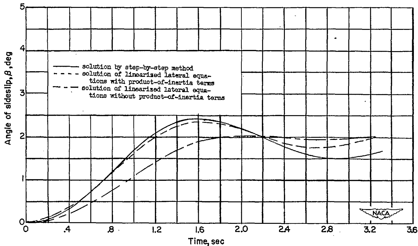
Figure 8.- Comparison of a solution by step-by-step method and a solution of linearized lateral equations of the variation of angle of sideslip with time for airplane A, loading 2, when rolled from trimmed flight at an angle of attack of 10^\circ .
