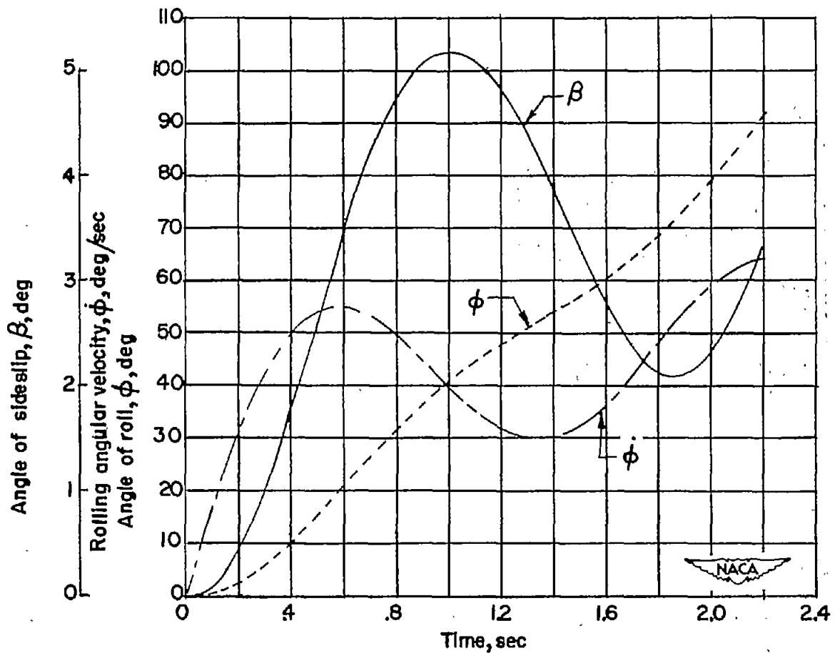
(a) \beta , \dot{\phi} , and \phi .
