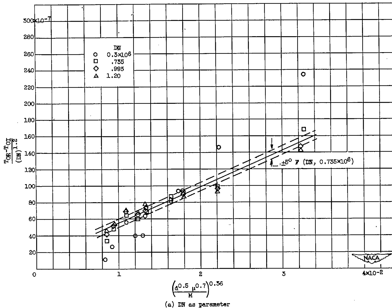
Figure 16. - Cooling-correlation curve for outer-race temperature of bearing 18. (Temperature T , °F; DN, bearing bore in mm times shaft speed in rpm; viscosity \mu , lb-sec/sq in.; oil-jet diameter, in.; oil flow M , lb/min.)
