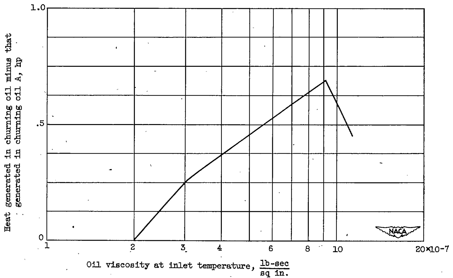
Figure 12. - Concluded. Effect of viscosity on heat generated in churning oil. Load, 368 pounds; DN, 1.2×10 6 .
