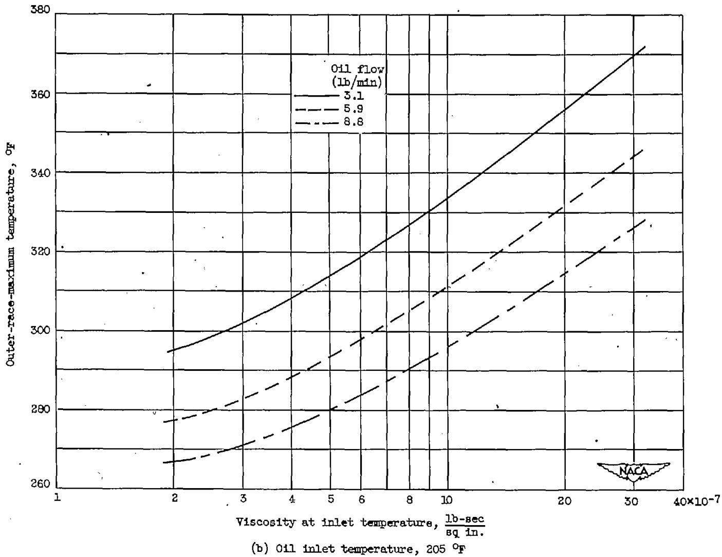
Figure 10. - Concluded. Effect of oil viscosity on outer-race-maximum temperature of bearing 18 (cross-plot of figs. 2 and 6(b)). Load, 368 pounds; DM, 1.2 \times 10^6 .
