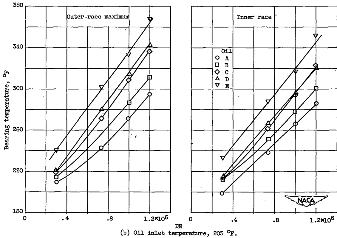
Figure 3. - Concluded. Effect of DN on outer-race-maximum and inner-race temperatures of bearing 18. Load, 368 pounds; oil flow, 2.75 pounds per minute.
