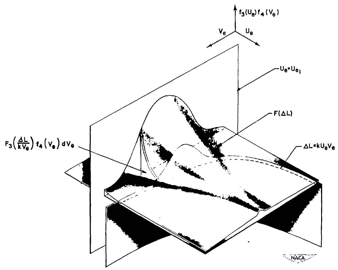
Figure 2.- Pictorial representation of volume integral equation (12),
