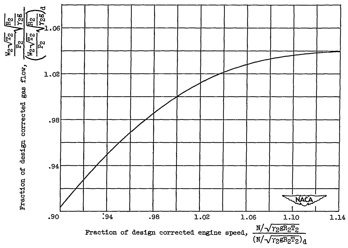
Figure 1. - Variation of compressor-inlet corrected gas flow with corrected engine speed.
