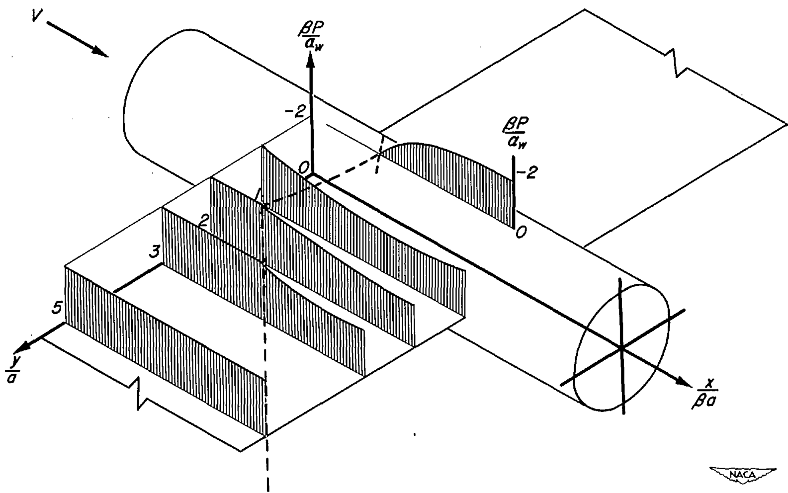
Figure 19.- Isometric drawing of pressure distribution acting on combination of body and rectangular wing.
