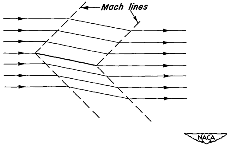
Figure 8.—Flow field produced by wing alone.
