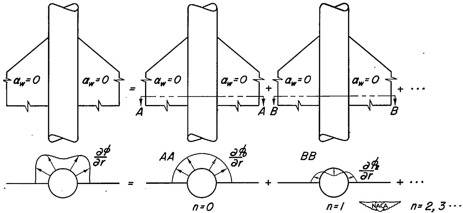
Figure 4.- Decomposition of interference combination into series of Fourier component interference combinations.
