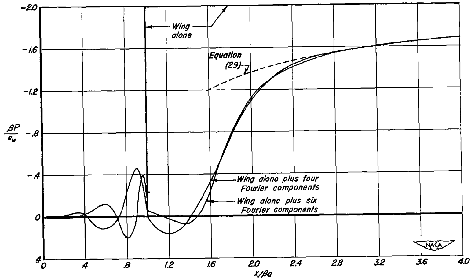
Figure 17. - Pressure distribution on top of combination of body and rectangular wing using four and six Fourier components.
