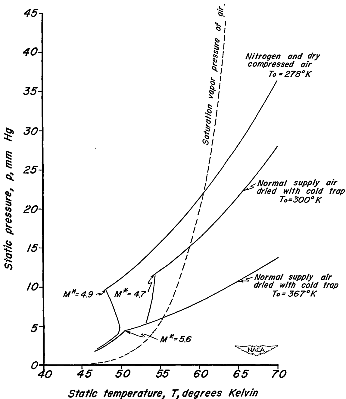
(b) Purified gases expanded from various reservoir temperatures in the 1-by 1.4-inch supersonic nozzle.
