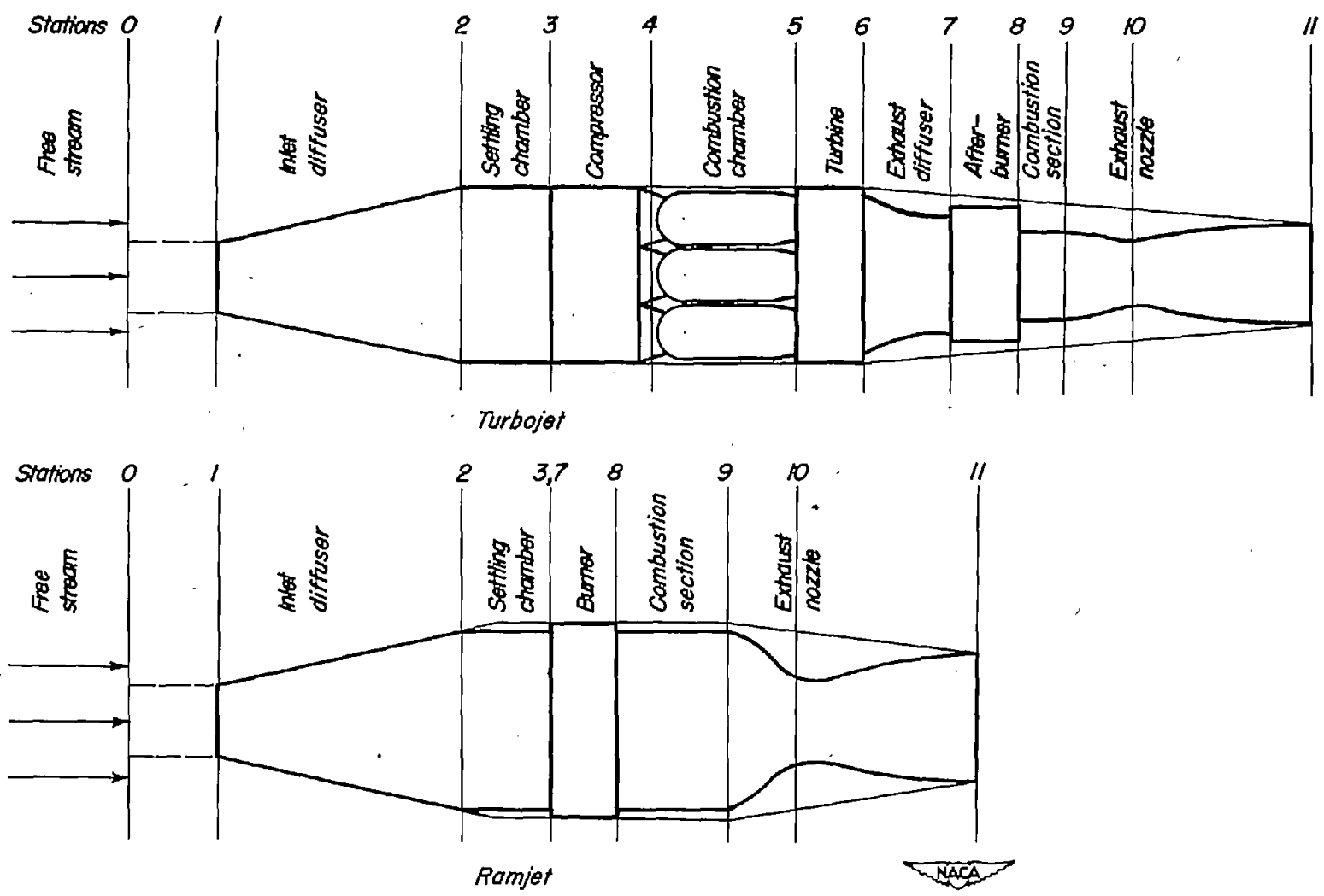
Figure 1.- Schematic representation of propulsive systems.
