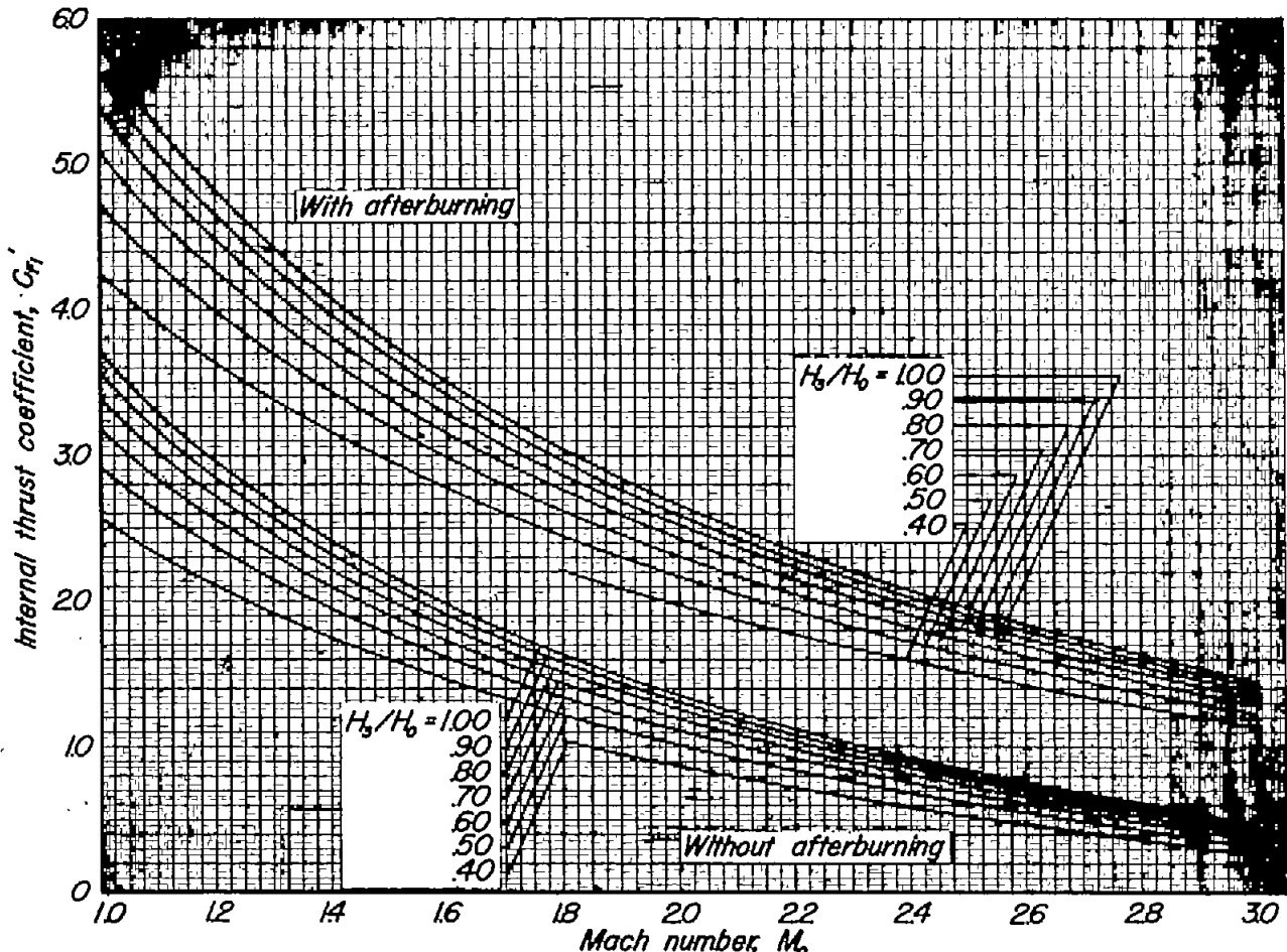
Figure 8- Effects of total-pressure recovery on internal thrust coefficient of turbojet of figure 7 operating at 2000° Rankine without afterburning and the same turbojet with afterburning having a total air-to-fuel ratio equal to that of the ram jet of figure 6.
