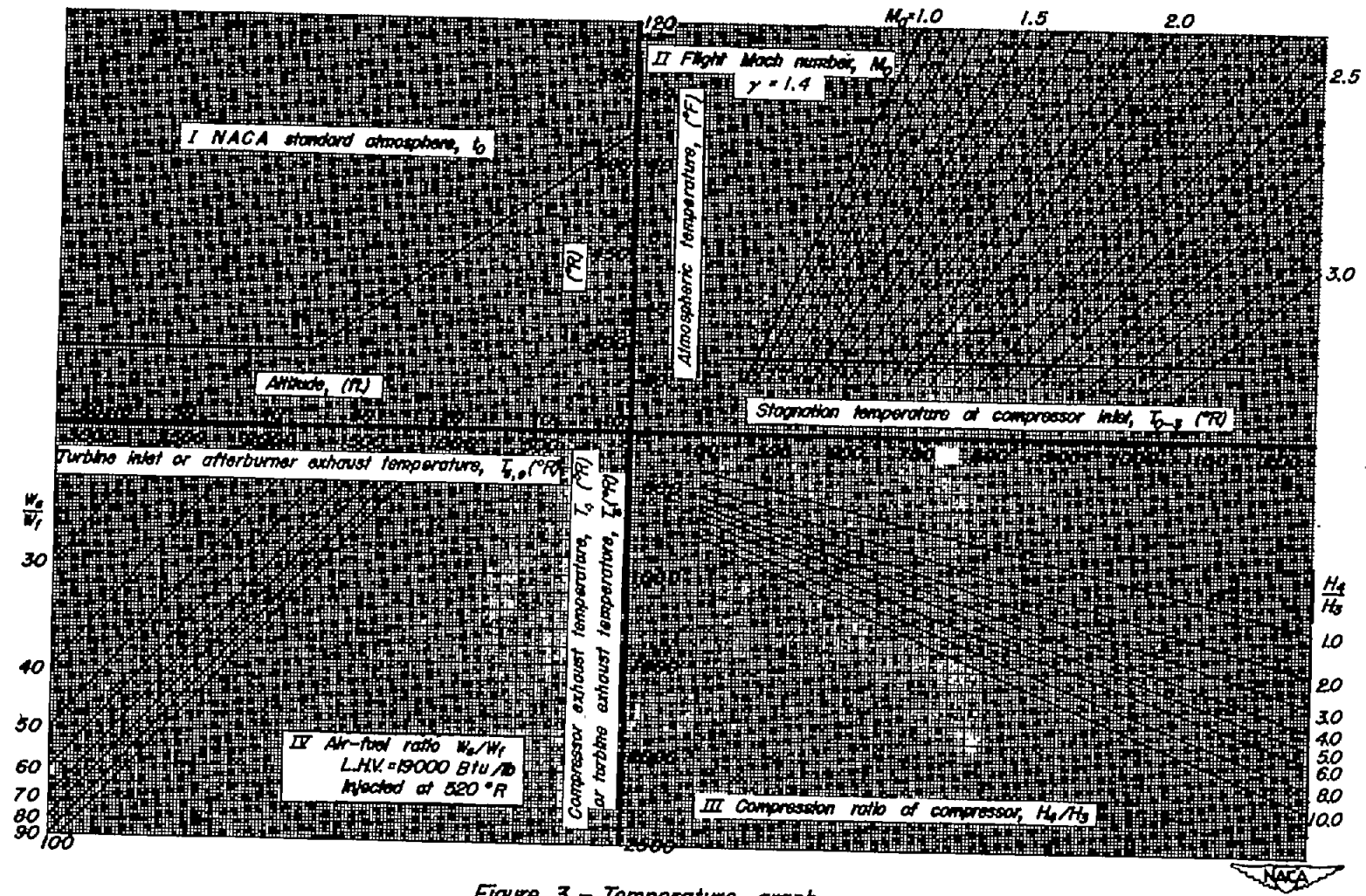
Figure 3. - Temperature graph.
