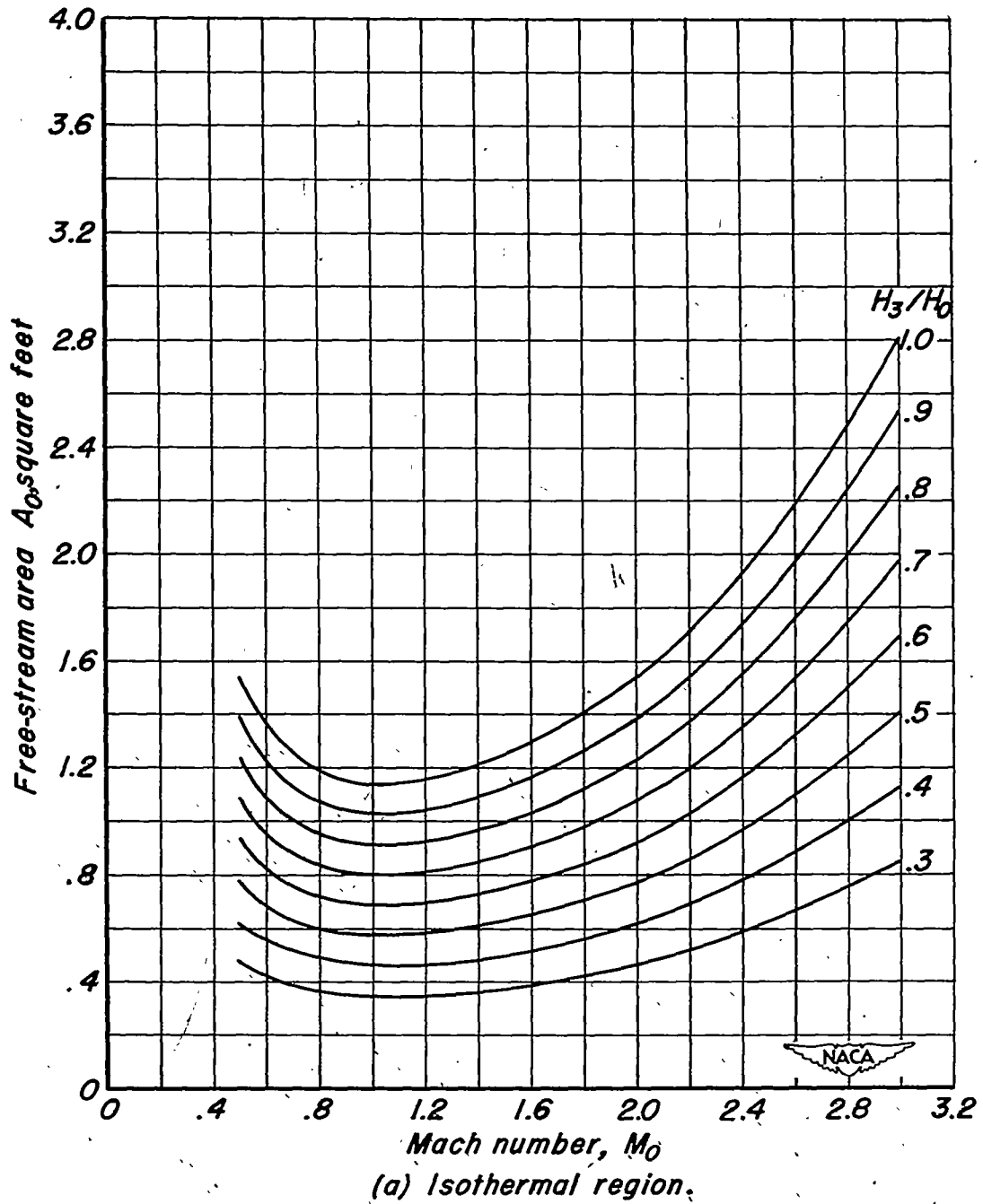
Figure 14.- Free-stream area required by the turbojet engine of the illustrative examples.
