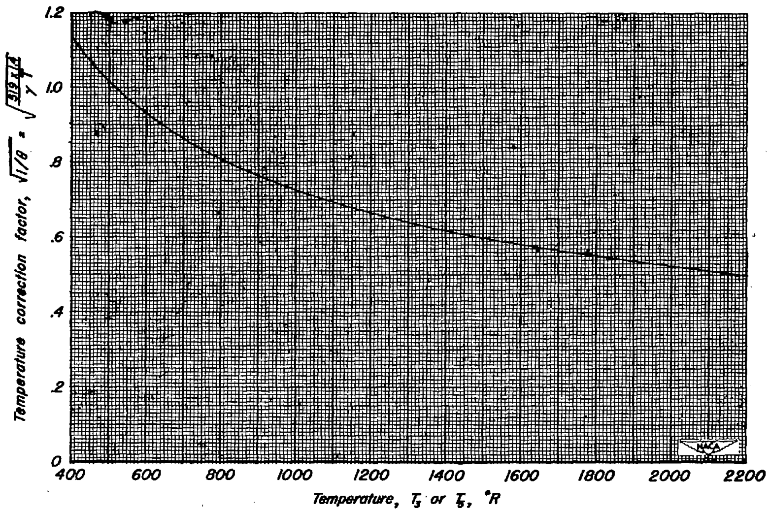
Figure 5.— Temperature correction graph.
