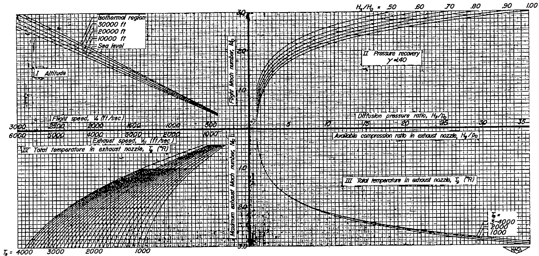
Figure 2.- Velocity graph.
