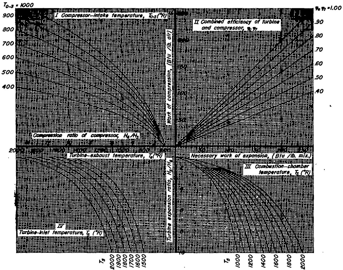
Figure 4.- Compressor - turbine graph.
