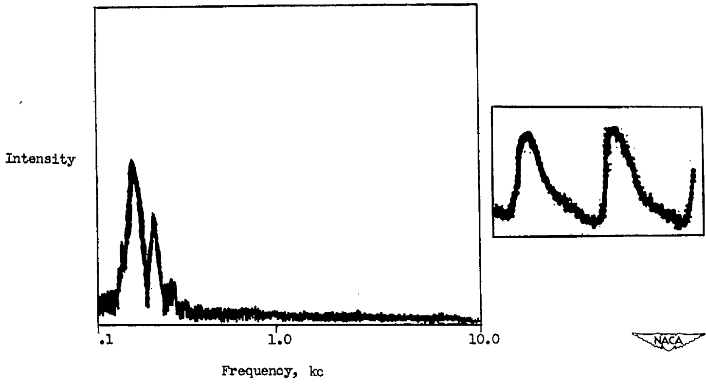
Figure 5.- Noise generated by a pulsing flow.
