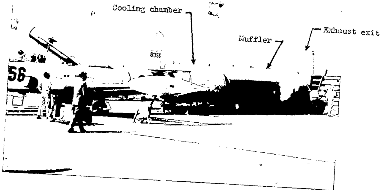
Figure 16.- Maxim silencer used by the Lockheed Aircraft Corp. for exhaust-noise reduction in the ground-testing of jet aircraft. (Photograph is reproduced by courtesy of the Maxim Silencer Co. of Hartford, Conn.)
