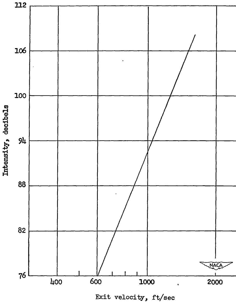
Figure 9.- Turbojet-engine noise as a function of the exit gas velocity. (Data correspond to a distance of 300 feet at an angle of 90° relative to the jet axis.)
