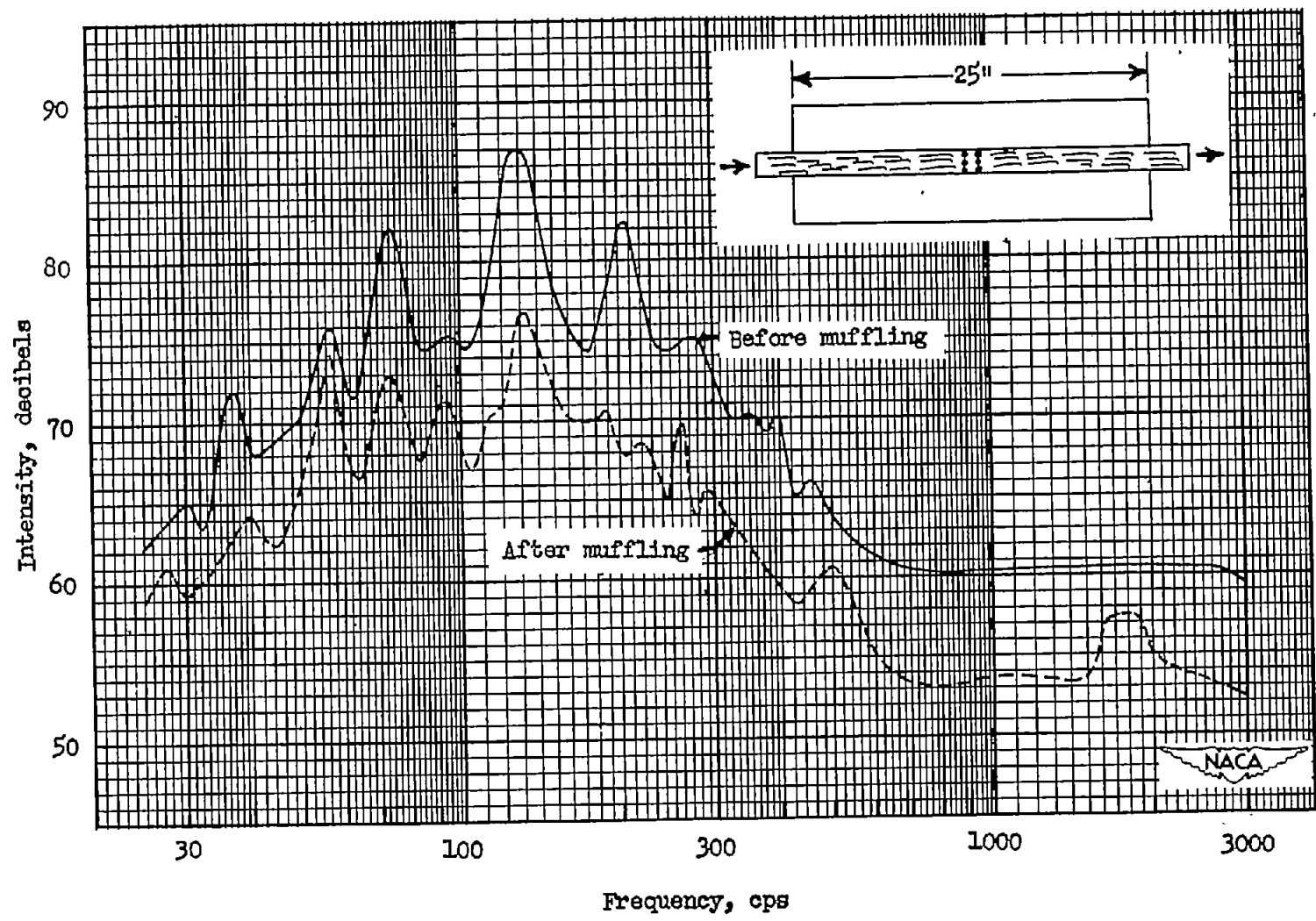
Figure 15.- Exhaust noise spectrums for a small reciprocating engine before and after muffling.
