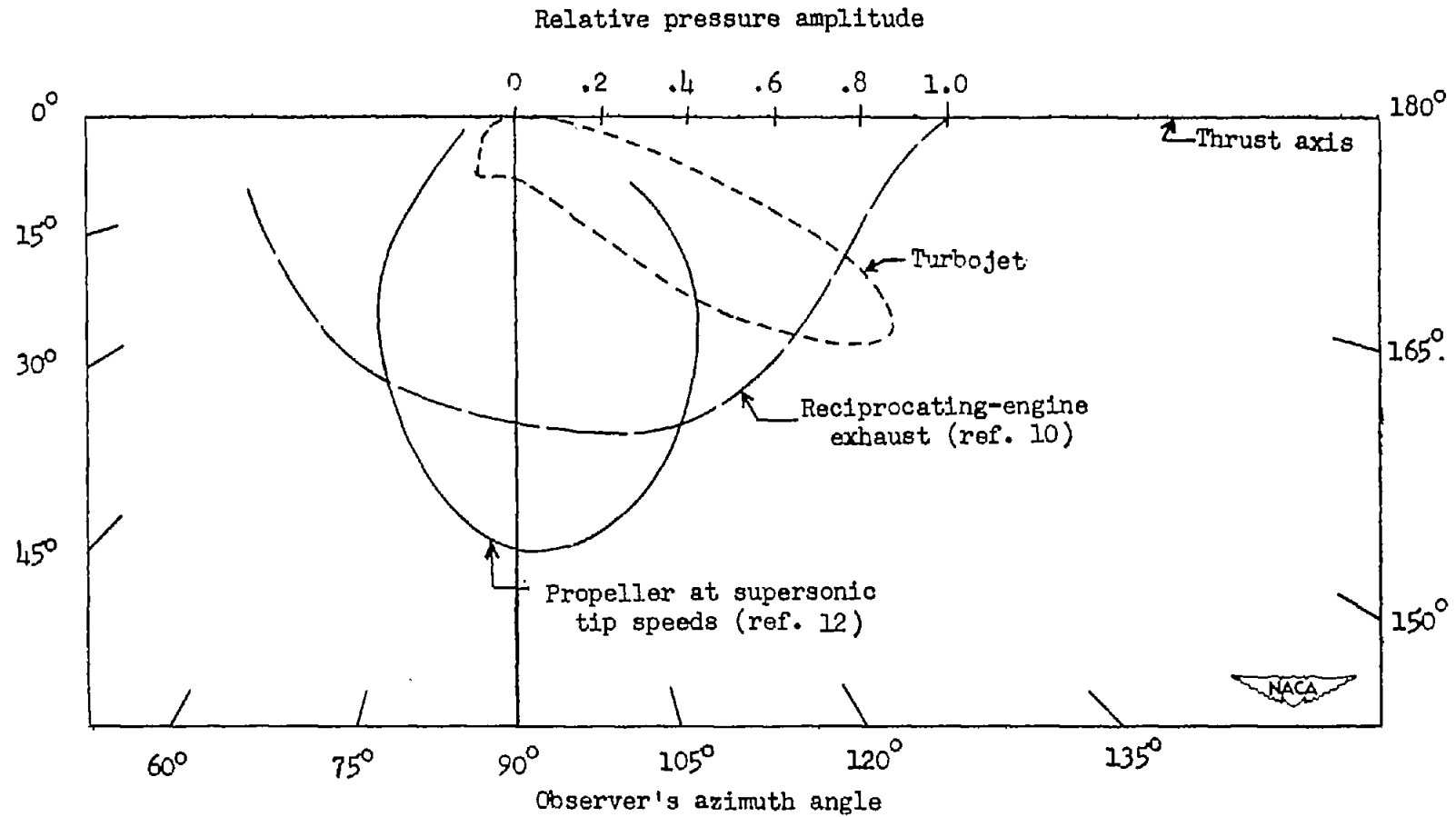
Figure 7.- Directional characteristics of the noise generated by three different types of aircraft-noise sources. (Data have been adjusted to equal maximum values for comparison.)
