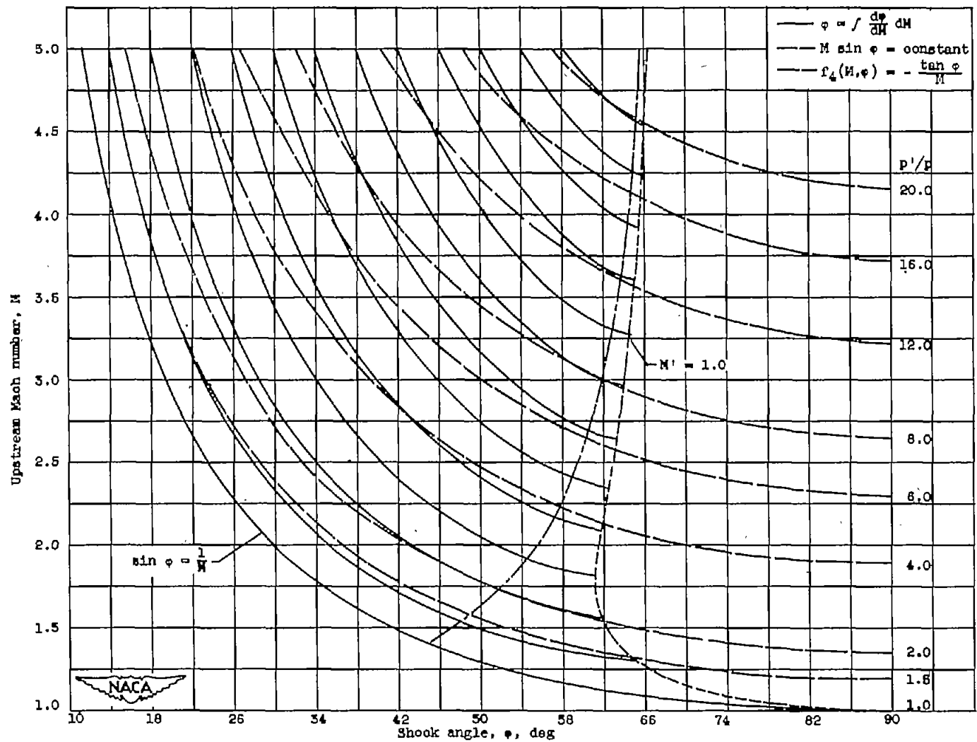
Figure 2. - Variation of shock angle with upstream Mach number. Constant upstream static pressure and flow angle. Ratio of specific heats, 1.40.
