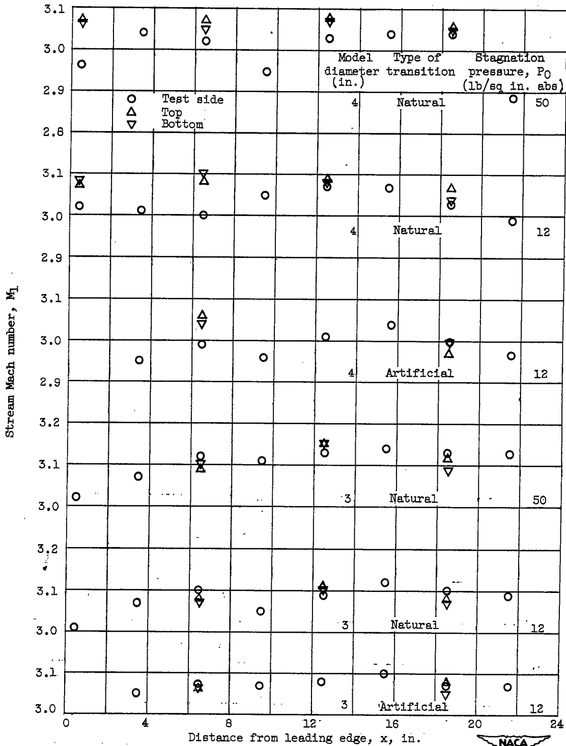
(c) Natural and artificial transition, 3- and 4-inch models.
