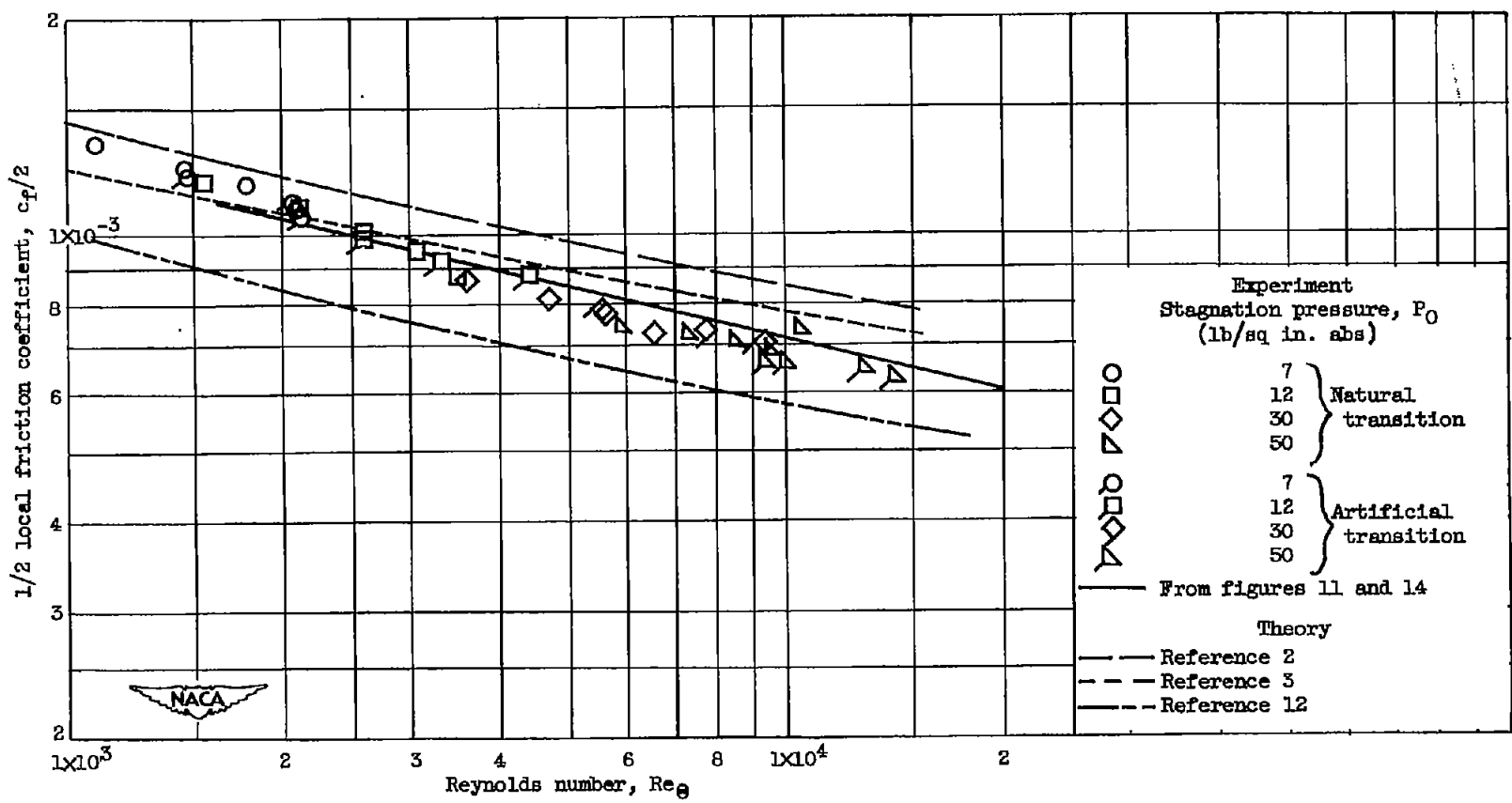
Figure 16. - Corrected measured friction coefficients as function of Re_\theta on 5-inch model. Natural and artificial transition.
