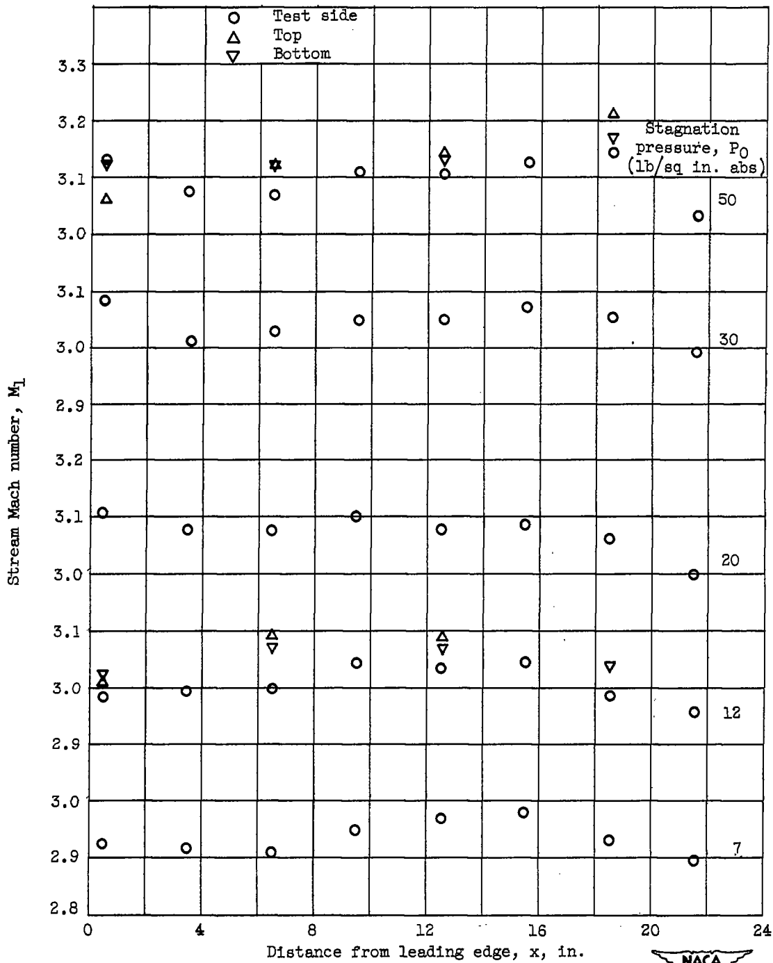
(a) Natural transition, 5-inch model.
