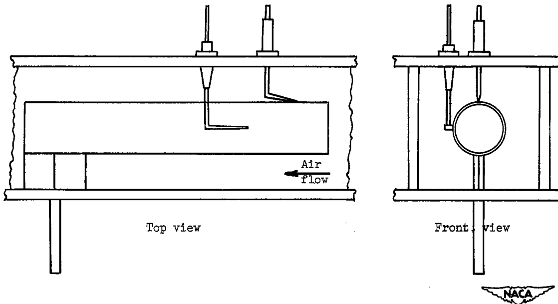
Figure 2. - Five-inch model in tunnel showing probe instrumentation.
