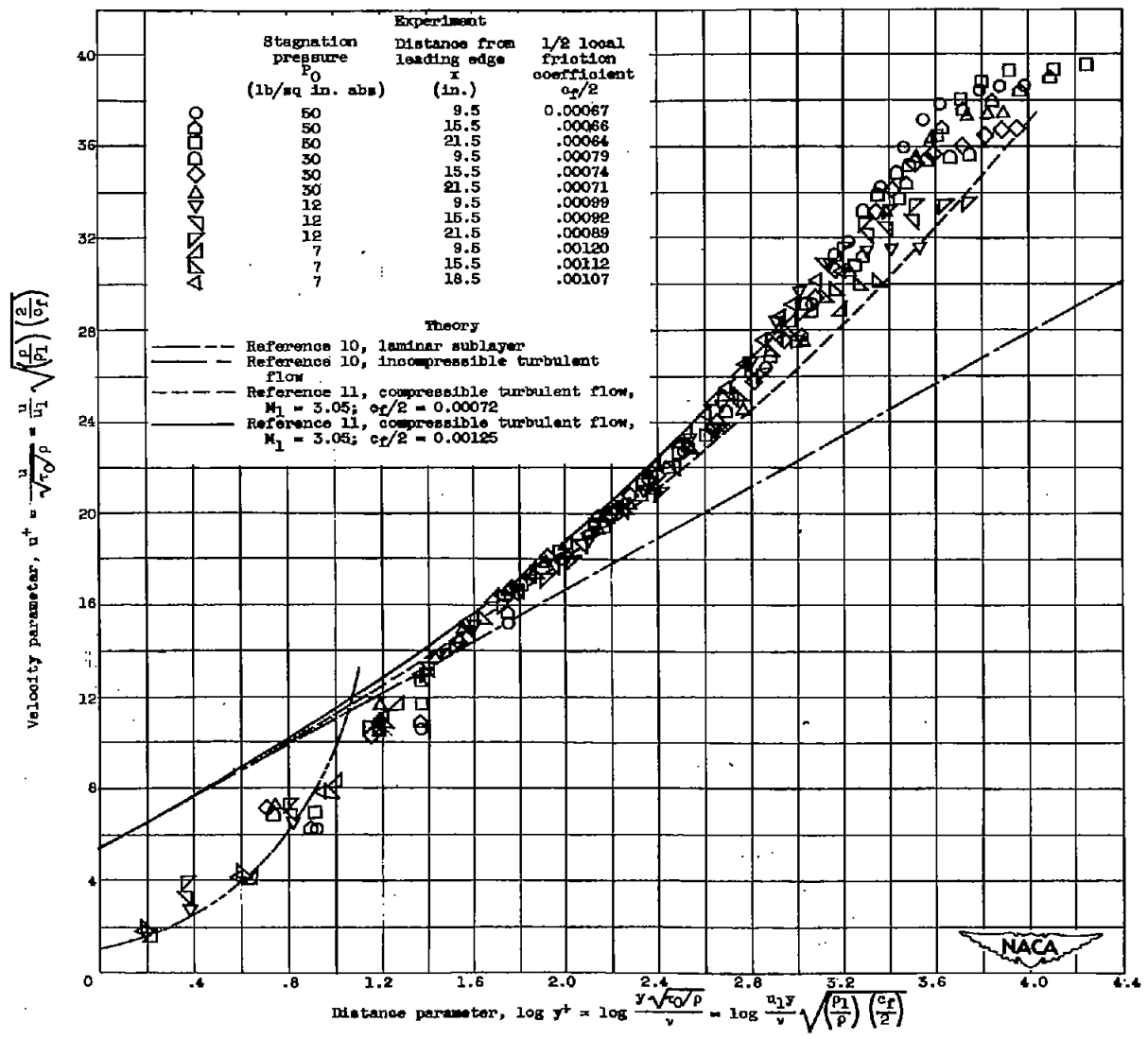
(b) Artificial transition.
