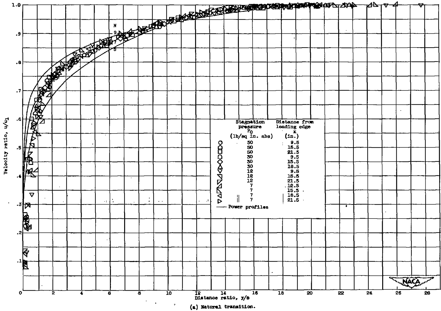
(a) Natural transition. Figure 10. - Turbulent velocity profiles and comparison with power profiles for 5-inch model. Side measurements.
