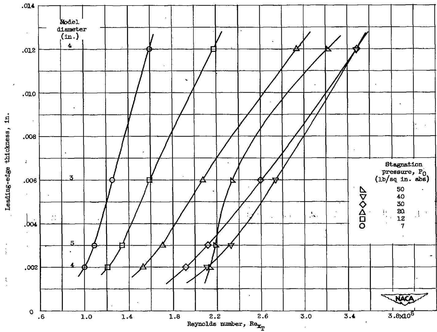
Figure 6. - Variation of transition Reynolds number with leading-edge thickness for all models.
