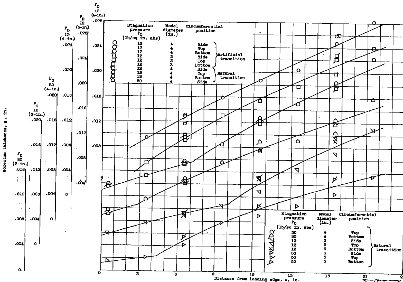
(a) Along 3- and 4-inch models, natural and artificial transition.
