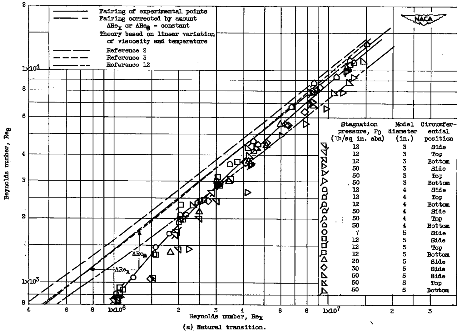
(a) Natural transition. Figure 11. - Variation of Re_0 with Re_x for 3-, 4-, and 5-inch cylinder models and comparison with theory. Top, side, and bottom measurements.
