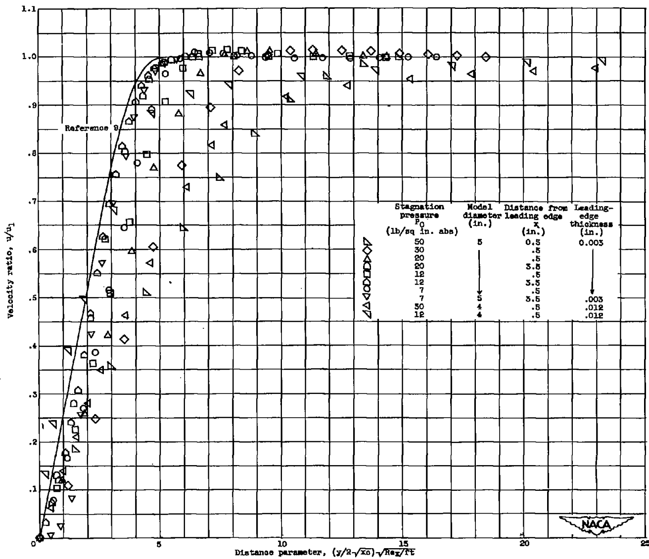
Figure 3: - Laminar velocity profiles and comparison with theory. Side measurements.
