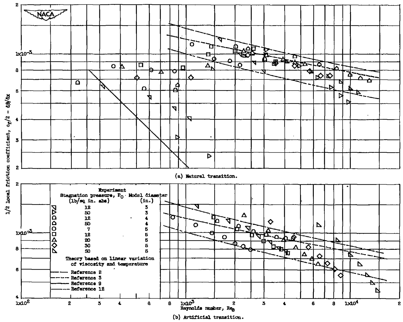
Figure 15. - Variation of local friction coefficient with Re_x for 3-, 4-, and 5-inch models.
