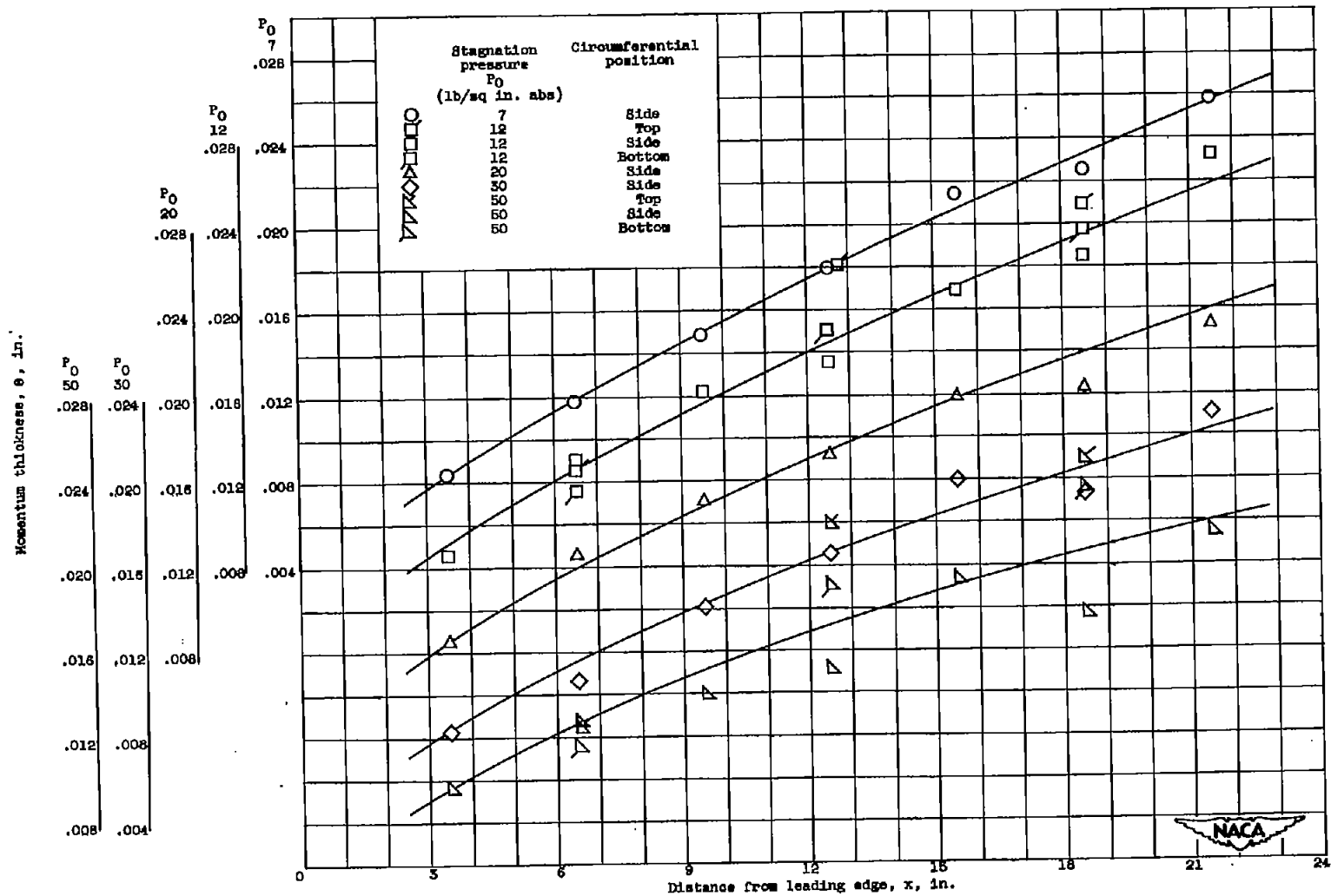
(b) Along 5-inch model, artificial transition.
