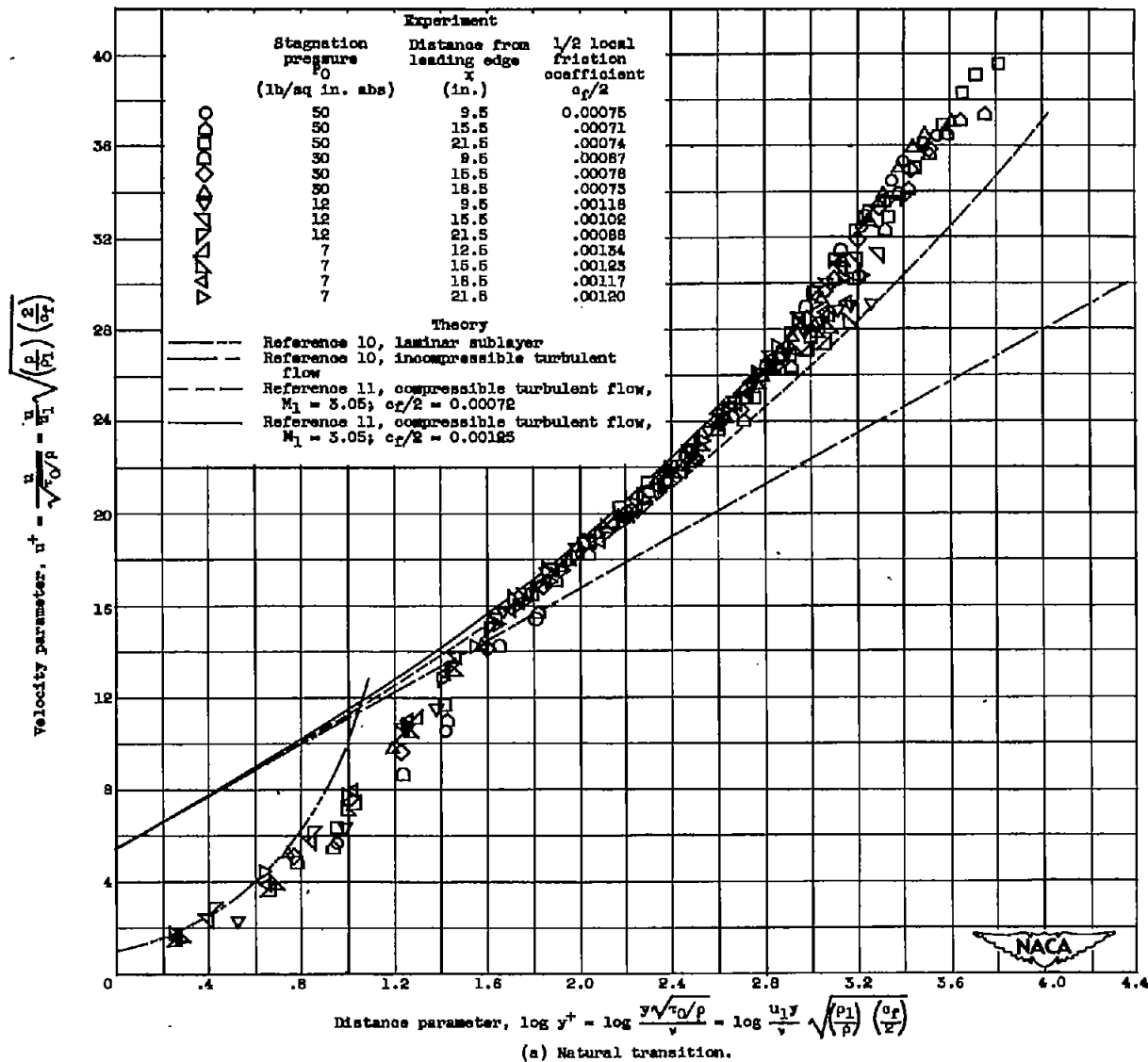
Figure 15. - Turbulent velocity profiles and comparison with theory. 5-inch model, side measurements.
