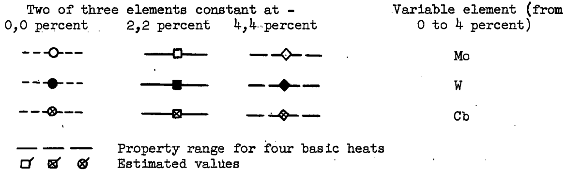
Figure 20.- Comparative influences of molybdenum, tungsten, and columbium on 1000-hour rupture strength at 1500° F of modified alloys.
