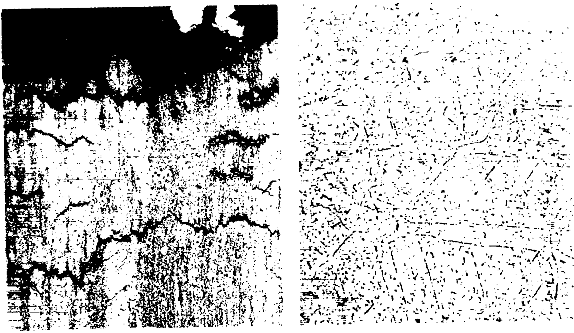
(c) Nickel, 30 percent (heat 26); 594 hours for rupture under 12,500 psi.
