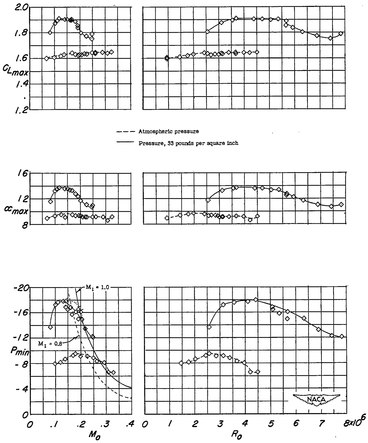
(c) 0.99-span split flaps deflected 60^\circ .
