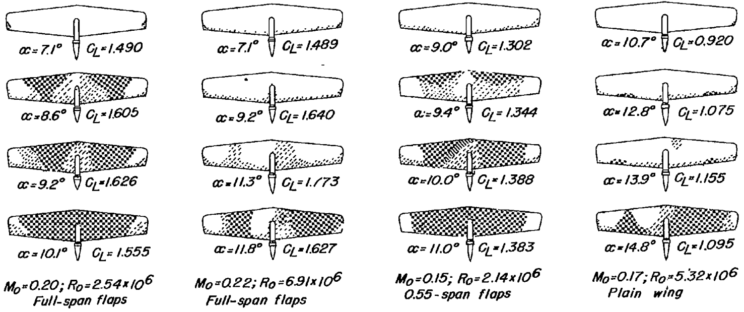
Figure 10.- Stalling patterns at various Mach numbers and Reynolds numbers for wing with full-span and partial-span flaps.
