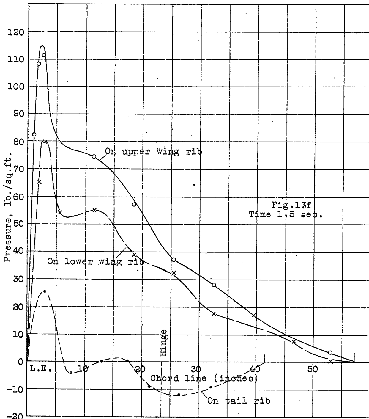
Fig.13f Pressure distribution on TS airplane in a pull-up with power off at 126 M.P.H.
