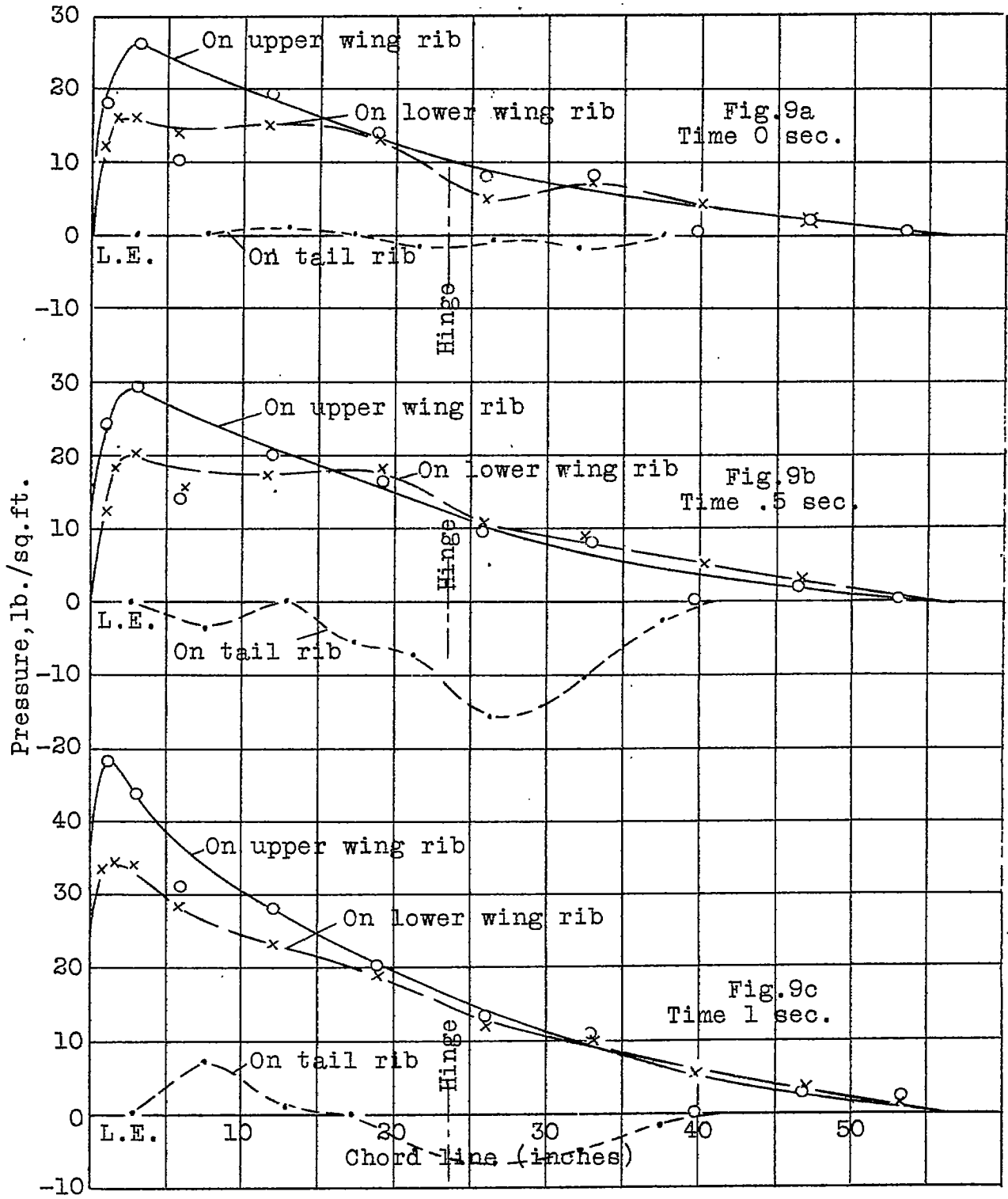
Figs.9a,b,c Pressure distribution on TS airplane in a pull-up at 63 M.P.H.
