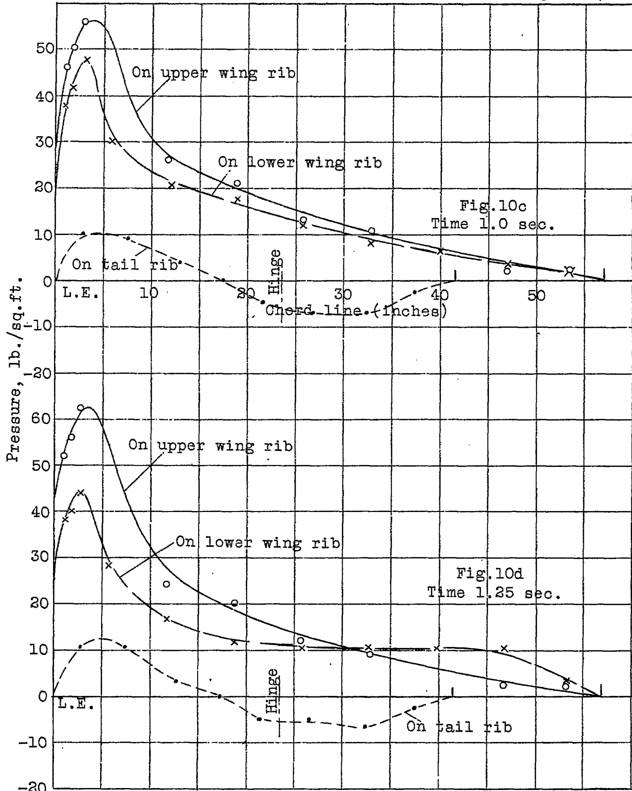
Figs.10c, d. Pressure distribution on TS airplane in a pull-up at 71 M.P.H.
