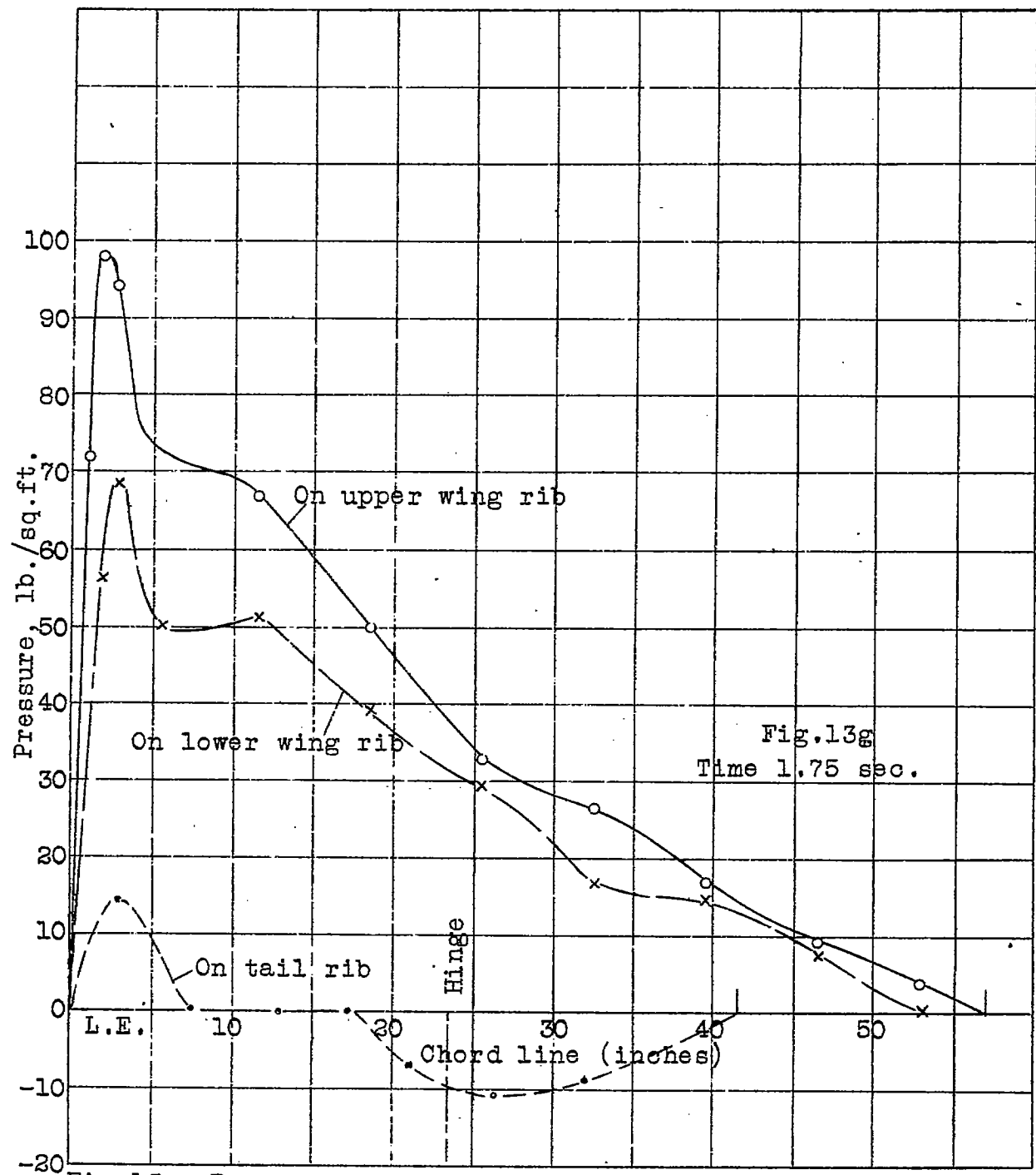
Fig.13g Pressure distribution on TS airplane in a pull-up with power off at 126 M.P.H.
