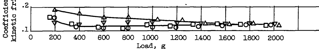
Figure 6. - Effect of temperature on coefficient of friction of solution of one-third di(2-ethylhexyl) sebacate and two-thirds silicone fluid (10 cs at 25° C) which contained 2 percent tricresyl phosphate.
