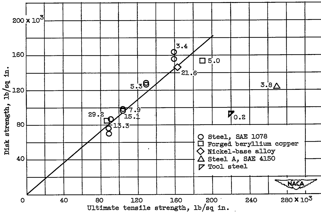
(c) Disks with \frac{1}{2} -inch-diameter central holes.
