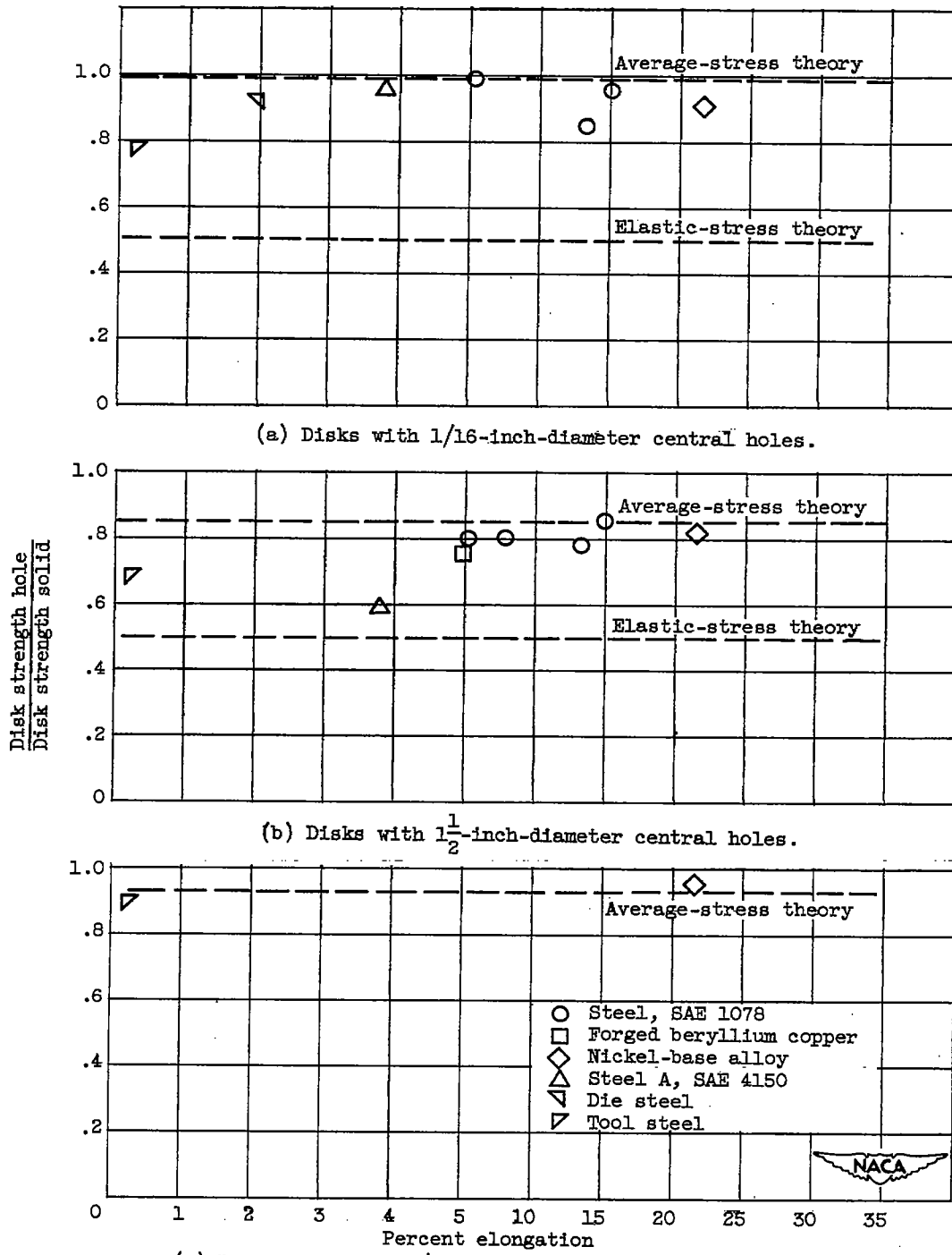
Figure 10. - Relation between ductility and strength reduction due to presence of holes.
