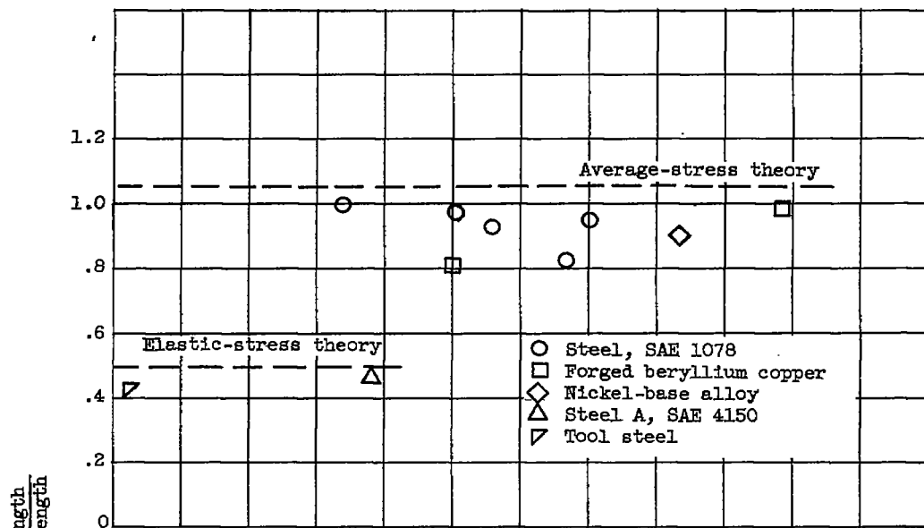
(c) Disks with 1/2-inch-diameter central holes.
