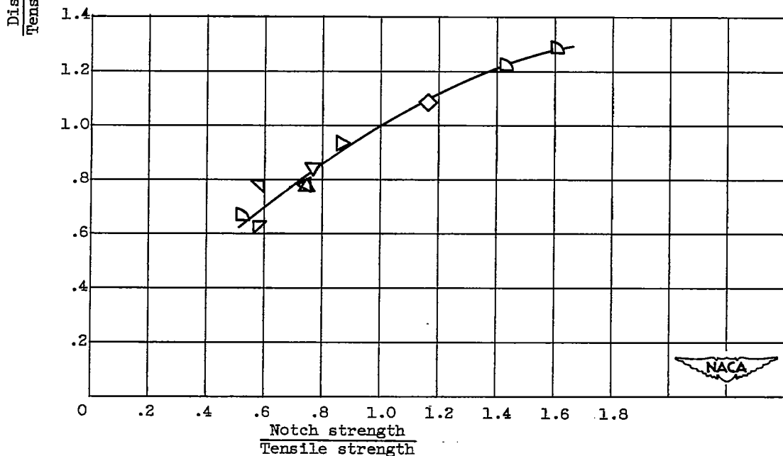
(b) Correlation with stress concentration resistance.
