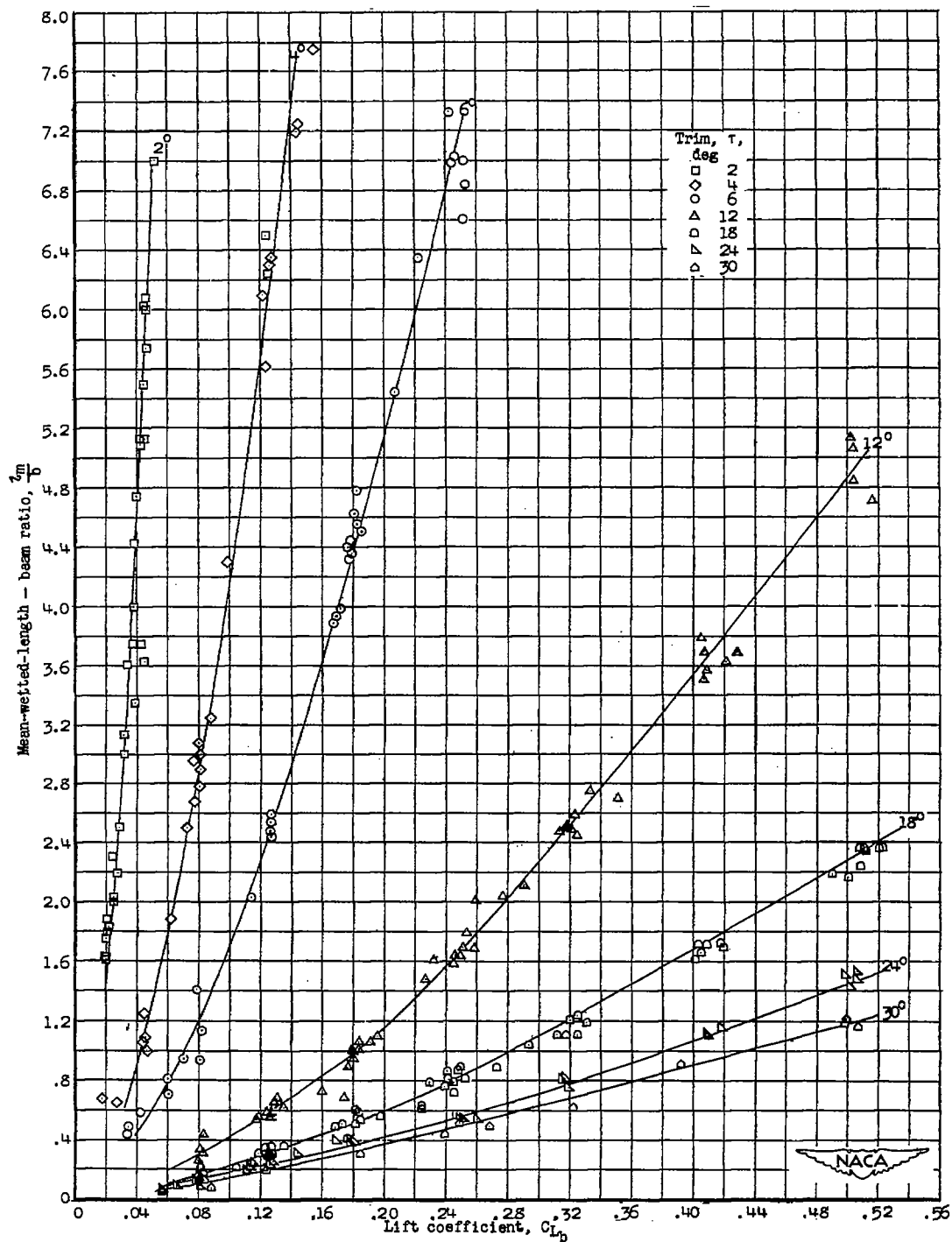
Figure 9.- Variation of mean-wetted-length-beam ratio l_m/b with lift coefficient C_{Lb} .
