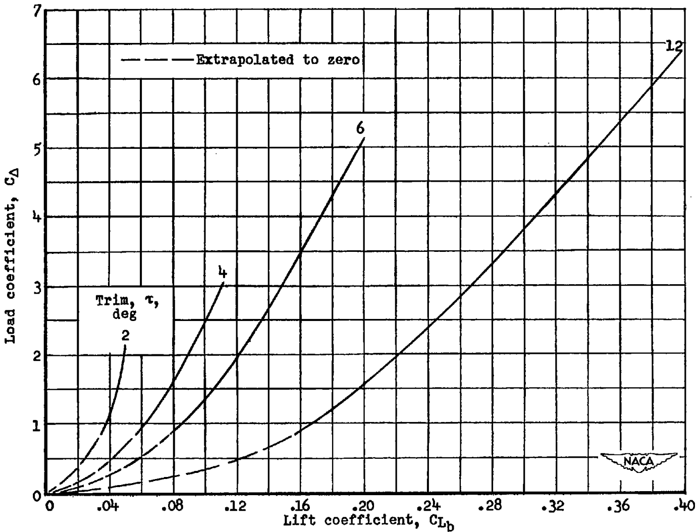
Figure 18.- Curves defining the variation of minimum load coefficient for pure planing.
