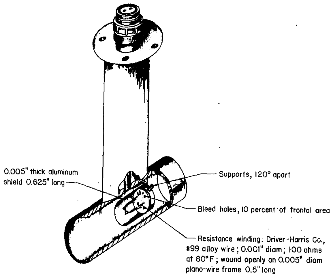
Figure 1.- Adiabatic-type resistance sensing element.
