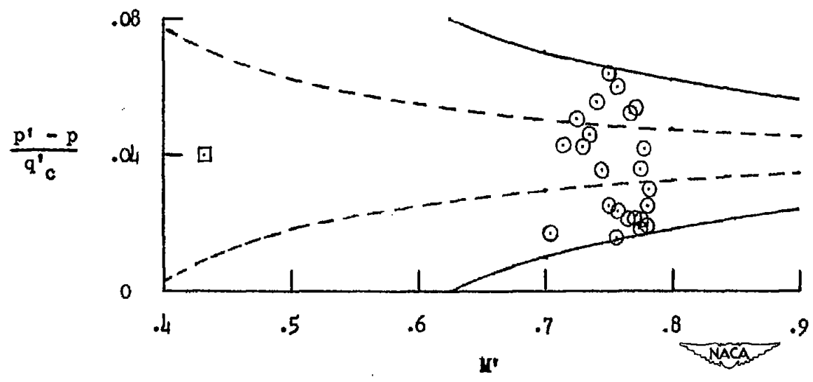
Figure 6.- Error in static pressure determined by evaluation of surveys and dive made on April 13.
