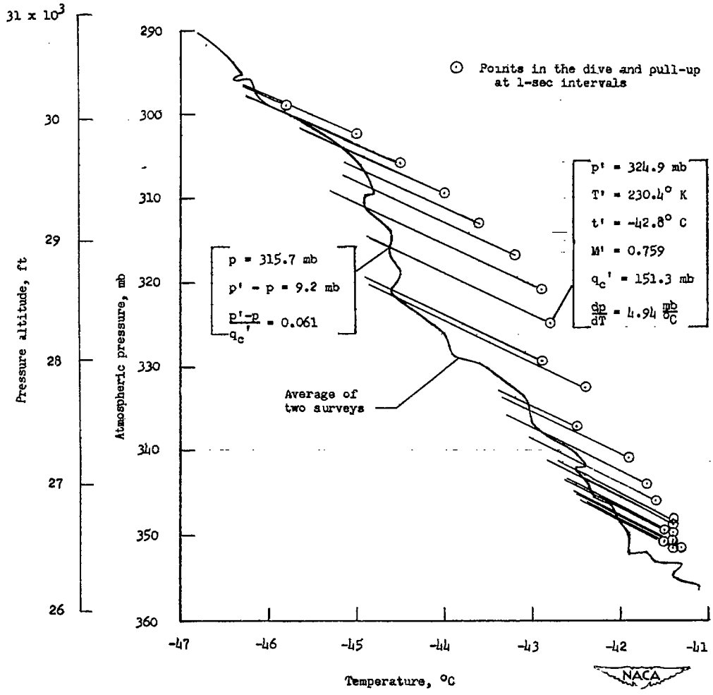
Figure 5.- Determination of free-stream pressure in the dive by the temperature method by using the average of the two surveys made in climbing flight on April 13.
