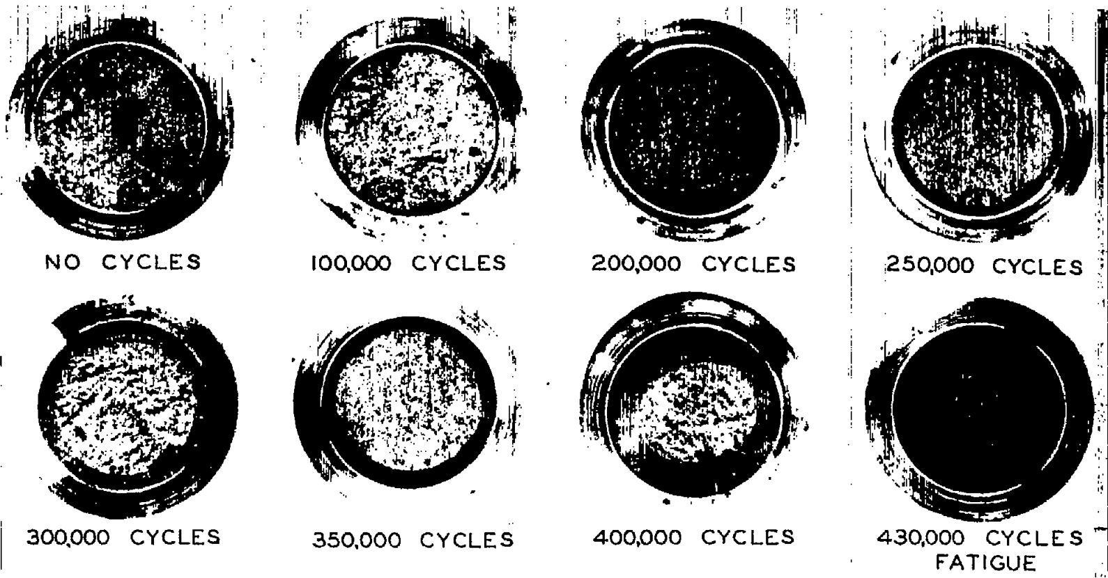
(a) SAE 4130 steel; nominal fatigue bending stress, 33,000 psi.
