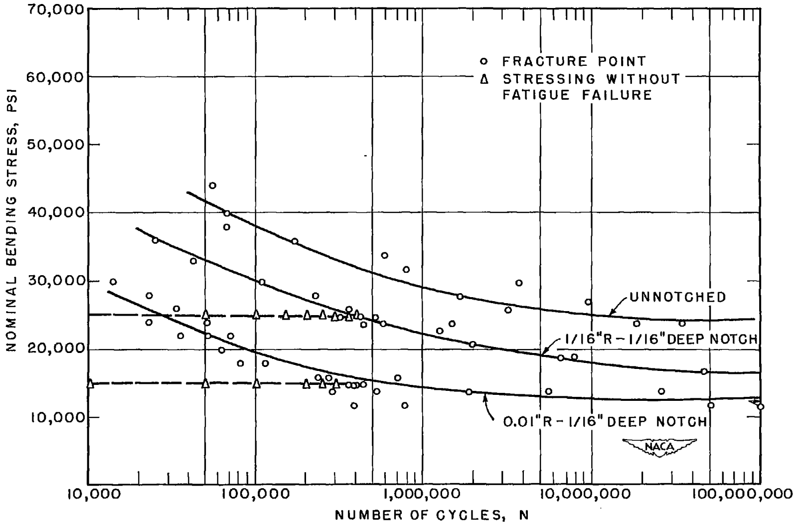
(c) For 75S-T6 aluminum alloy.
