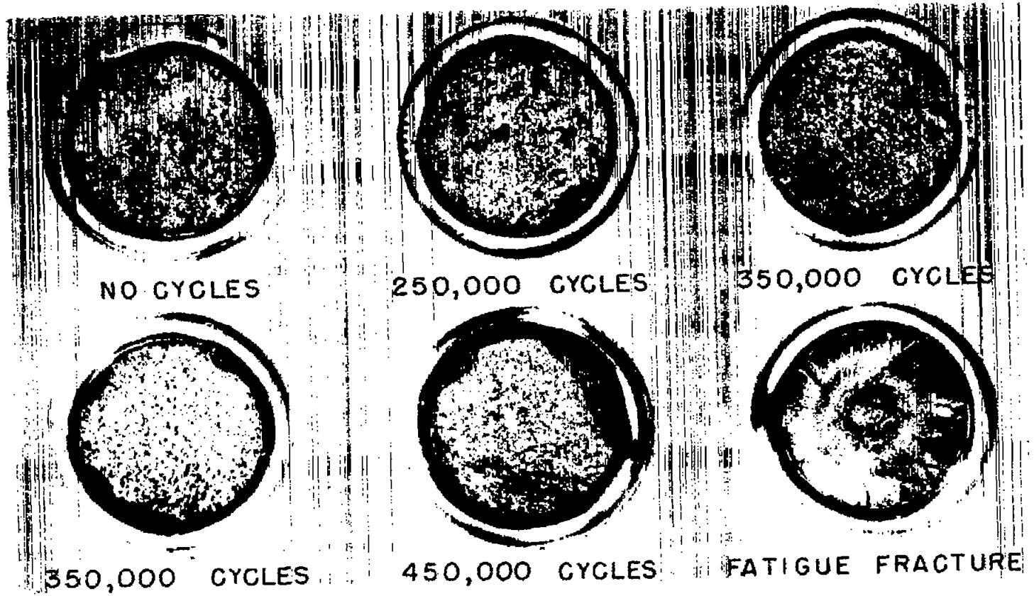
(a) SAE 4130 steel; nominal fatigue bending stress, 46,000 psi.
