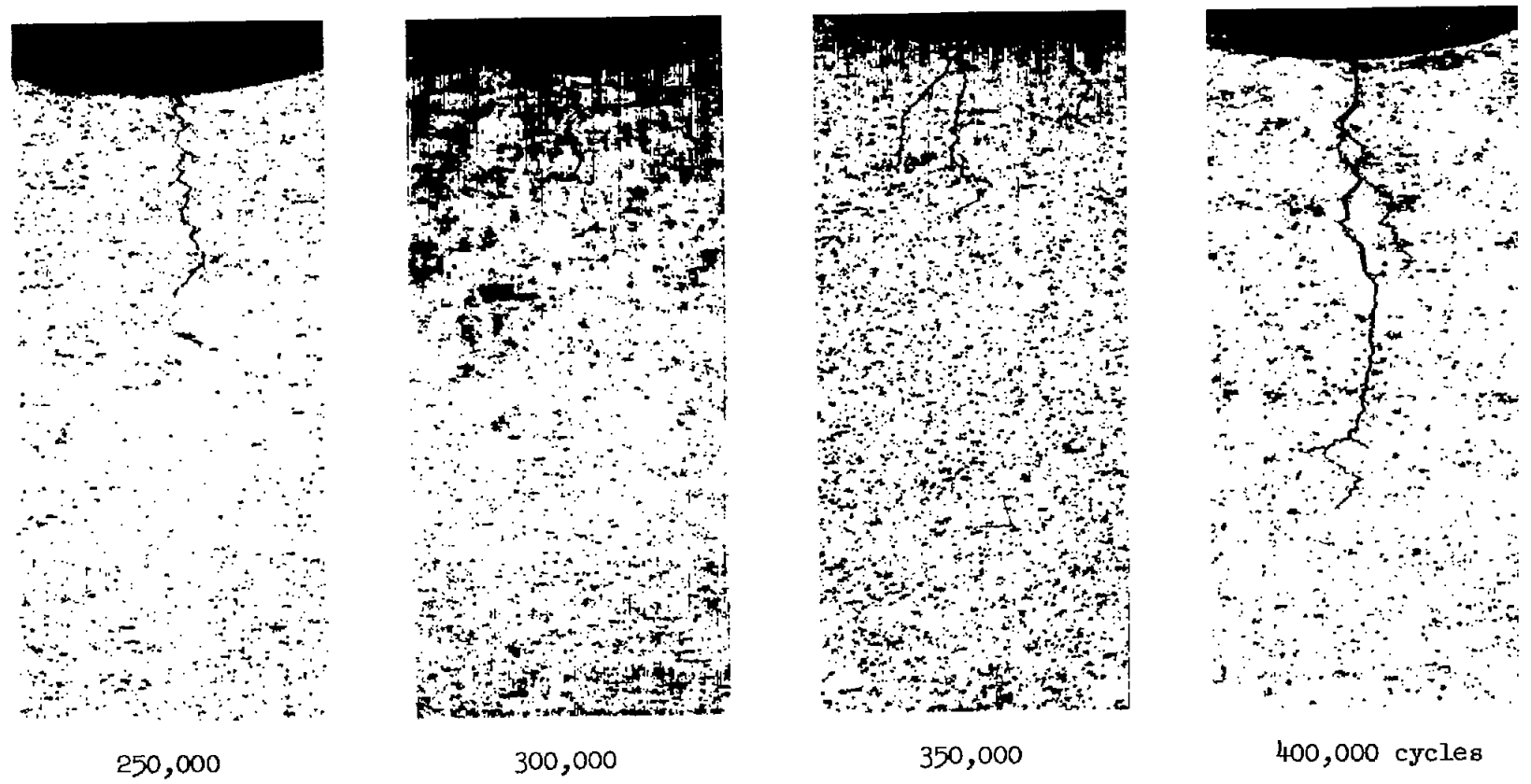
(b) 24S-T4 aluminum alloy; nominal fatigue bending stress, 26,000 psi.
