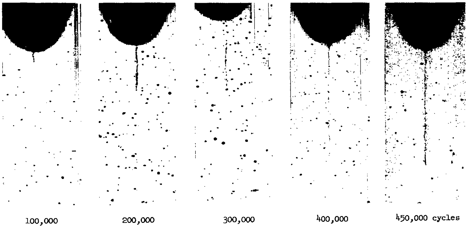
(a) SAE 4130 steel; nominal fatigue bending stress, 33,000 psi.
