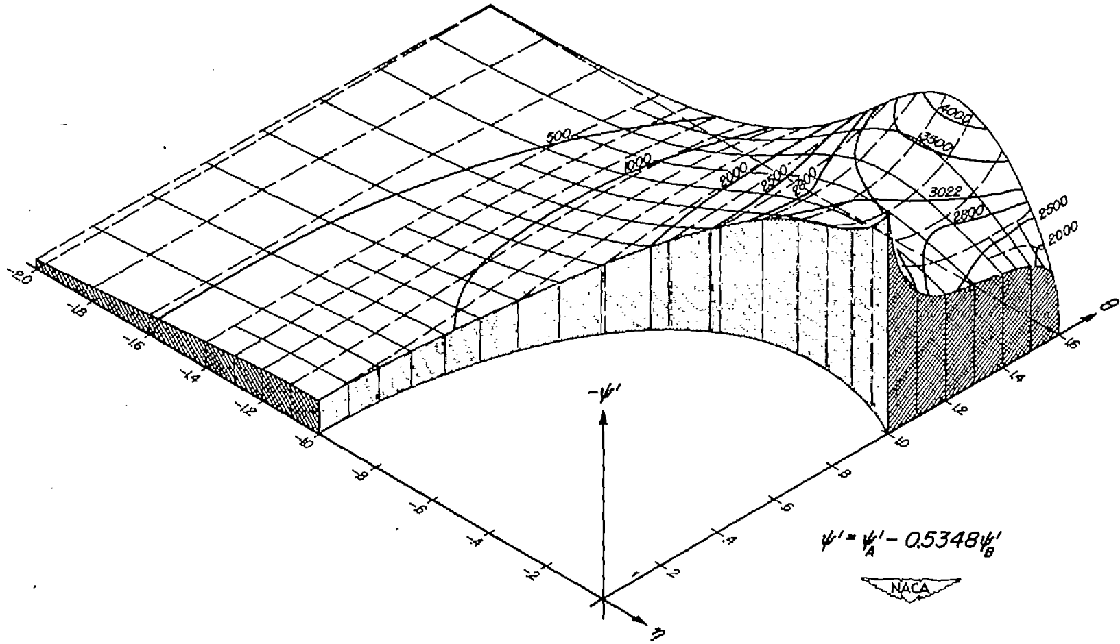
Figure 3.—The variation of \psi' as a function of \eta and \theta for \theta_w = 1.6 ( \xi_0 = 0.921 ).
