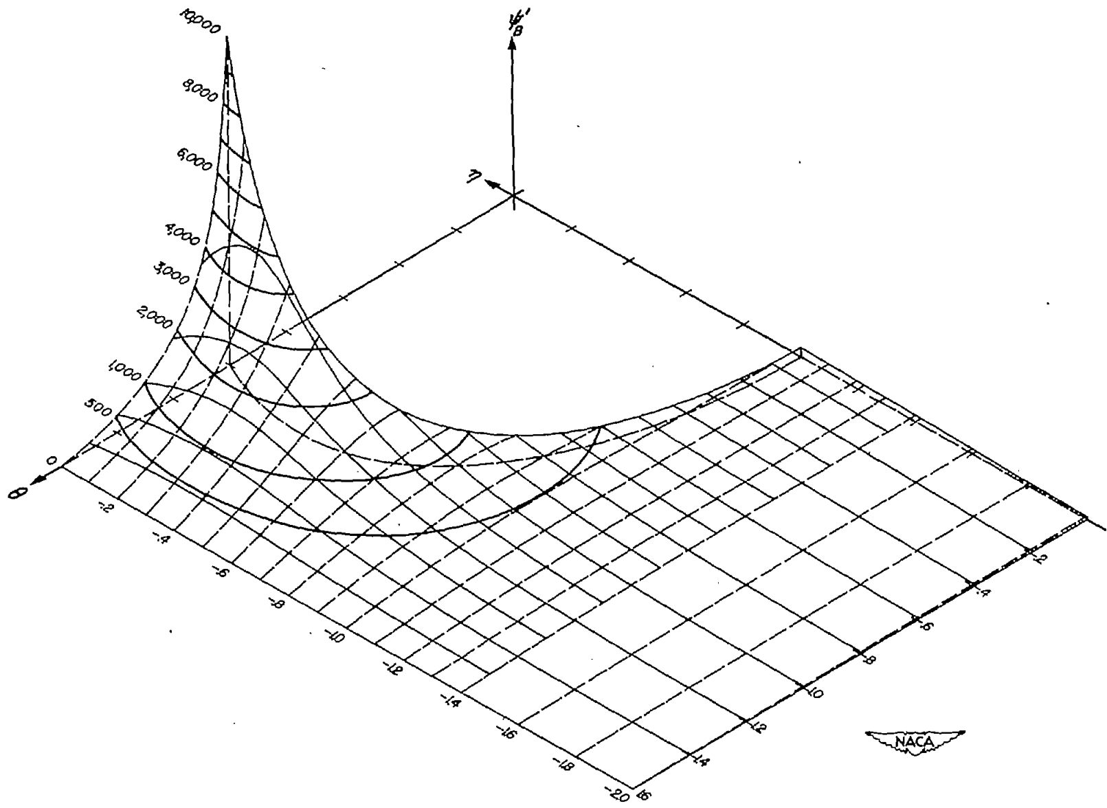
Figure 1.—The variation of \psi_B' as a function of \eta and \theta for \theta_w = 16 ( \xi_0 = 0.921 ).
