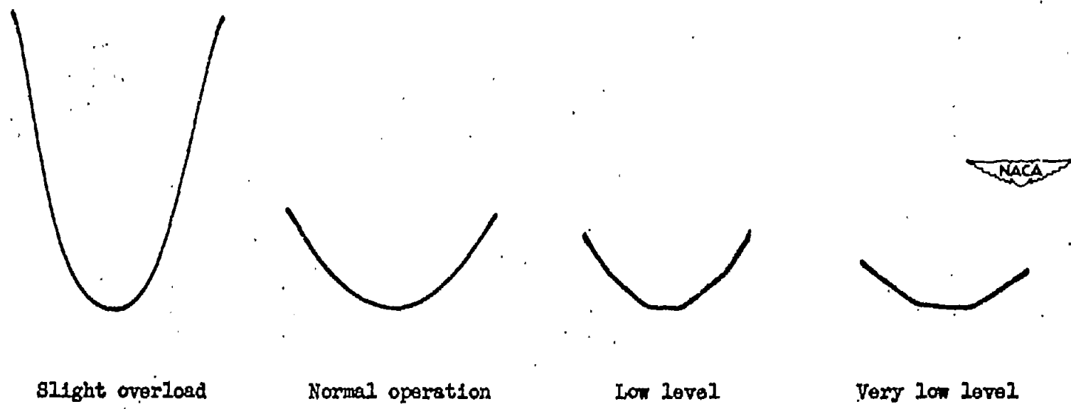
Figure 40.- Amplitude response of square-law circuit. Amplification readjusted for each oscillograph. Frequency, 100 cycles per second.
