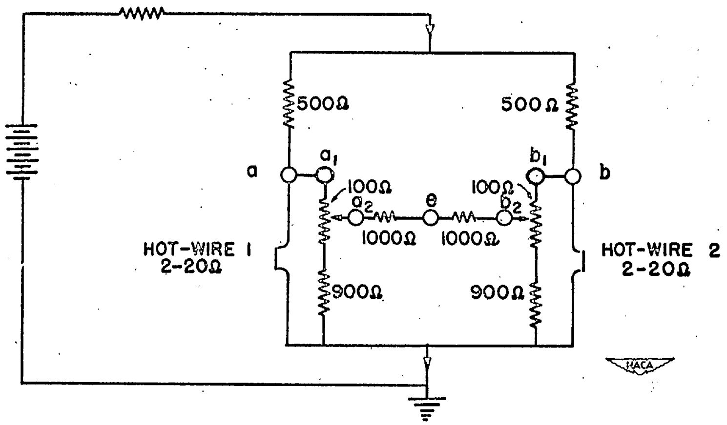
Figure 16.- Matching circuit.
