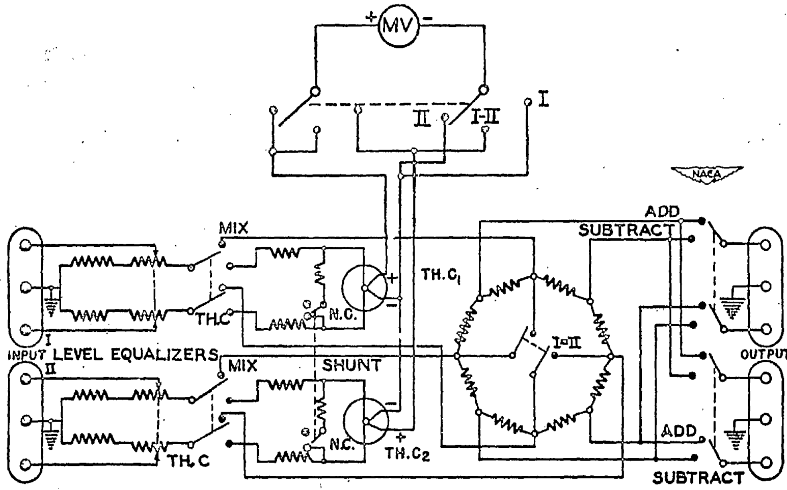
Figure 35.- Service-unit circuit.
