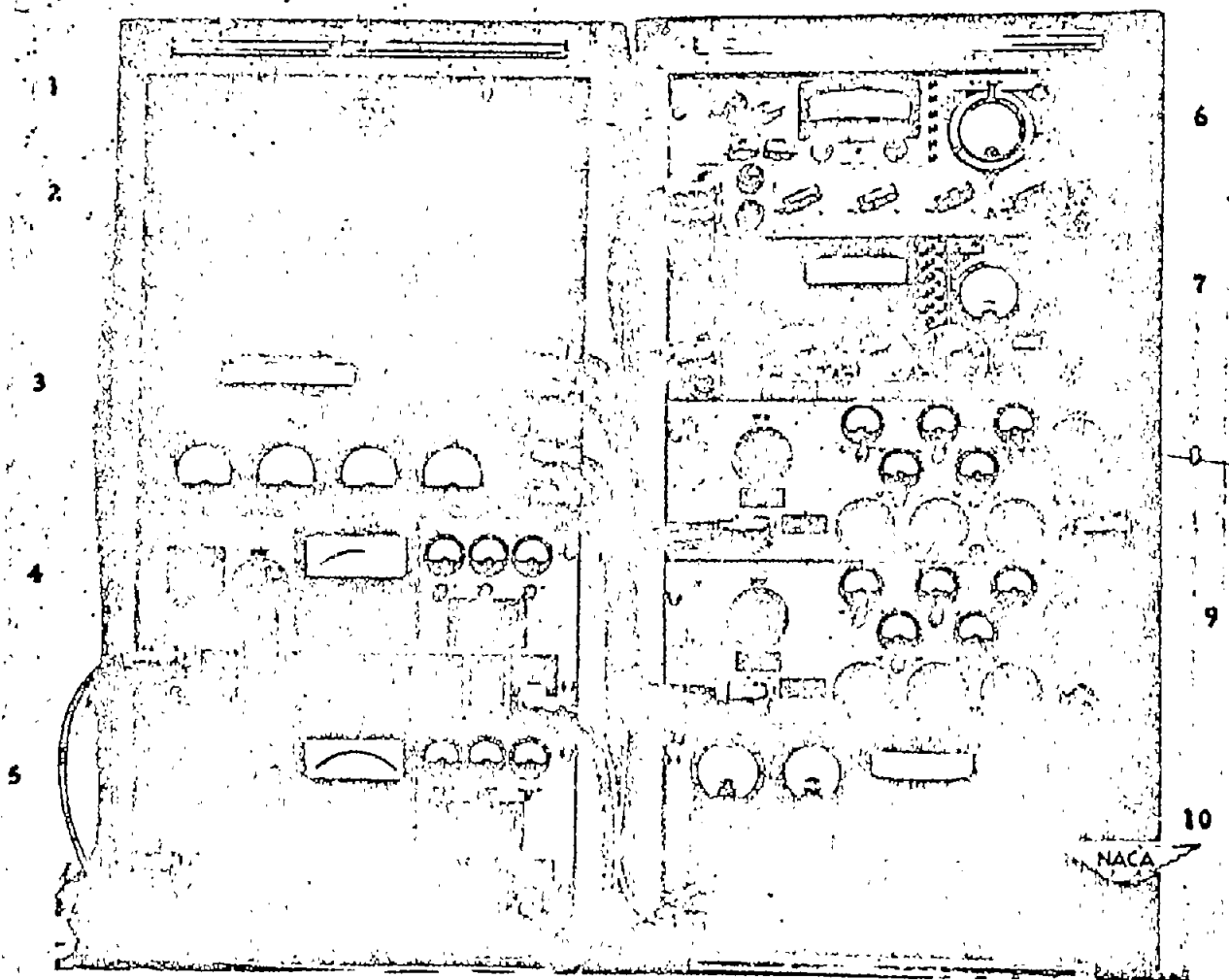
Figure 10.- Hot-wire turbulence equipment. 1 and 2, power supplies; 3, service unit; 4 and 5, power units; 6 and 7, control units; 8 and 9, compensating amplifiers; 10, calibration unit.
