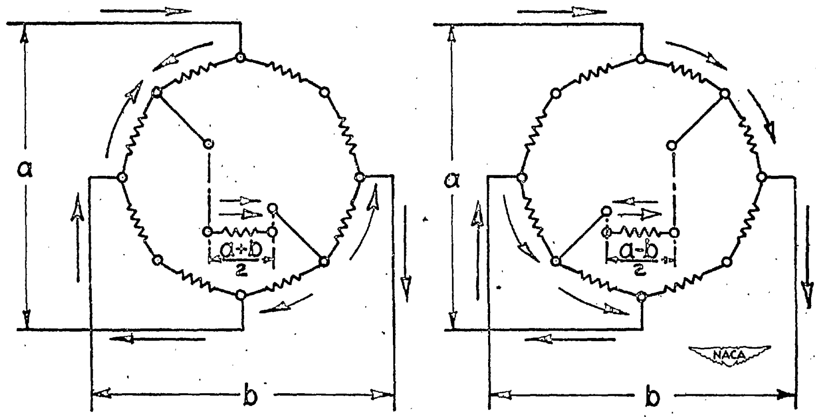
Figure 36.- Sum-difference circuit.
