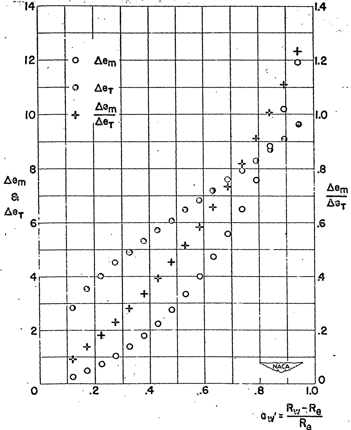
Figure 8.- Variation of fluctuation sensitivities with wire temperature in supersonic flow. Tungsten wire with 0.0015-inch diameter was used. Flow conditions: M = 1.73 , T_0 = 293^\circ K , and pressure at stagnation temperature was 40 centimeters of mercury.
