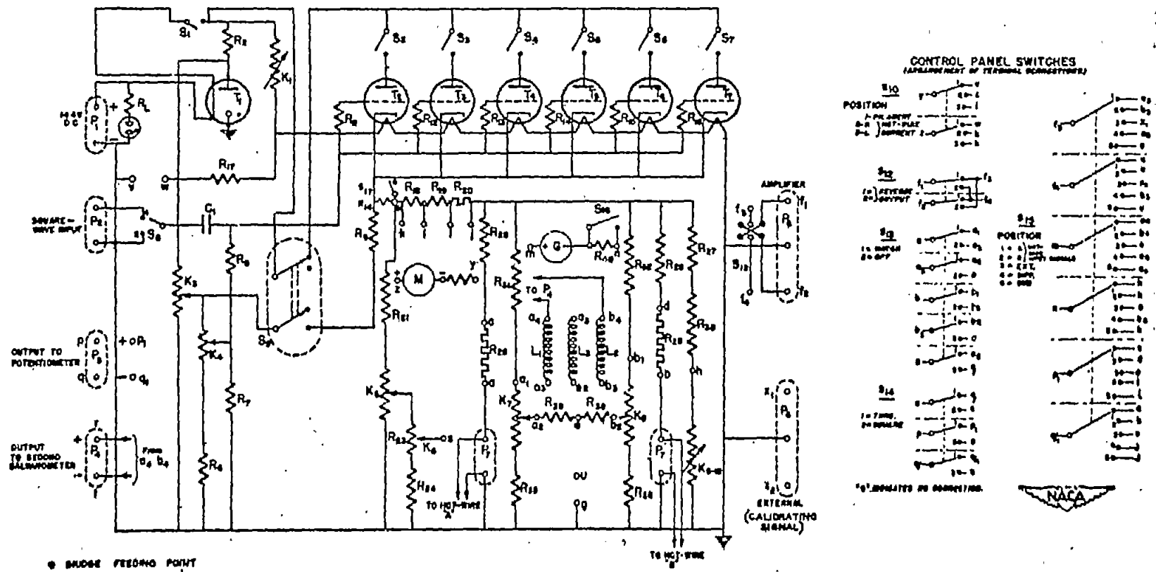
Figure 11.- Basic diagram of control unit.
