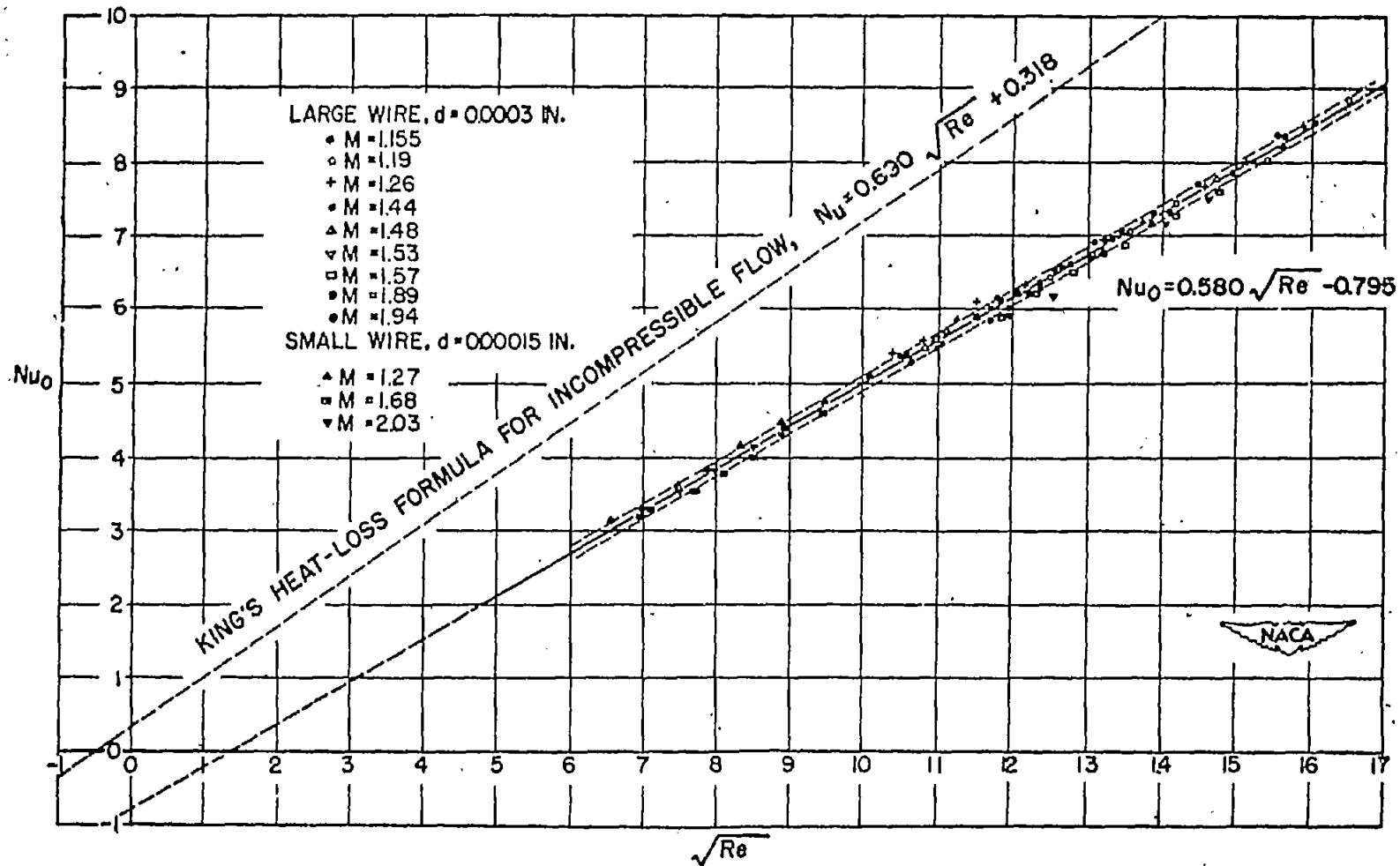
Figure 7.- Heat loss of wire at supersonic speeds. Re = \frac{\rho u d}{\mu_0} ; Nu_0 = \frac{H}{\pi r \Delta T k_0} ; standard deviation of Nu_0 is 0.098.
