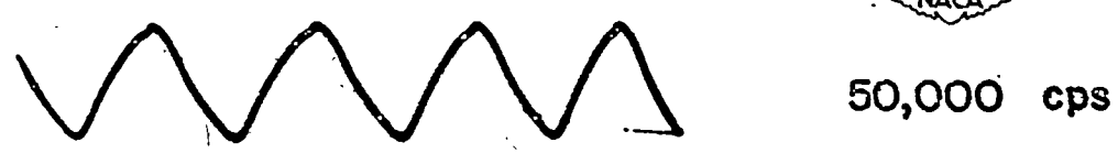
Figure 31.- Response of compensation to very high frequency square waves.
