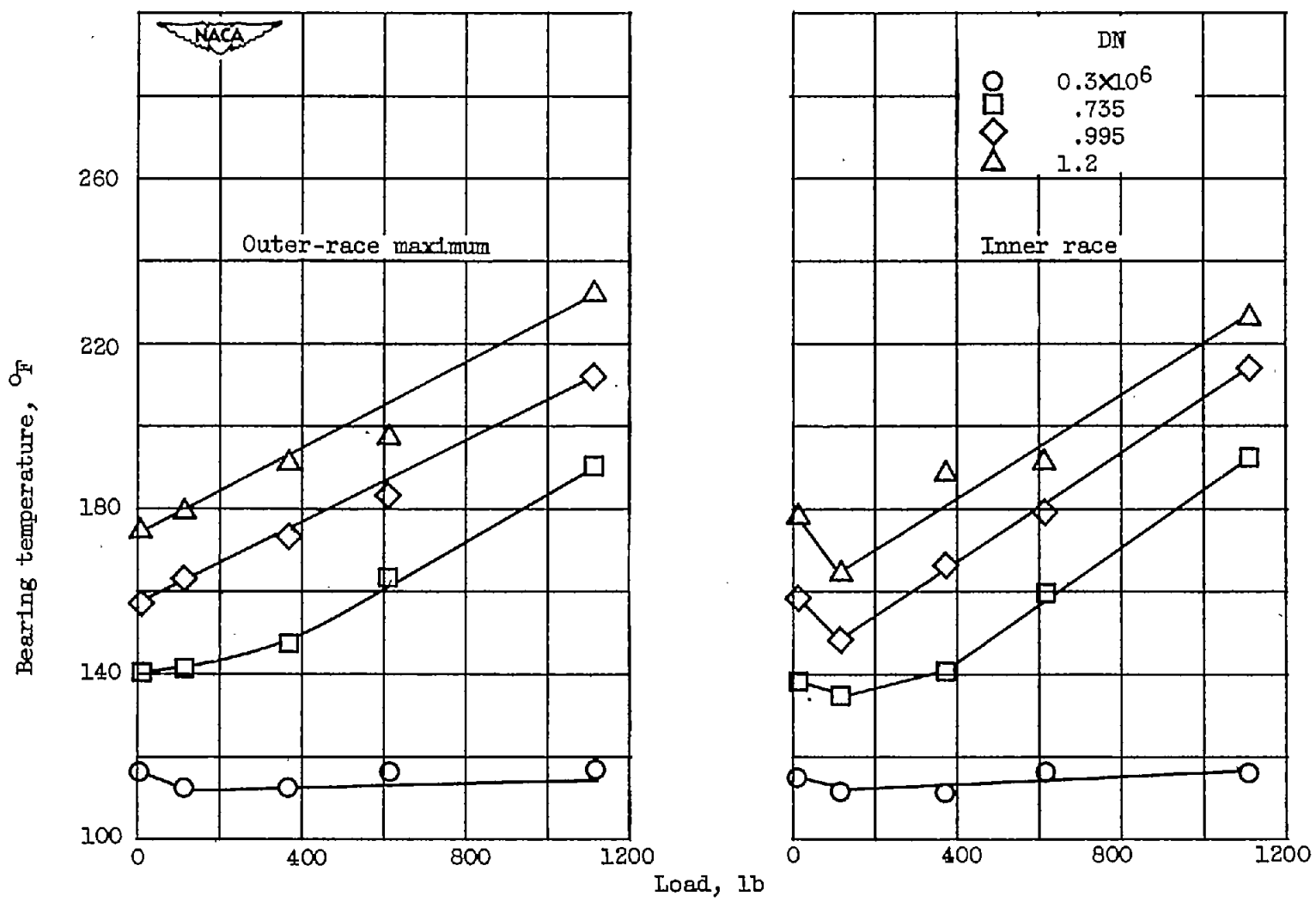
Figure 13. - Effect of load on outer-race-maximum and inner-race temperatures of bearing 19. DN, 0.3 \times 10^6 , 0.735 \times 10^6 , 0.995 \times 10^6 , 1.2 \times 10^6 ; oil flow, 2.75 pounds per minute; oil inlet temperature, 100° F; oil-jet diameter, 0.050 inch.
