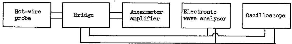
(f) Spectrum of turbulence measurements (method 2).
