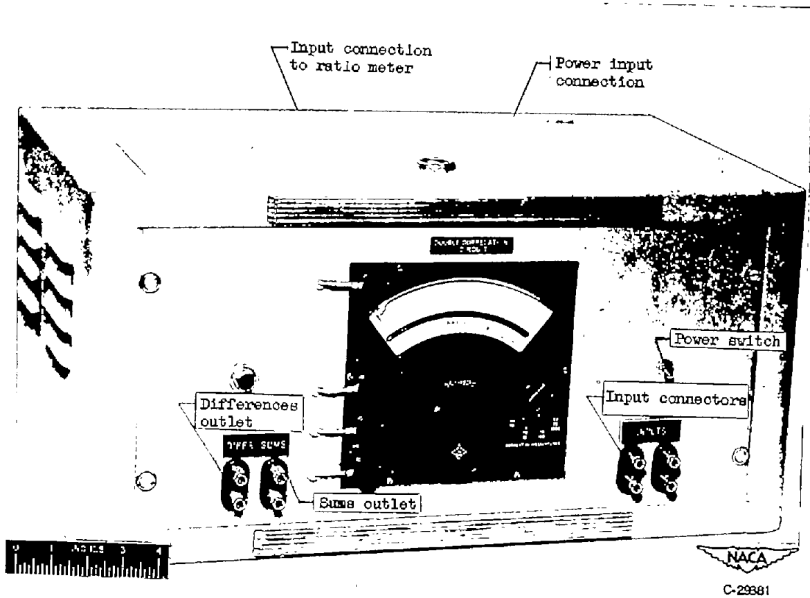
Figure 32. - Double-correlation instrument.
