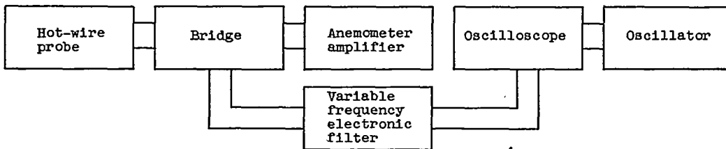
(c) Compressor surge and rotary stall measurements.
