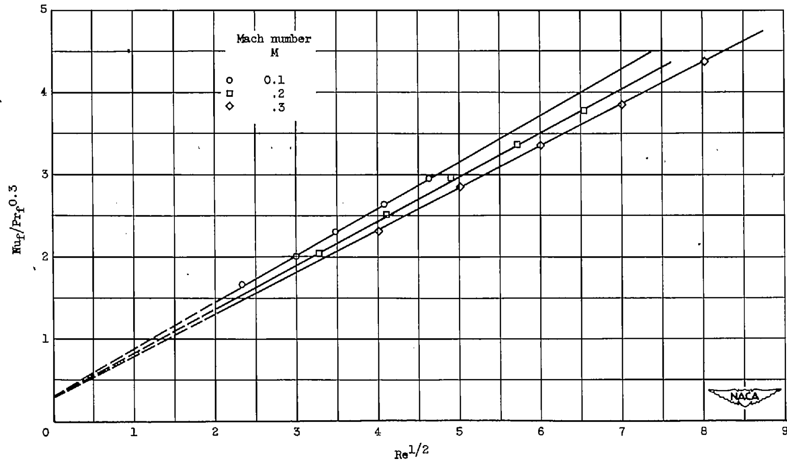
(a) Wire temperature, 213° F.
