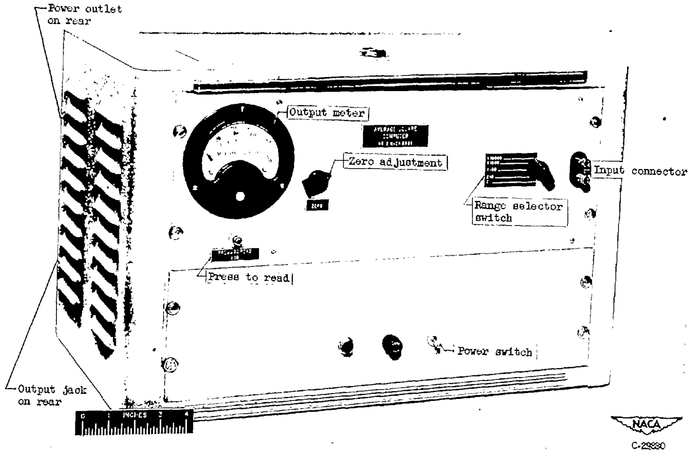
Figure 30. - Average-square computer.
