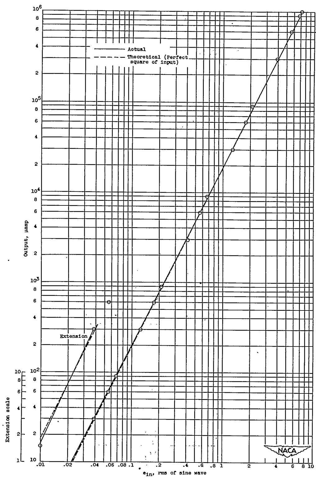
Figure 12. - Calibration for average-square computer number 2.
