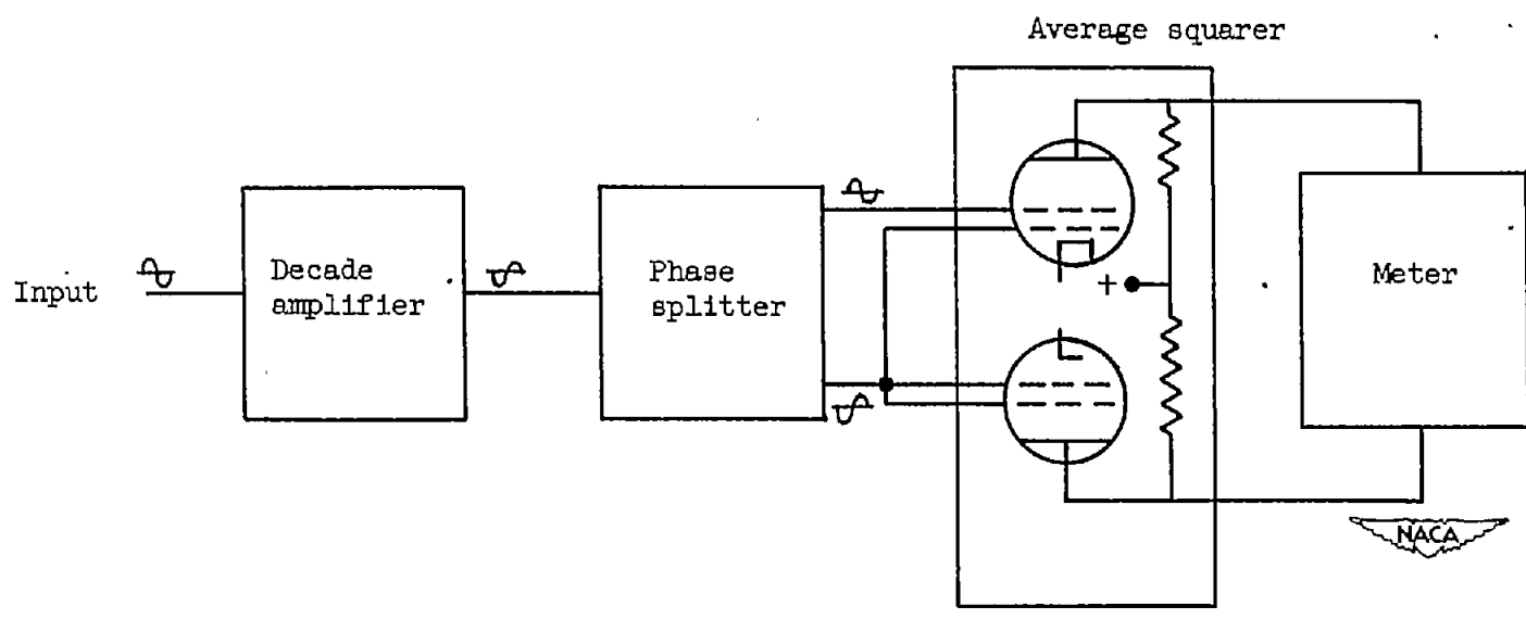
Figure 9. - Simplified diagram of average-square computer.
