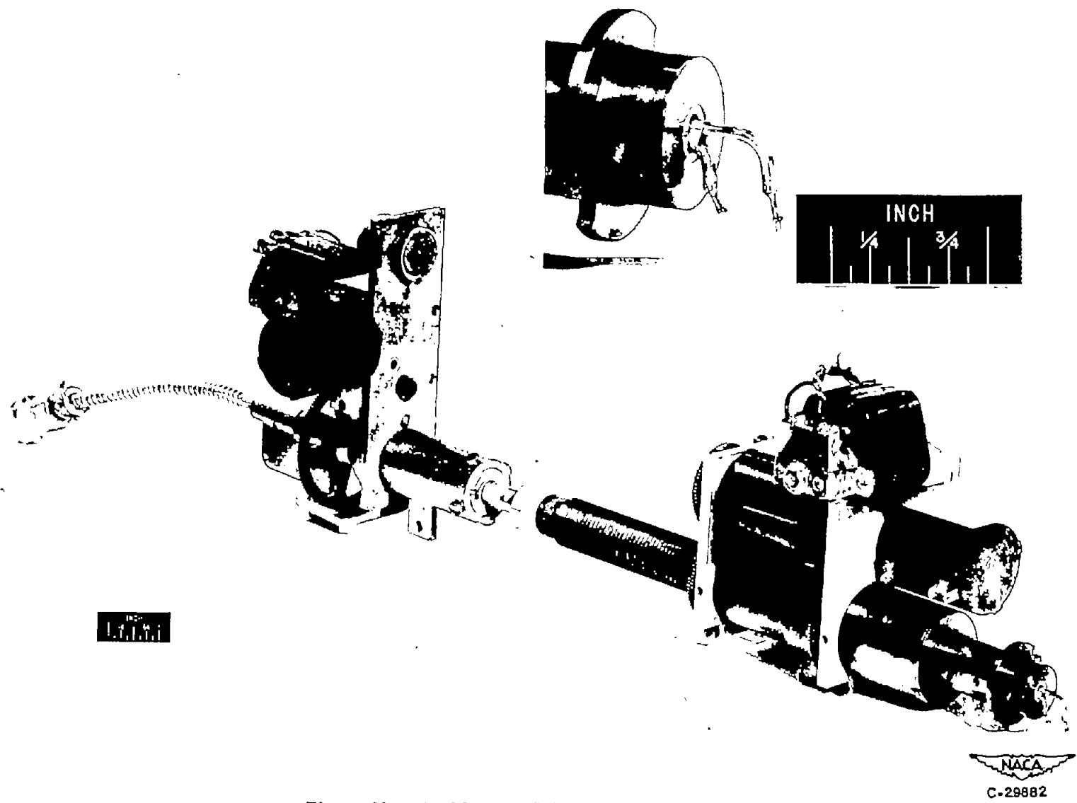
Figure 28. - Double-correlation probe and actuators.
