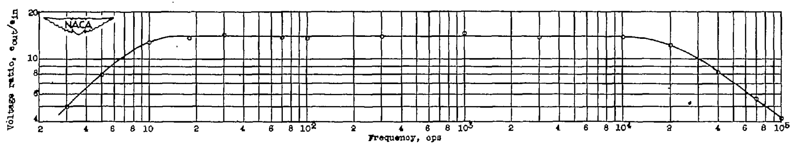
Figure 16. - Frequency response for double-correlation computer.
