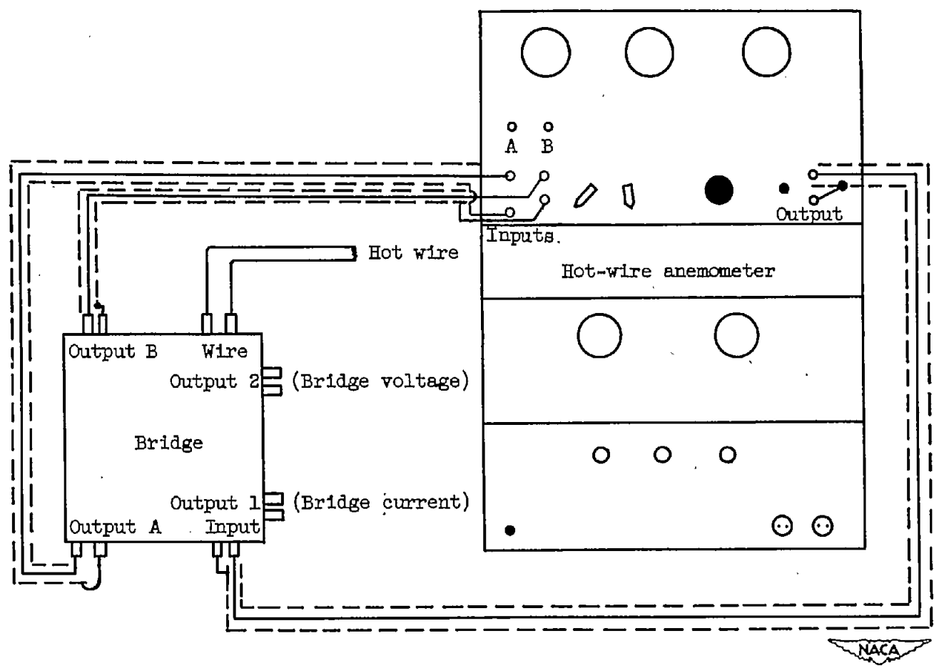
Figure 29. - Hot-wire anemometer to bridge connections.
