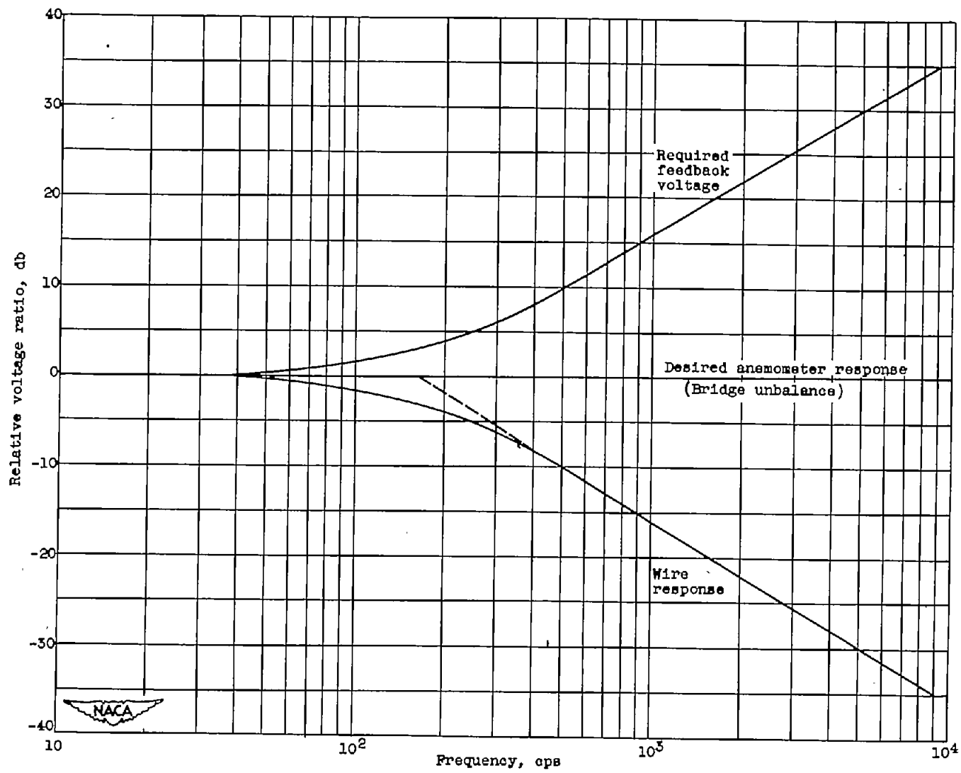
Figure 4. - Theoretical frequency response.
