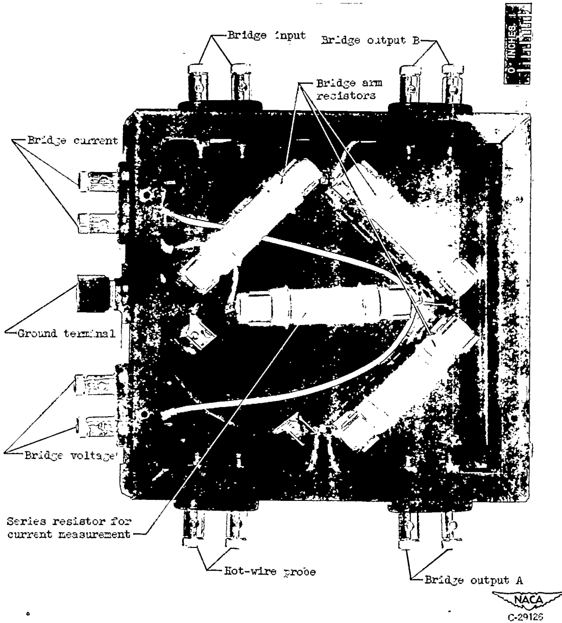
Figure 5. - Hot-wire bridge.
