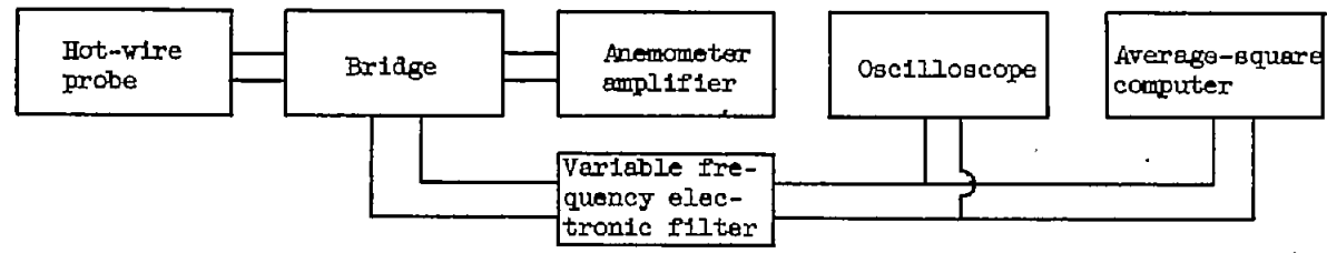
(e) Spectrum of turbulence measurements (method 1).
