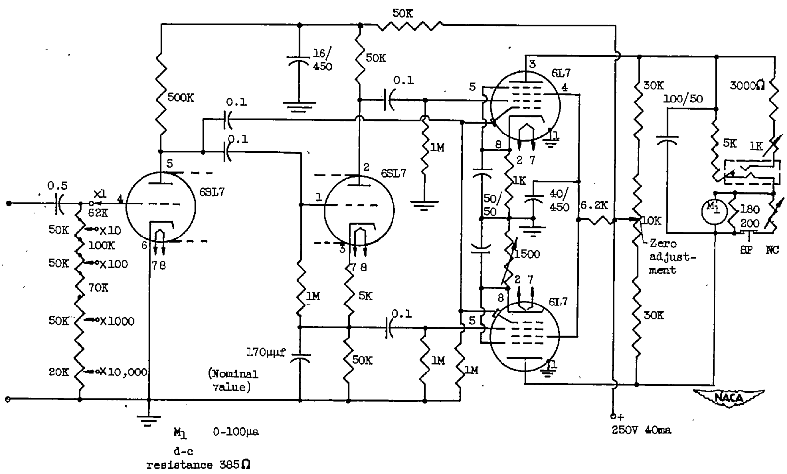
Figure 10. - Average-square computer circuit.
