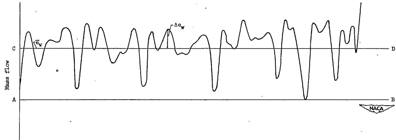
(b) Trace of oscillogram, showing method of locating mean flow line.
