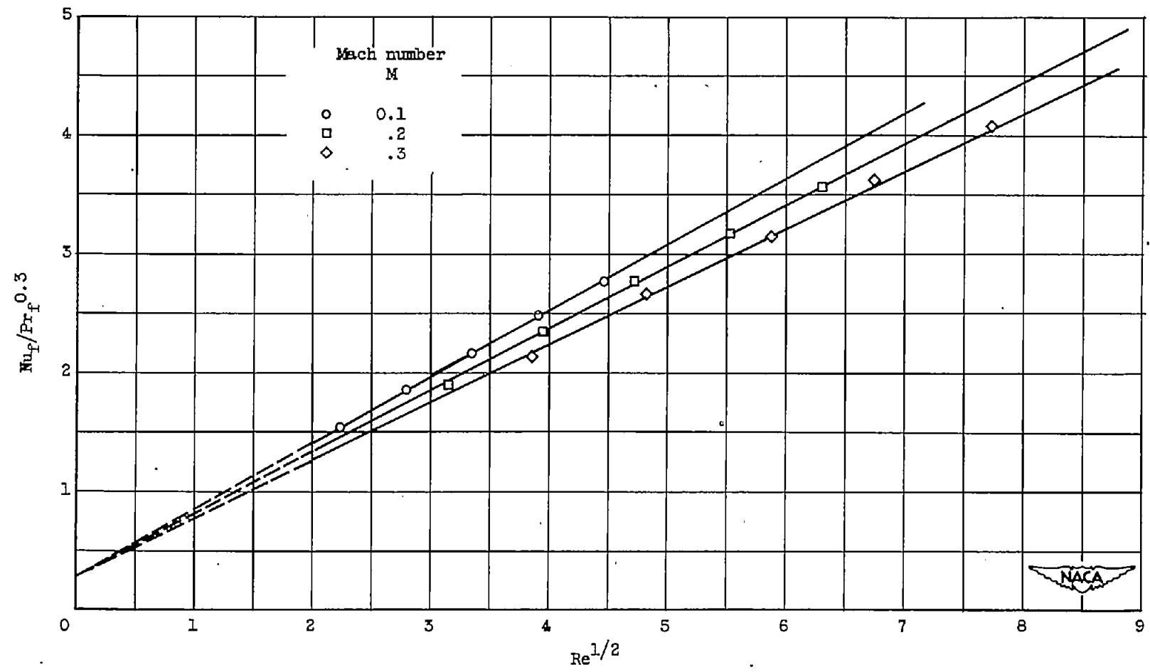
(b) Wire temperature, 343° F.
