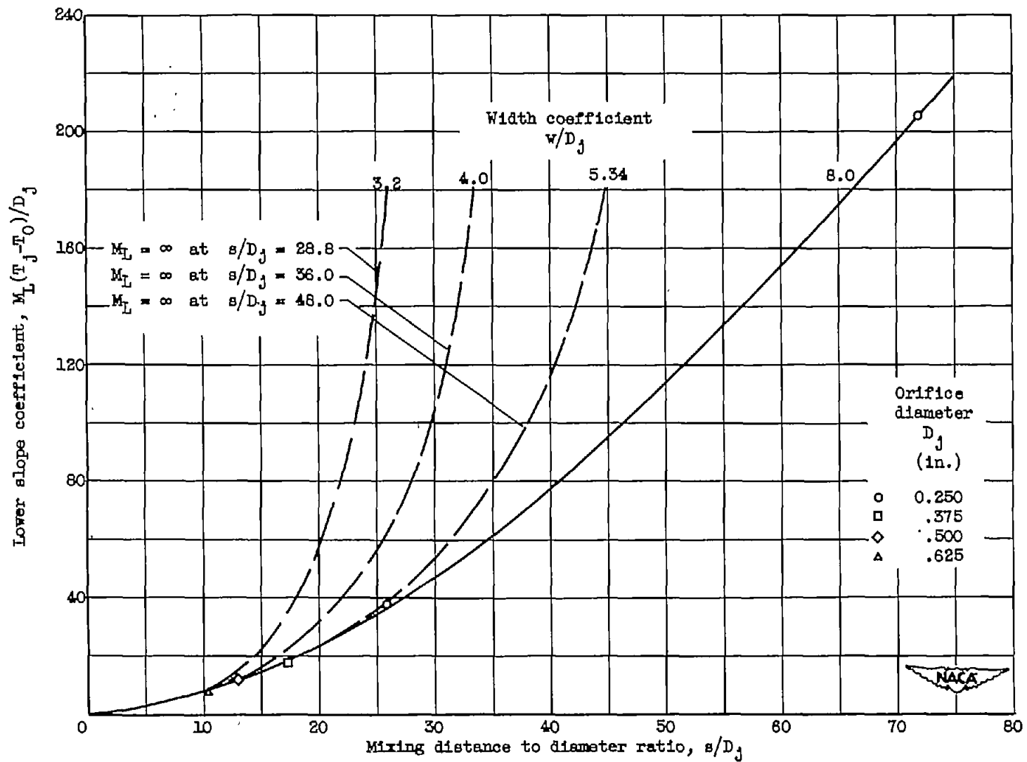
Figure 24. - Variation of lower slope coefficient with mixing distance to diameter ratio for constant values of width coefficient. Jet angle, 30^\circ .
