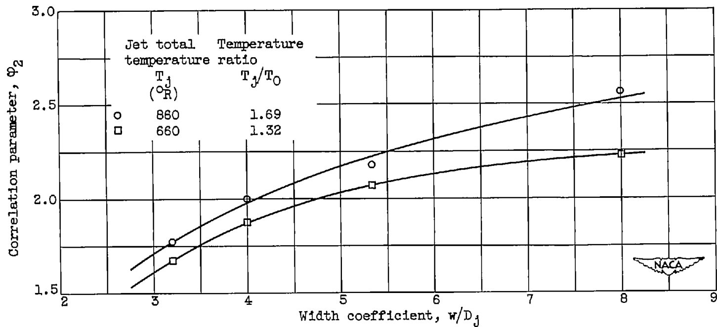
Figure 6. - Variation of correlation parameter \phi_2 with width coefficient for constant values of temperature ratio. Jet angle, 60^{\circ} .
