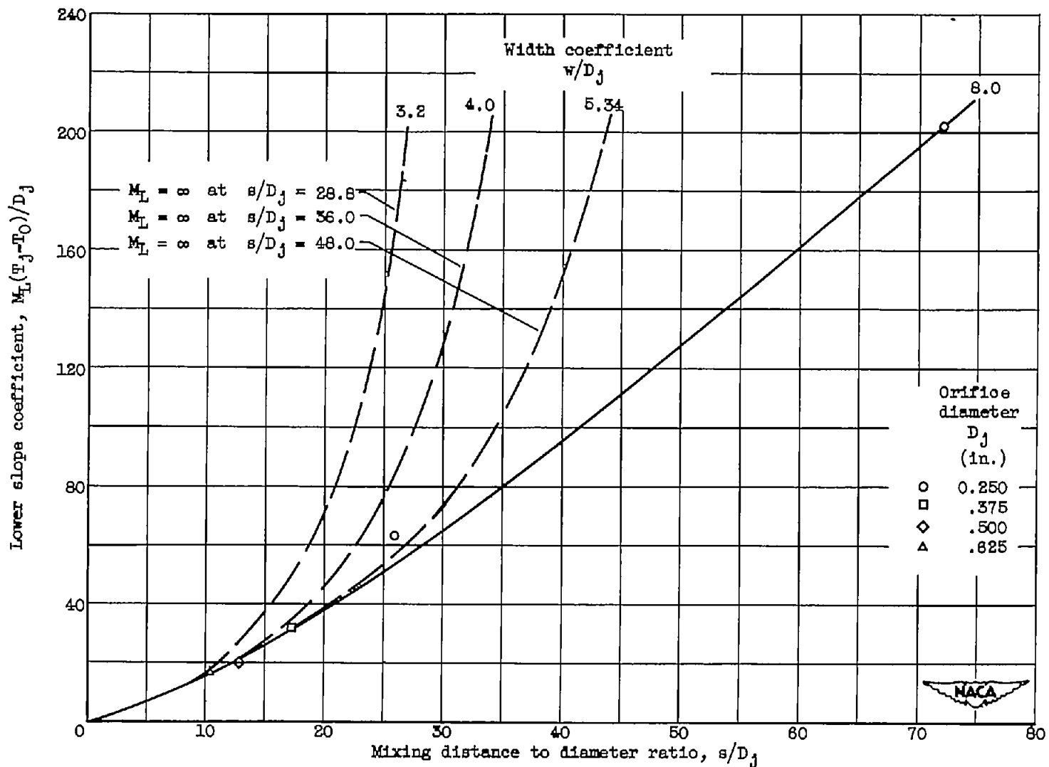
Figure 23. - Variation of lower slope coefficient with mixing distance to diameter ratio for constant values of width coefficient. Jet angle, 45°.
