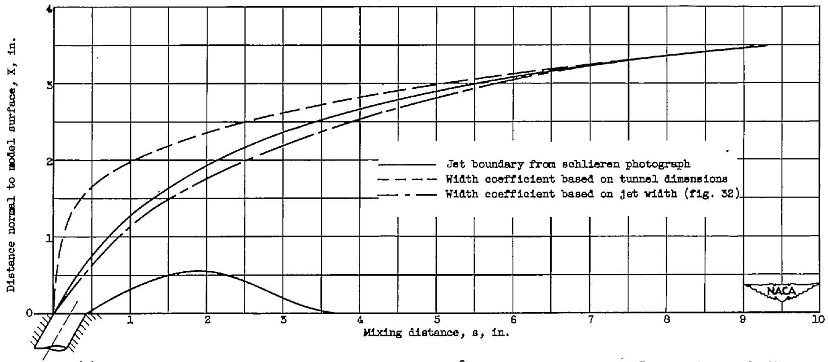
(b) Orifice diameter, 0.375 inch; jet total temperature, 880^{\circ} R; jet pressure ratio, 3.15; free-stream velocity, 395 feet per second; jet angle, 60^{\circ} .
