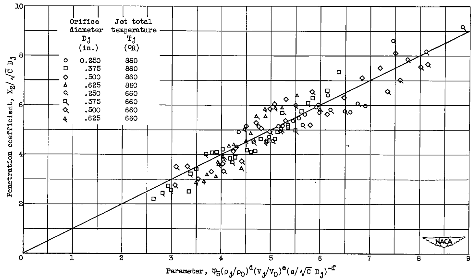
Figure 11. - Variation of penetration coefficient X_2/\sqrt{C} D_j with parameter \phi_5(\rho_j/\rho_0)^d (v_j/v_0)^e (s/\sqrt{C} D_j)^{-f} for various jet total temperatures. Jet angle, 90^\circ .
