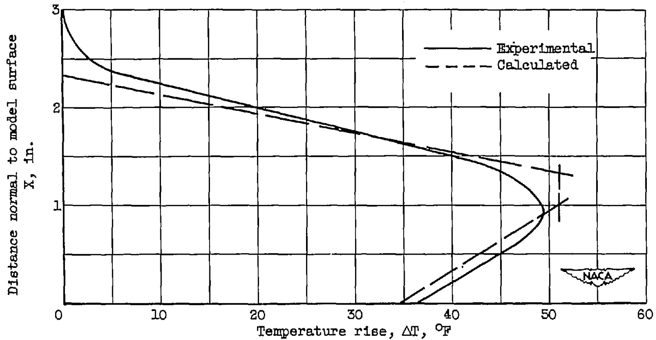
Figure 31. - Comparison of calculated and experimental temperature profiles for jet operating at pressure ratio below choking. Jet pressure ratio, 1.36; orifice diameter, 0.625 inch; jet total temperature, 840° R; free-stream velocity, 400 feet per second; rake position, 6.47 inches; jet angle, 90°.
