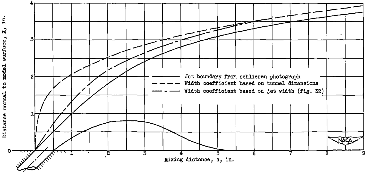
(c) Orifice diameter, 0.375 inch; jet total temperature, 860^{\circ} R; jet pressure ratio, 2.86; free-stream velocity, 232 feet per second; jet angle, 45^{\circ} .
