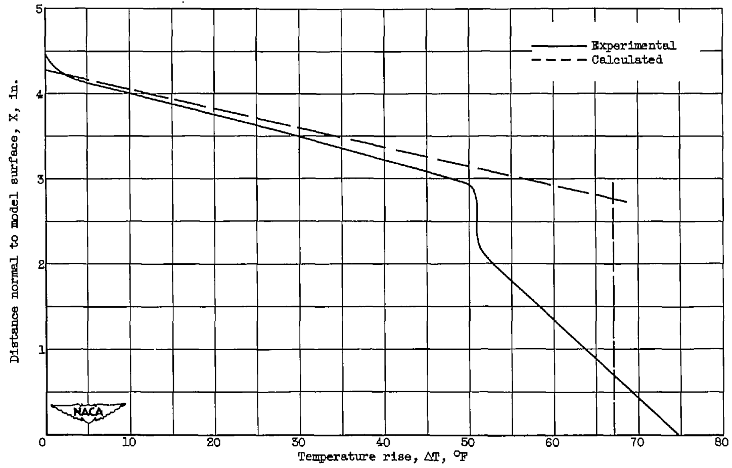
(c) Orifice diameter, 0.625 inch; jet total temperature, 860° R; jet pressure ratio, 2.53; free-stream velocity, 235 feet per second; rake position, 6.47 inches; jet angle, 60°.
