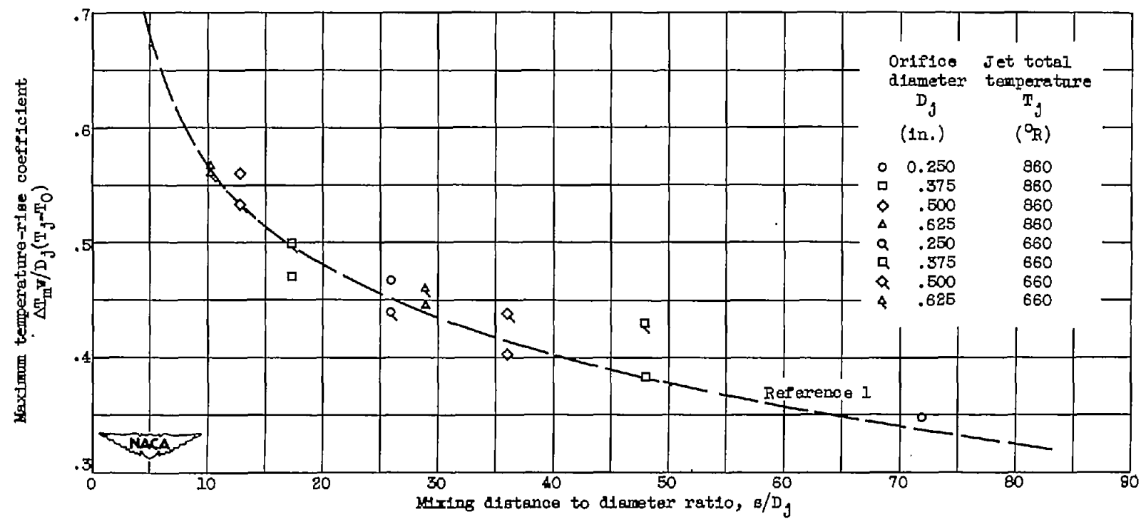
Figure 25. - Variation of maximum temperature-rise coefficient \Delta T_{m,w}/D_j(T_j - T_0) with mixing distance to diameter ratio. Jet angle, 90^{\circ} .
