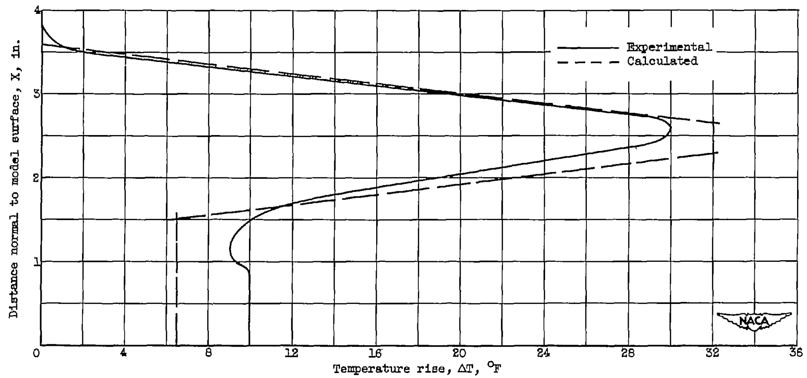
(d) Orifice diameter, 0.375 inch; jet total temperature, 860° R; jet pressure ratio, 3.02; free-stream velocity, 235 feet per second; rake position, 6.47 inches; jet angle, 45°.
