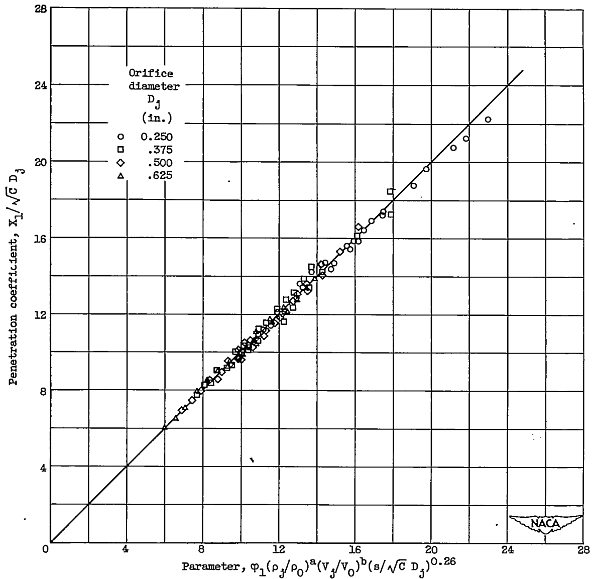
Figure 3. - Variation of penetration coefficient X_1/\sqrt{C} D_j with parameter \phi_1(\rho_j/\rho_0)^a (v_j/v_0)^b (s/\sqrt{C} D_j)^{0.26} . Jet angle, 90^\circ .
