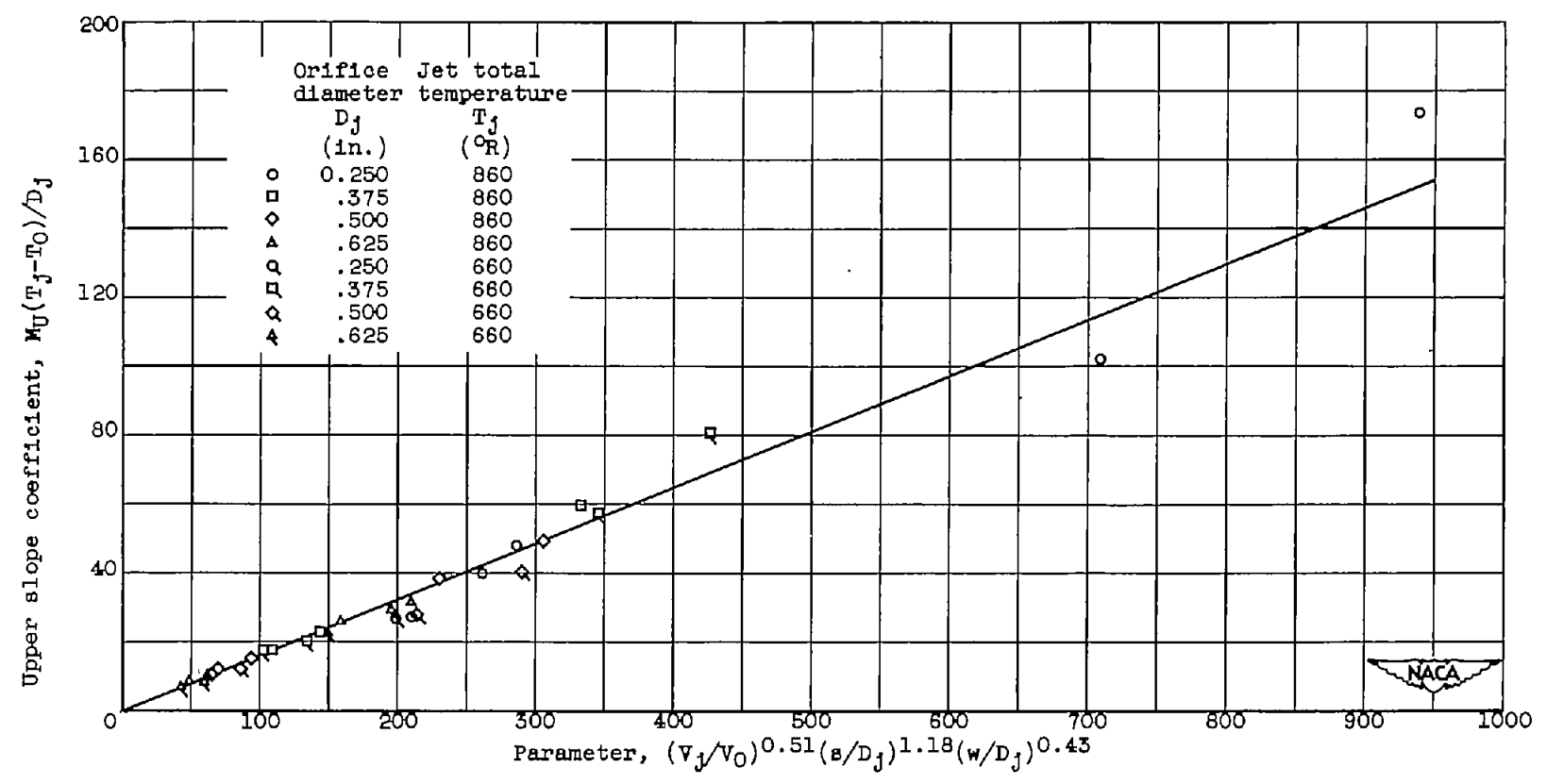
Figure 19. - Variation of upper slope coefficient with parameter (V_j/V_0)^{0.51} (s/D_j)^{1.18} (w/D_j)^{0.43} . Jet angle, 45°.
