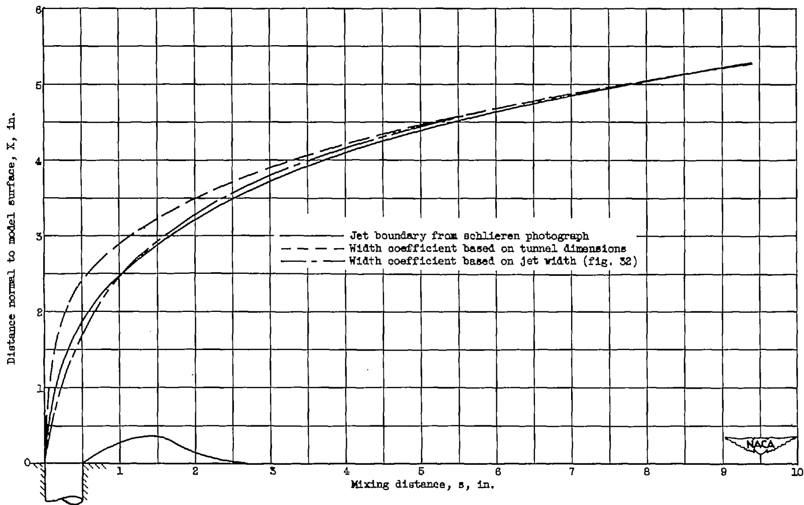
(a) Orifice diameter, 0.500 inch; jet total temperature, 860^{\circ} R; jet pressure ratio, 3.33; free-stream velocity, 375 feet per second; jet angle, 90^{\circ} .
