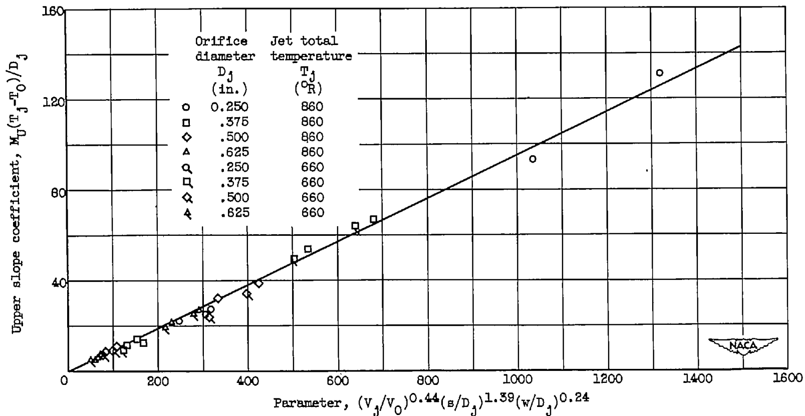
Figure 20. - Variation of upper slope coefficient with parameter (V_j/V_0)^{0.44} (s/D_j)^{1.39} (w/D_j)^{0.24} . Jet angle, 30^{\circ} .
