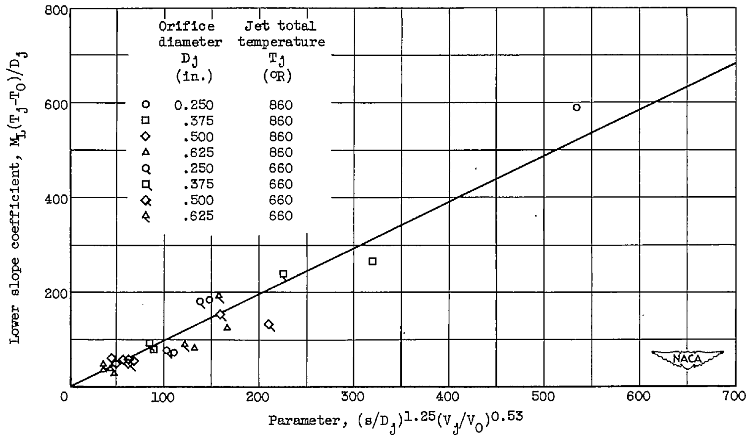
Figure 21. - Variation of lower slope coefficient with parameter (s/D_j)^{1.25}(v_j/v_0)^{0.53} for various jet total temperatures. Jet angle, 90^\circ .
