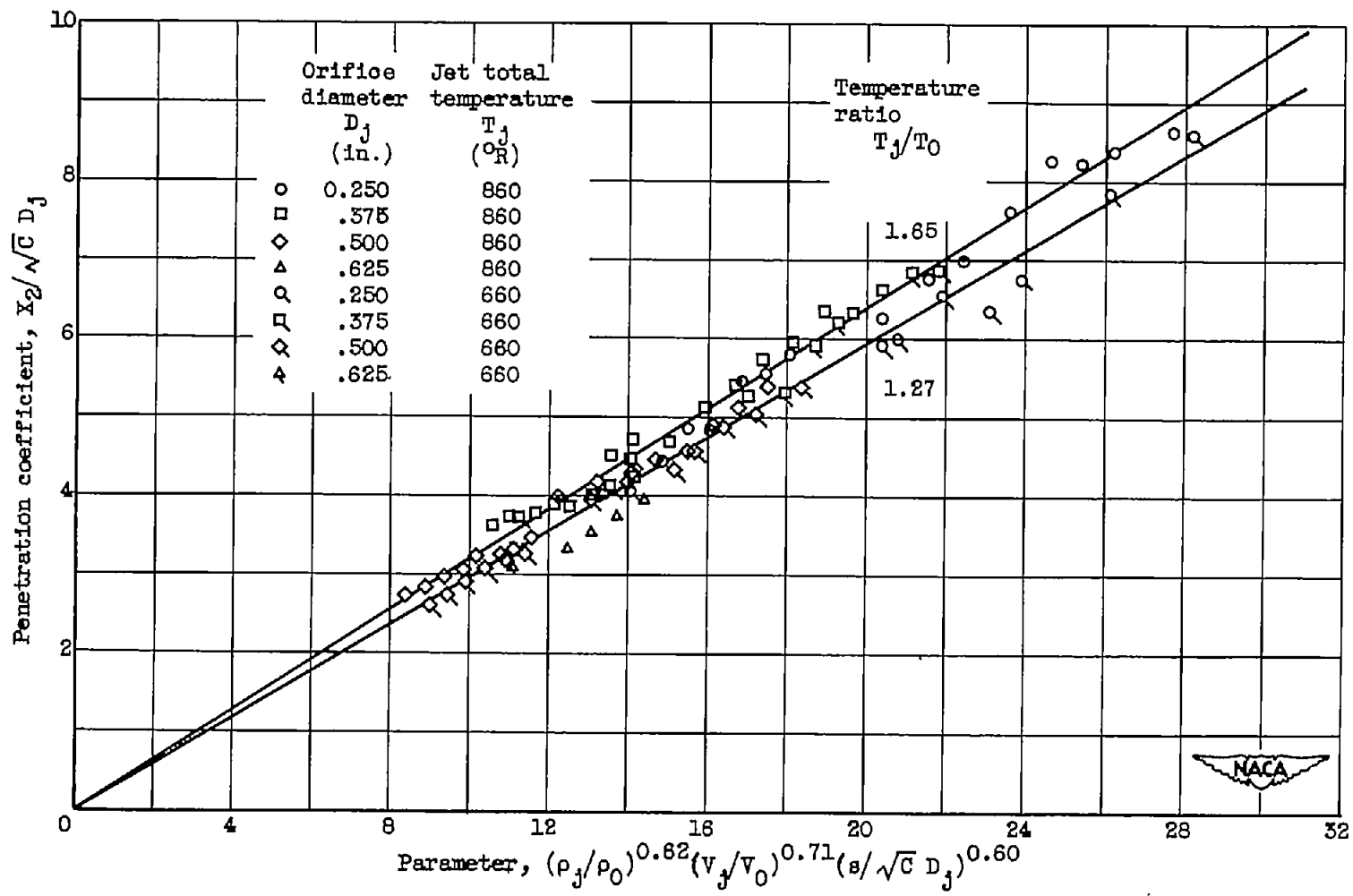
Figure 15. - Variation of penetration coefficient X_2/\sqrt{C} D_j with parameter (\rho_j/\rho_0)^{0.62}(v_j/v_0)^{0.71}(s/\sqrt{C} D_j)^{0.60} for constant values of temperature ratio. Jet angle, 45^{\circ} .
