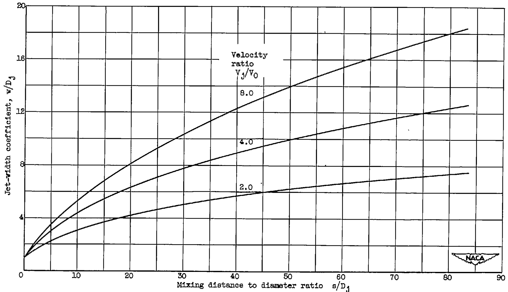
Figure 32. - Variation of jet-width coefficient w/D_j with mixing distance to diameter ratio for three velocity ratios.
