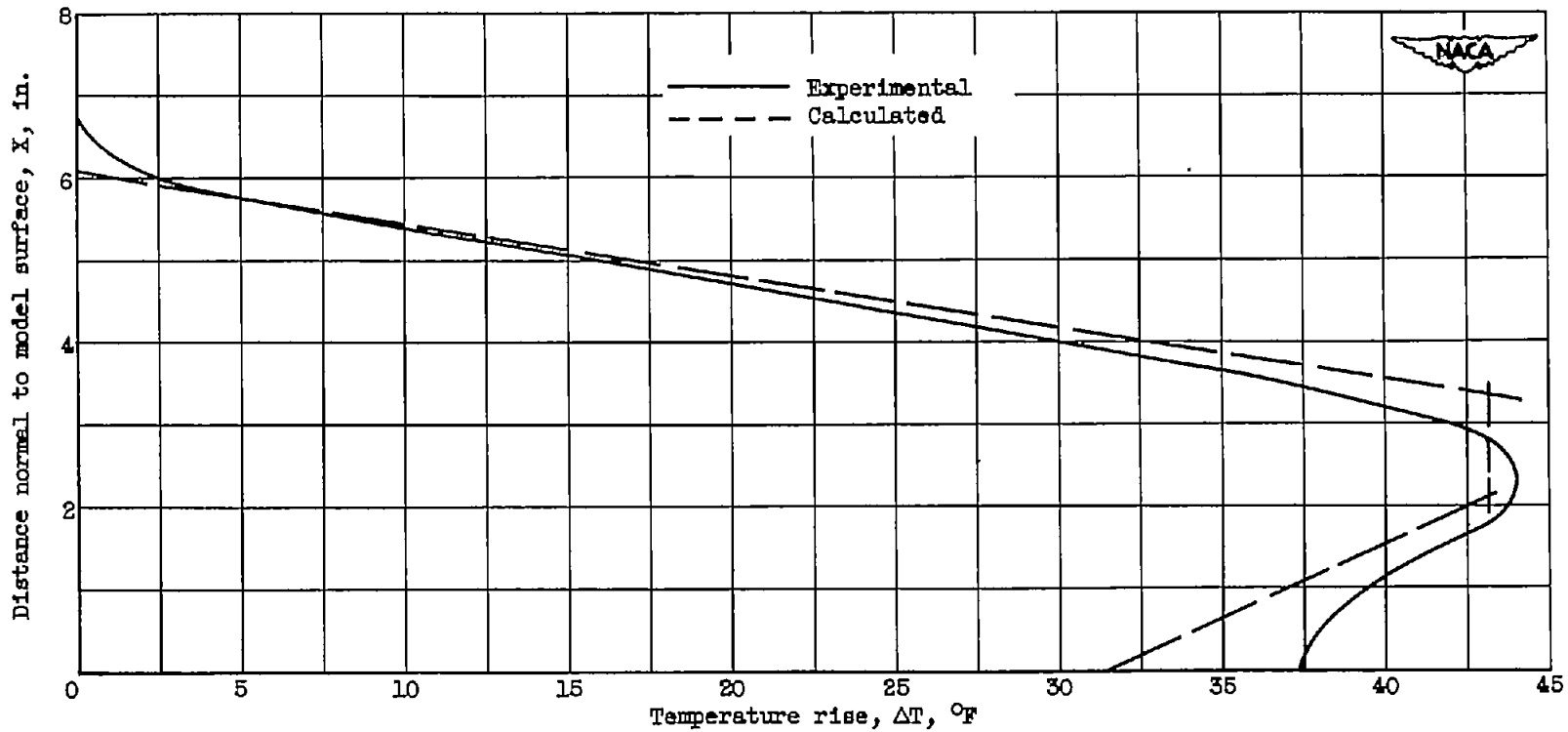
(a) Orifice diameter, 0.625 inch; jet total temperature, 880° R; jet pressure ratio, 2.38; free-stream velocity, 380 feet per second; rake position, 18.0 inches; jet angle, 90°.
