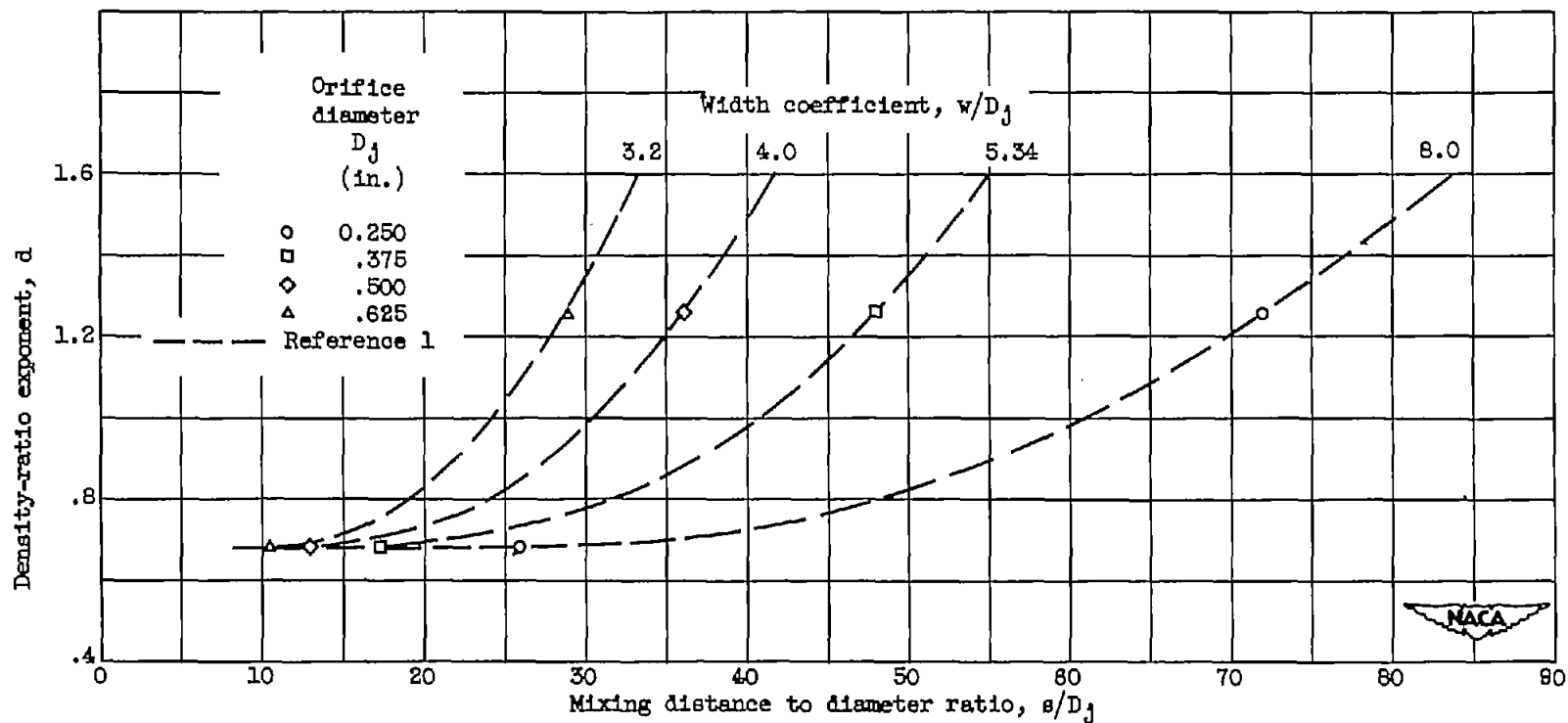
Figure 12. - Variation of density-ratio exponent d with mixing distance to diameter ratio for constant values of width coefficient. Jet angle, 60^\circ .
