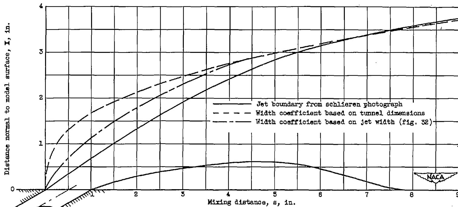
(d) Orifice diameter, 0.500 inch; jet total temperature, 660° R; jet pressure ratio, 2.93; free-stream velocity, 235 feet per second; jet angle, 30°.
