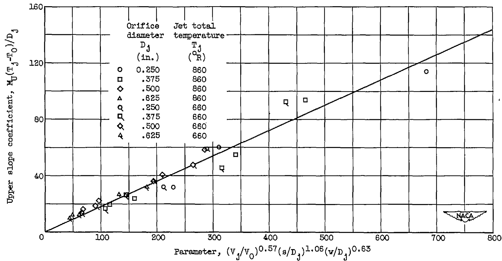
Figure 18. - Variation of upper slope coefficient with parameter (V_j/V_0)^{0.57}(s/D_j)^{1.06}(w/D_j)^{0.63} . Jet angle, 60^{\circ} .
