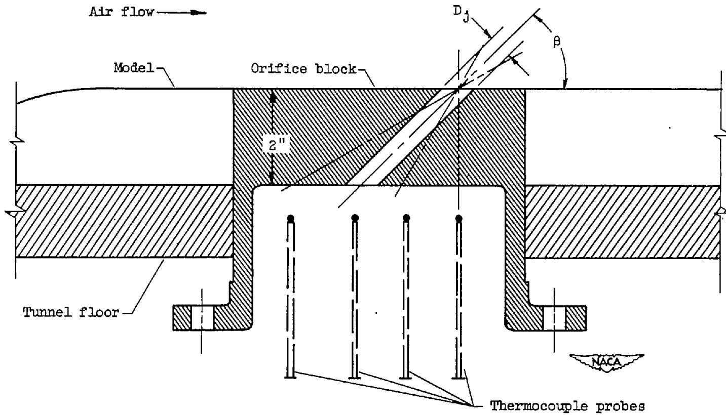
(b) Orifice mounted in plane parallel to air stream.
