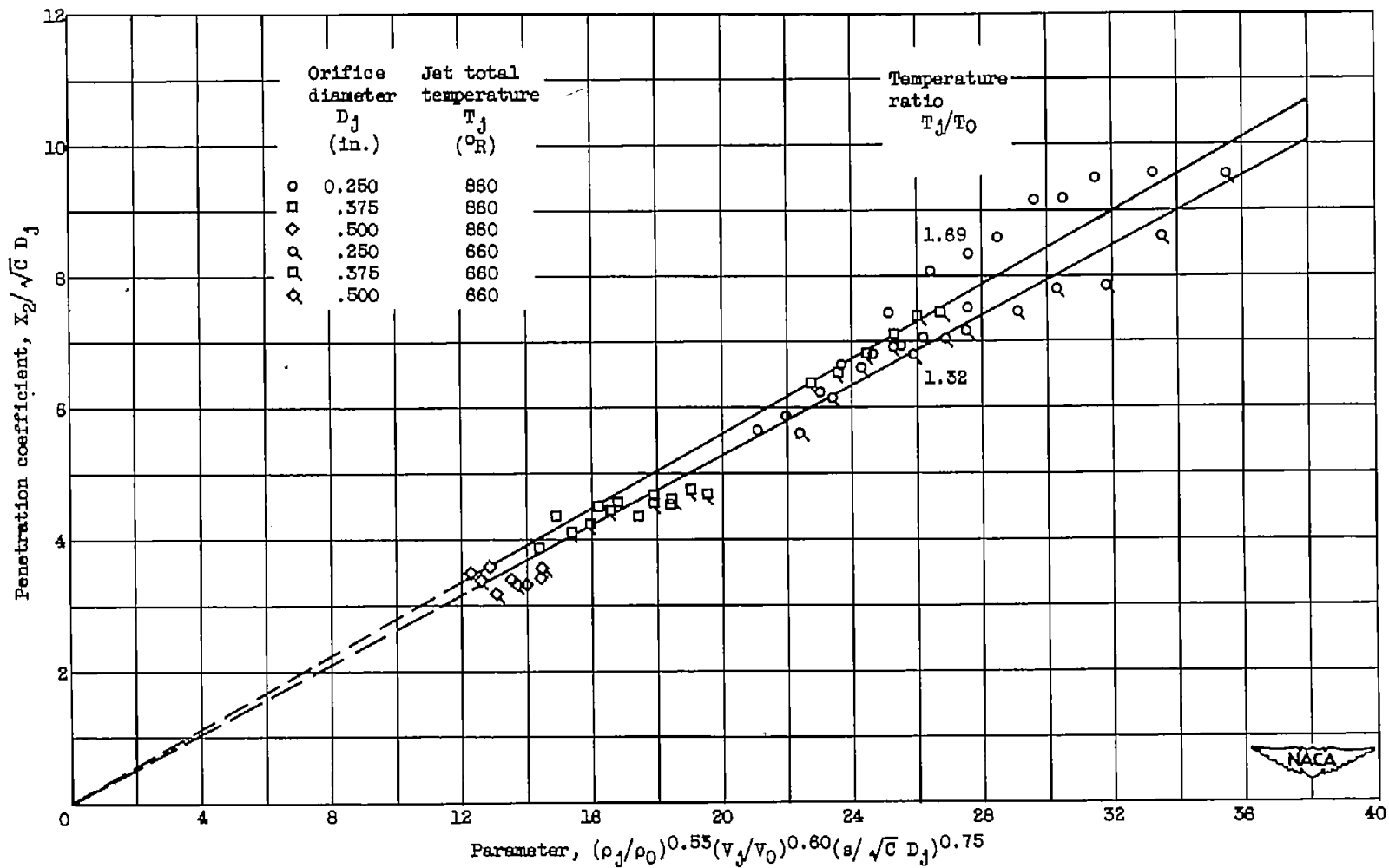
Figure 14. - Variation of penetration coefficient X_2/\sqrt{C} D_j with parameter (\rho_j/\rho_0)^{0.53}(v_j/v_0)^{0.60}(s/\sqrt{C} D_j)^{0.75} for constant values of temperature ratio. Jet angle, 60°.
