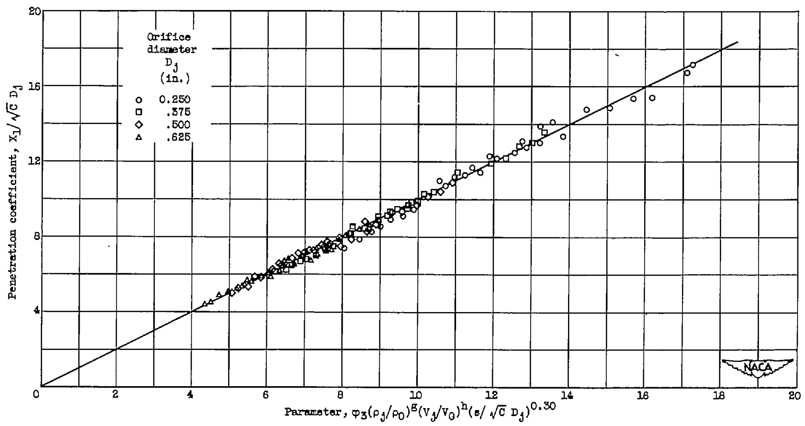
Figure 7. - Variation of penetration coefficient X_1/\sqrt{C} D_j with parameter \phi_3(\rho_j/\rho_0)^B(V_j/V_0)^h(\epsilon/\sqrt{C} D_j)^{0.30} . Jet angle, 45^\circ .
