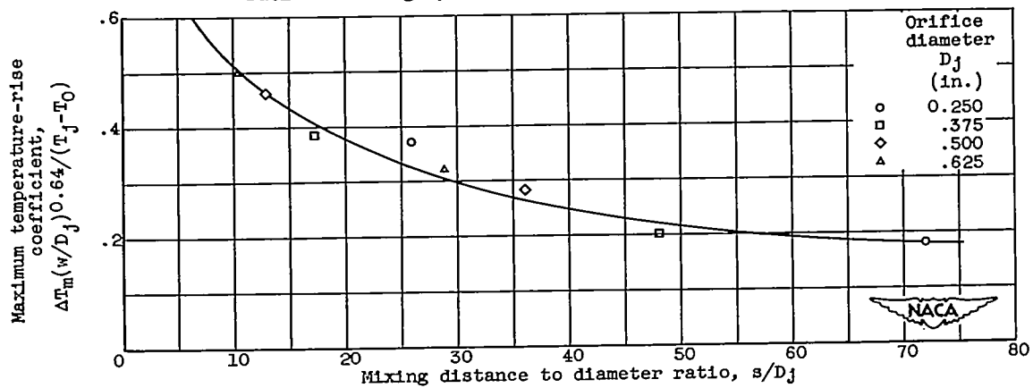
Figure 28. - Variation of maximum temperature-rise coefficient \Delta T_m(w/D_j)^{0.64}/(T_j-T_0) with mixing distance to diameter ratio. Jet angle, 30^\circ .
