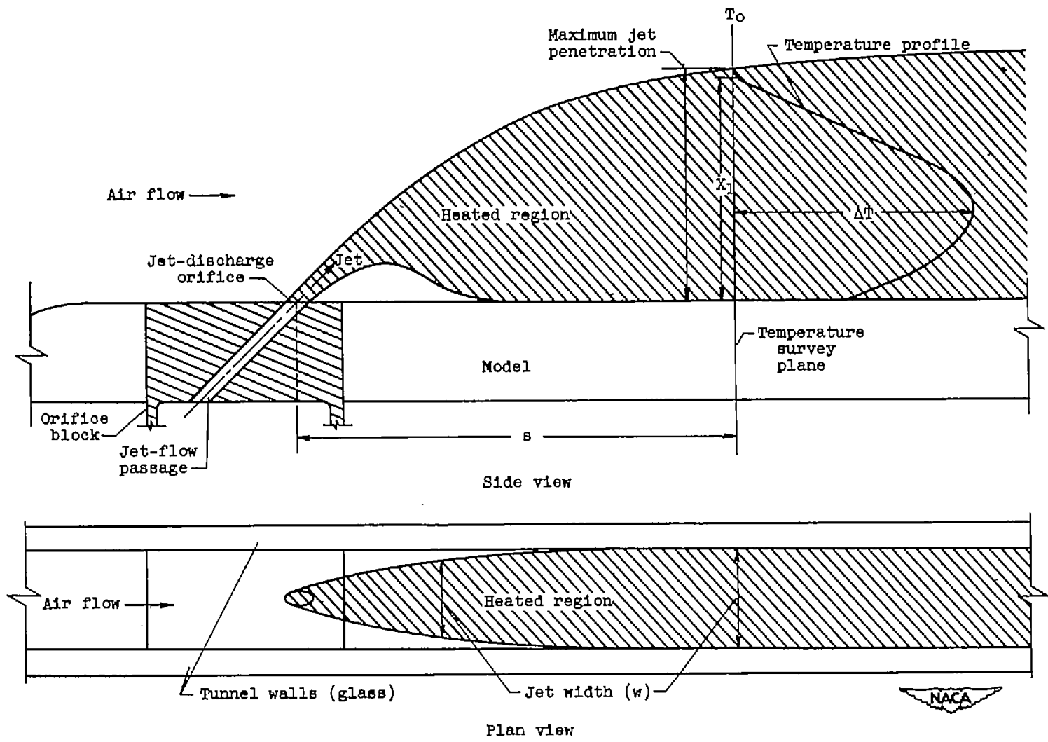
(c) Nomenclature and typical temperature profile produced by jet discharging at angle to air stream.
