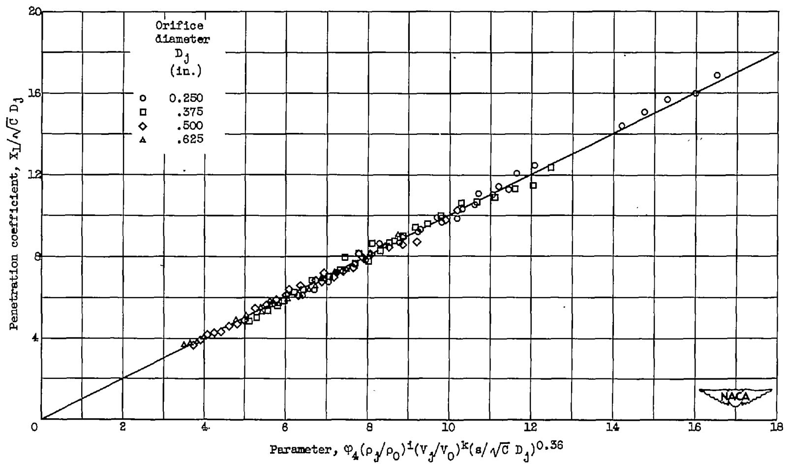
Figure 9. - Variation of penetration coefficient X_1/\sqrt{C} D_j with parameter \varphi_4(\rho_j/\rho_0)^1(v_j/v_0)^k(s/\sqrt{C} D_j)^{0.36} . Jet angle, 30^\circ .
