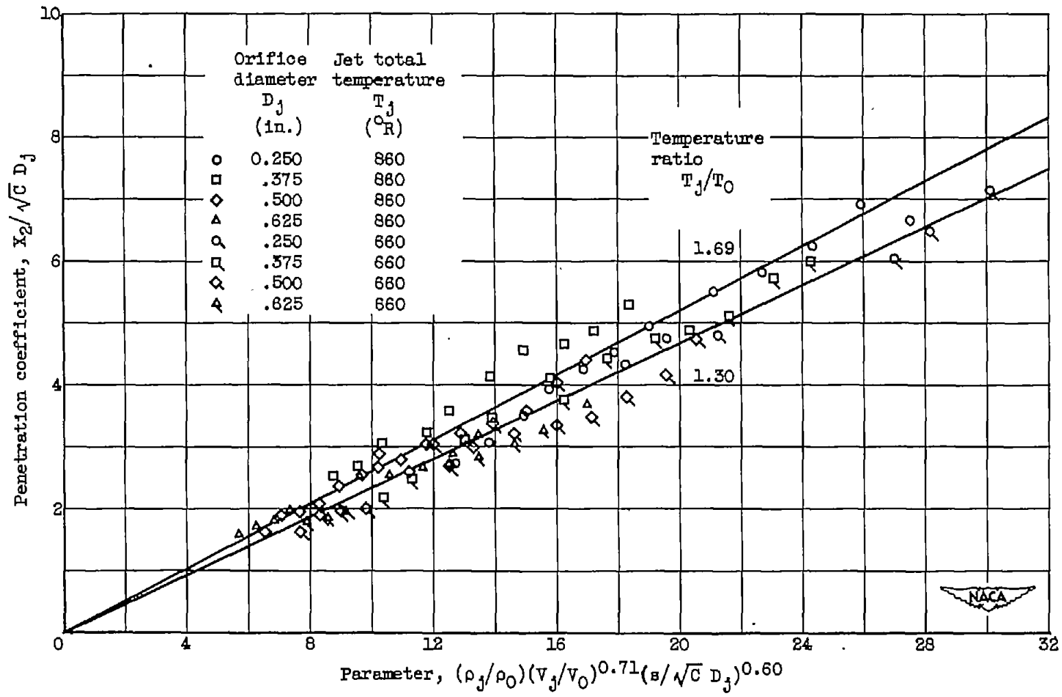
Figure 16. - Variation of penetration coefficient X_2/\sqrt{C} D_j with parameter (\rho_j/\rho_0)(v_j/v_0)^{0.71}(s/\sqrt{C} D_j)^{0.60} for constant values of temperature ratio. Jet angle, 30°.
