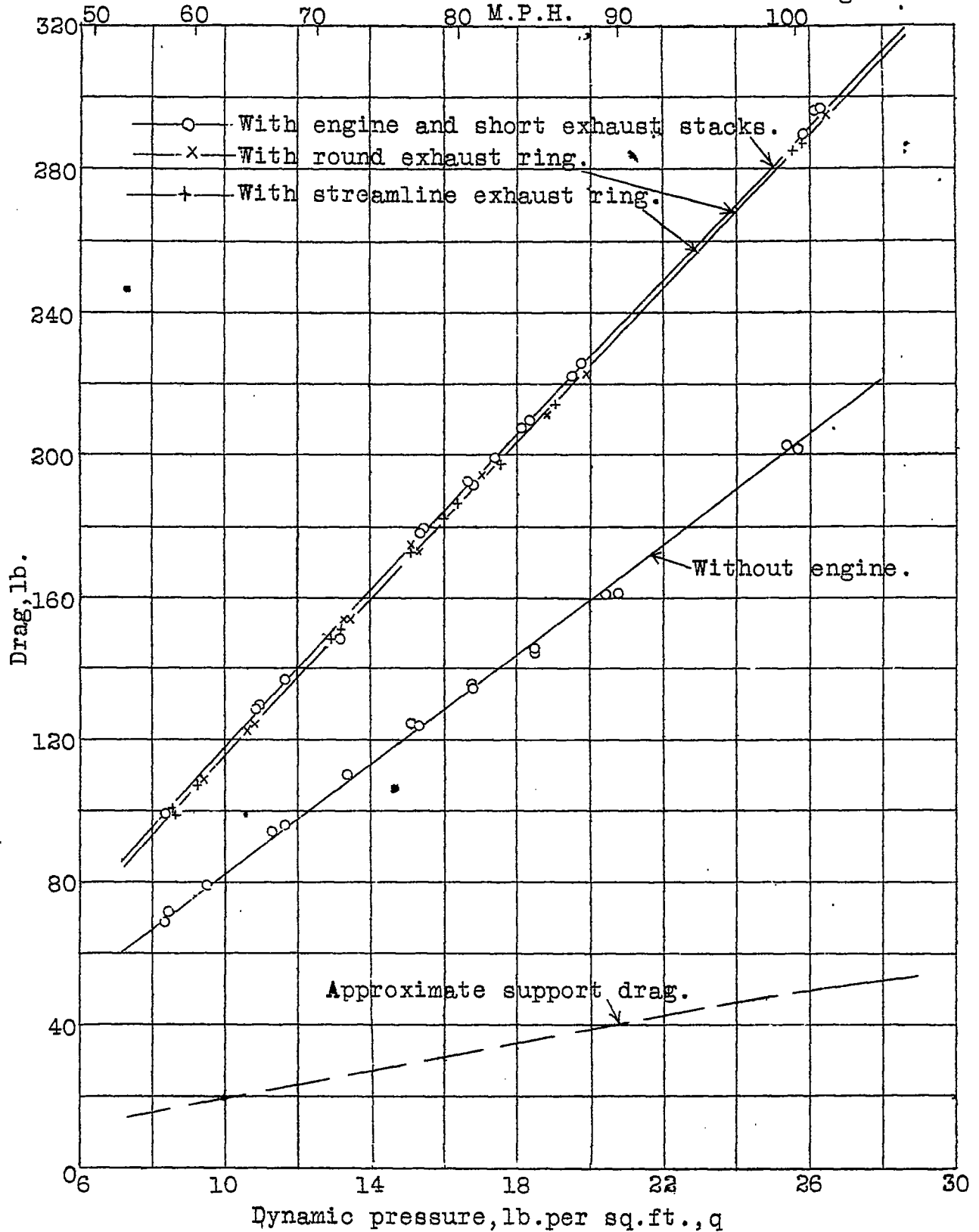
Fig. 5 Observed drag.
