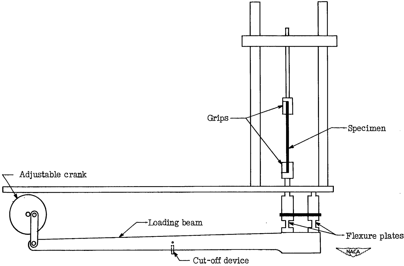
Figure 3.- Schematic drawing of fatigue testing machine used by Battelle.
