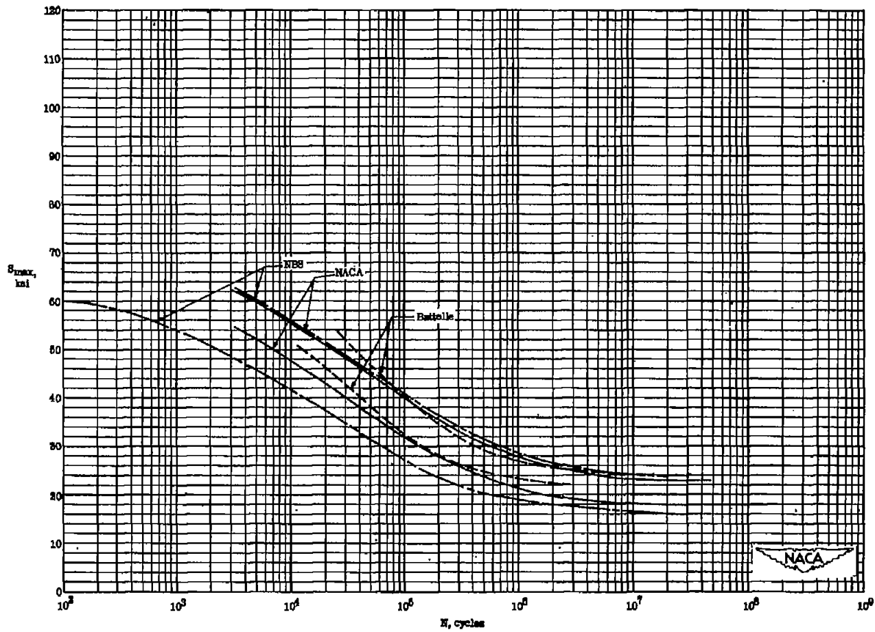
Figure 26.- Comparison of results of fatigue tests at R = -1.00 on unnotched 24S-T3 aluminum-alloy sheet specimens tested by Battelle, NACA, and NBS.
