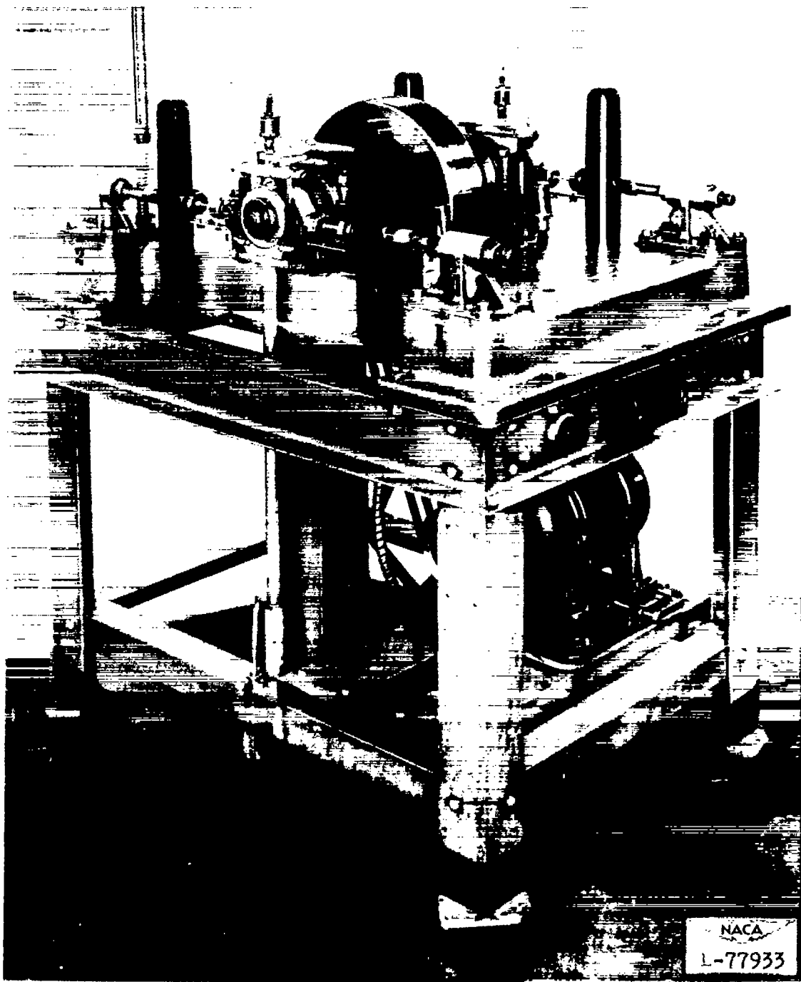
Figure 18.- Axial-stress fatigue testing machine used by ALCOA.
