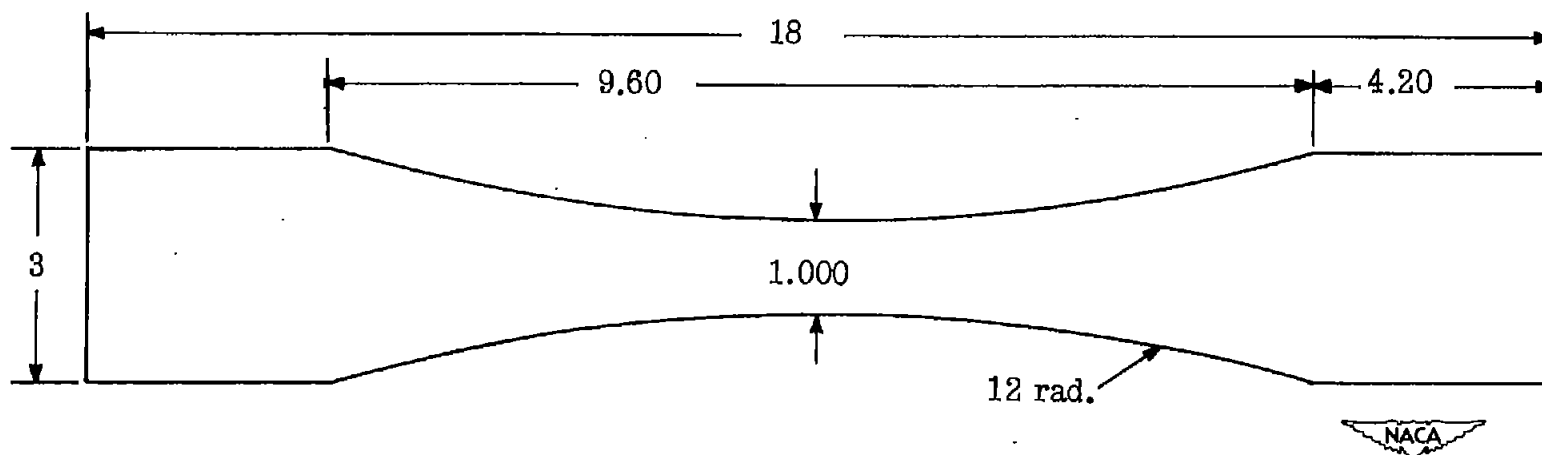
Figure 1.- Fatigue test specimen tested by Battelle and NACA. All dimensions are in inches.
