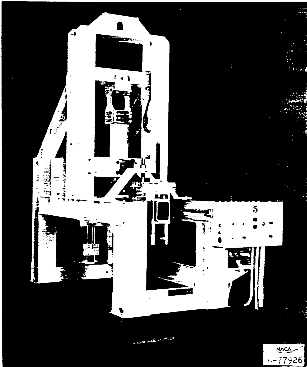
Figure 7.- Axial-load fatigue testing machine used by NACA.
