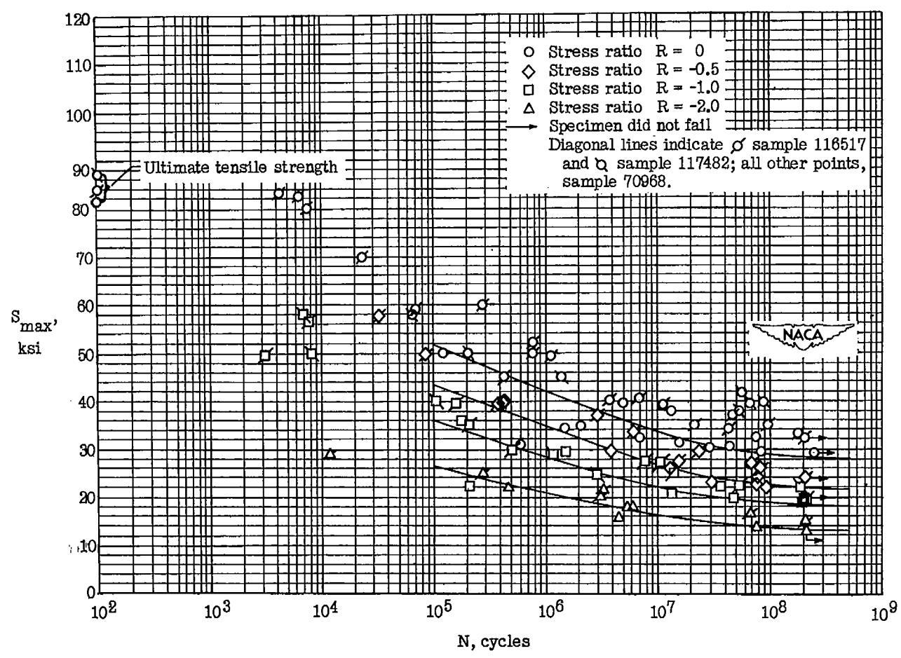
Figure 20.- Results of fatigue tests on unnotched 75S-T6 aluminum-alloy rolled and drawn rod specimens tested by ALCOA.
