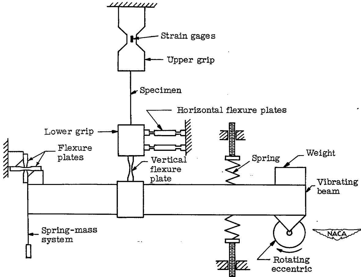
Figure 8.- Schematic drawing of fatigue testing machine used by NACA.
