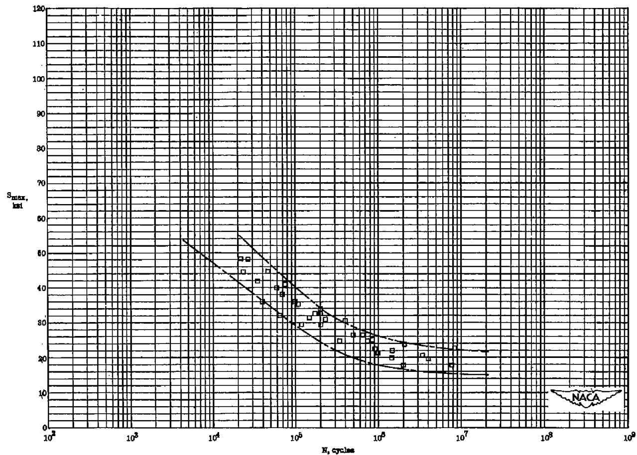
Figure 27.- Results of fatigue tests at R = -1.00 on unnotched 75S-T6 aluminum-alloy sheet specimens tested by NBS (data from ref. 12).
