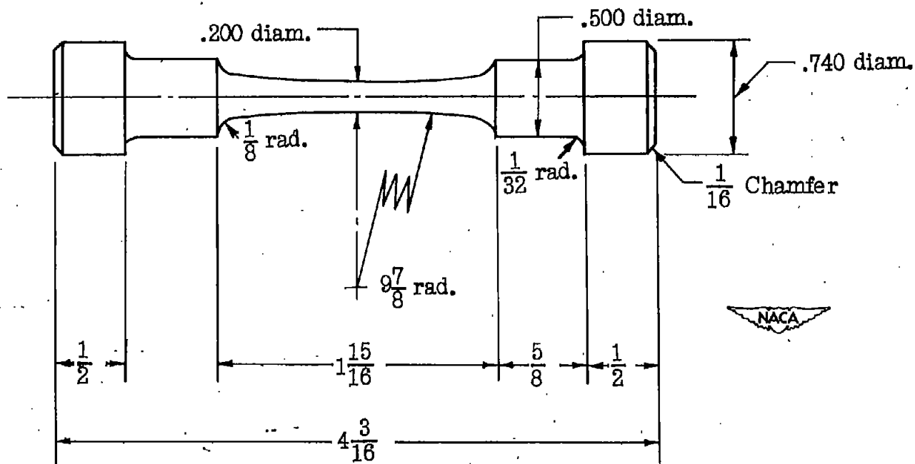
Figure 17.- Fatigue test specimen tested by ALCOA. All dimensions are in inches.
