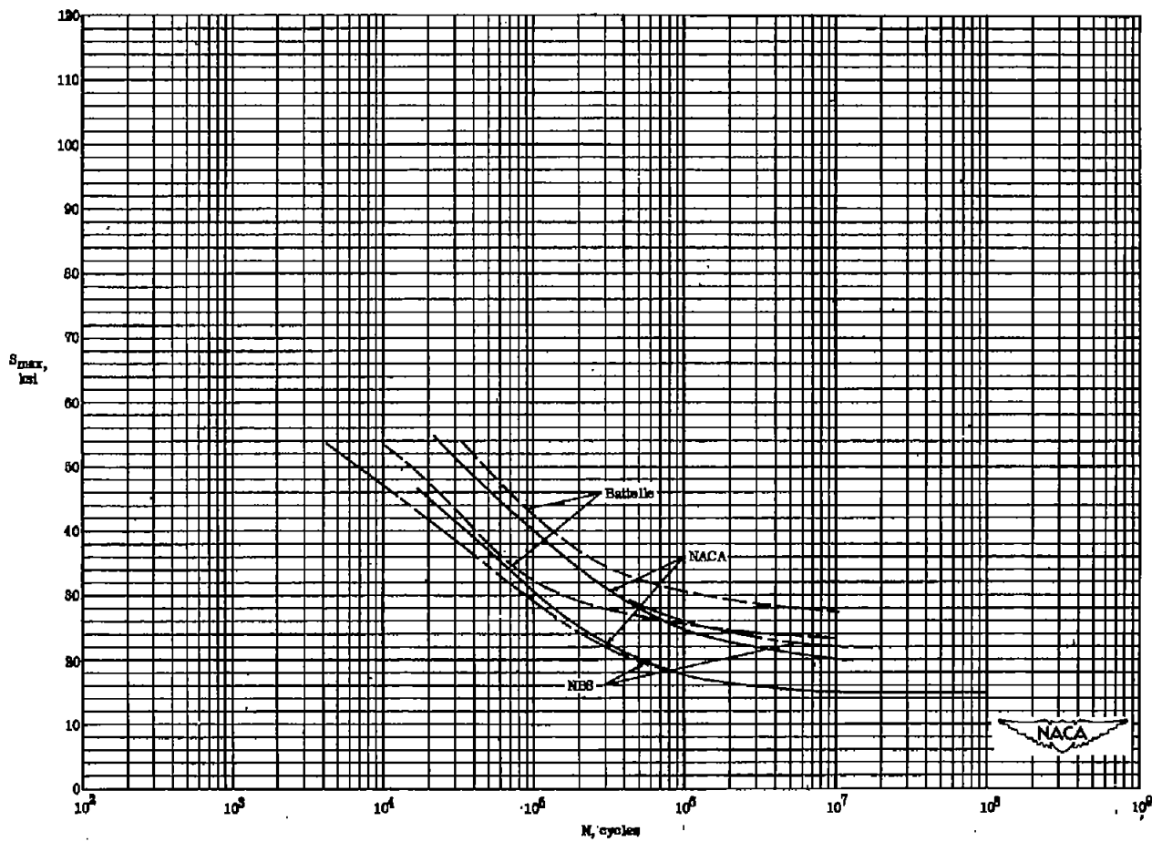
Figure 28.- Comparison of results of fatigue tests at R = -1.00 on unnotched 75S-T6 aluminum-alloy sheet specimens tested by Battelle, NACA, and NBS.
