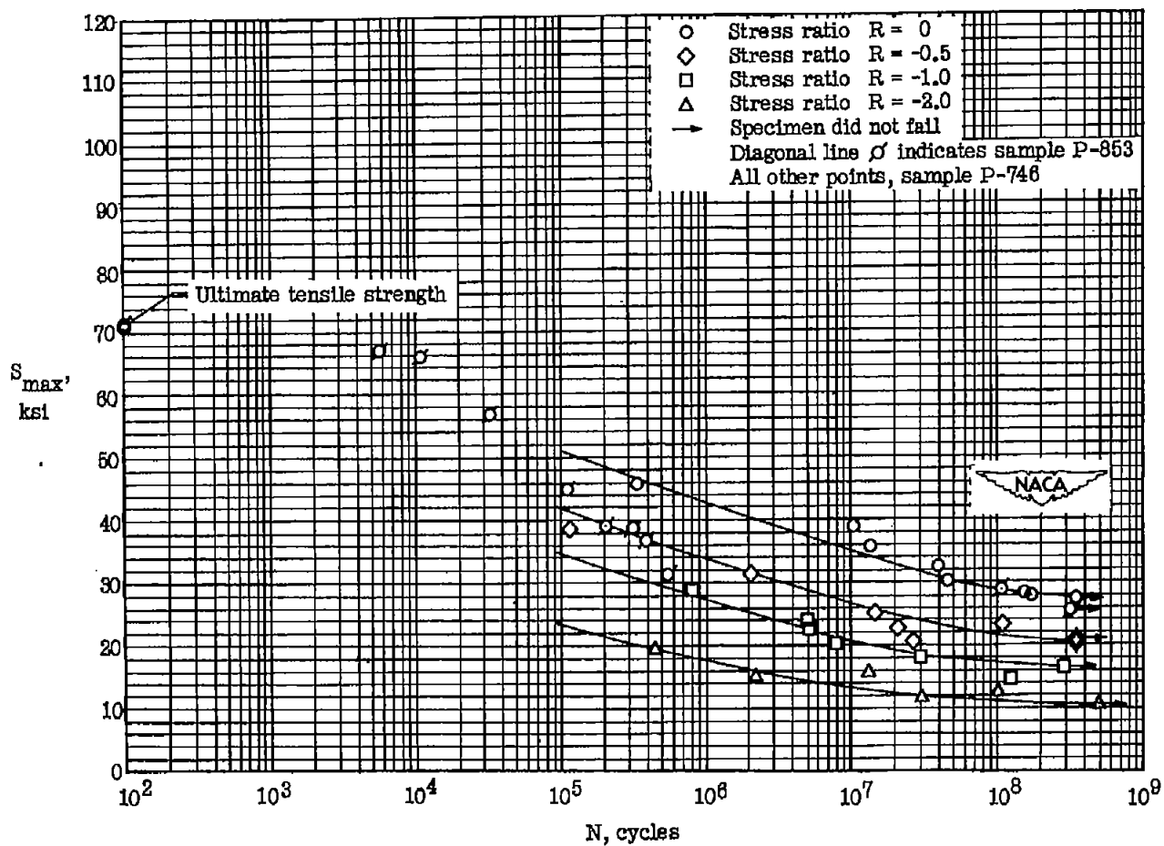
Figure 19.- Results of fatigue tests on unnotched 24S-T4 aluminum-alloy rolled and drawn rod specimens tested by ALCOA.
