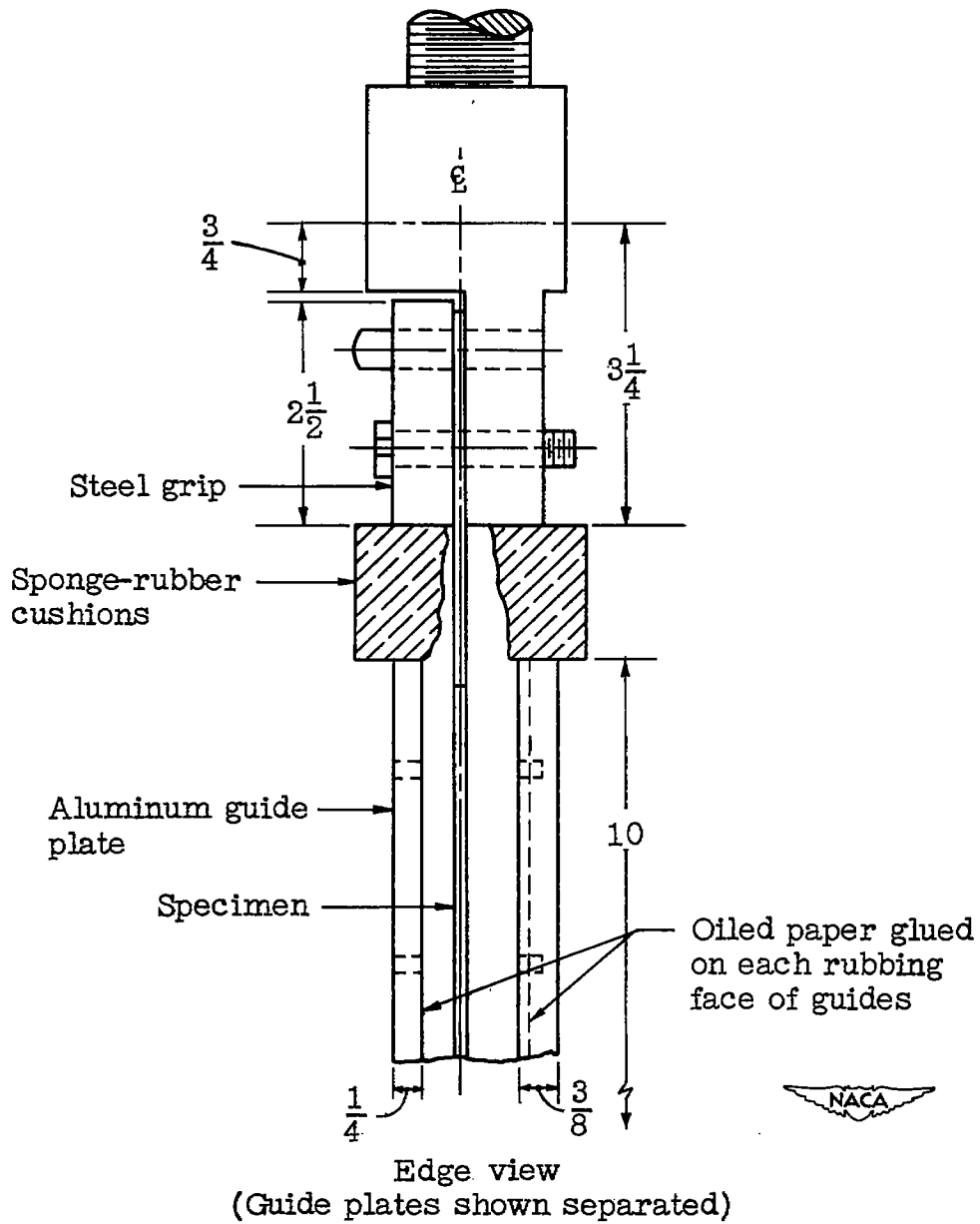
Figure 4.- Sketch of tension-compression grips and guide plates. Only upper portion shown. All dimensions are in inches.
