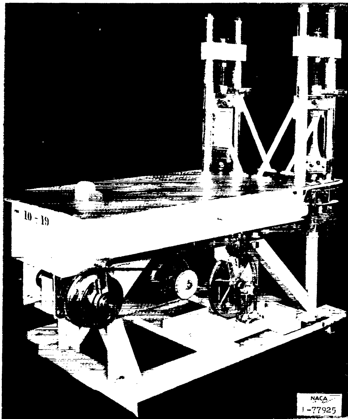
Figure 2.- Krouse direct repeated-stress testing machine.
