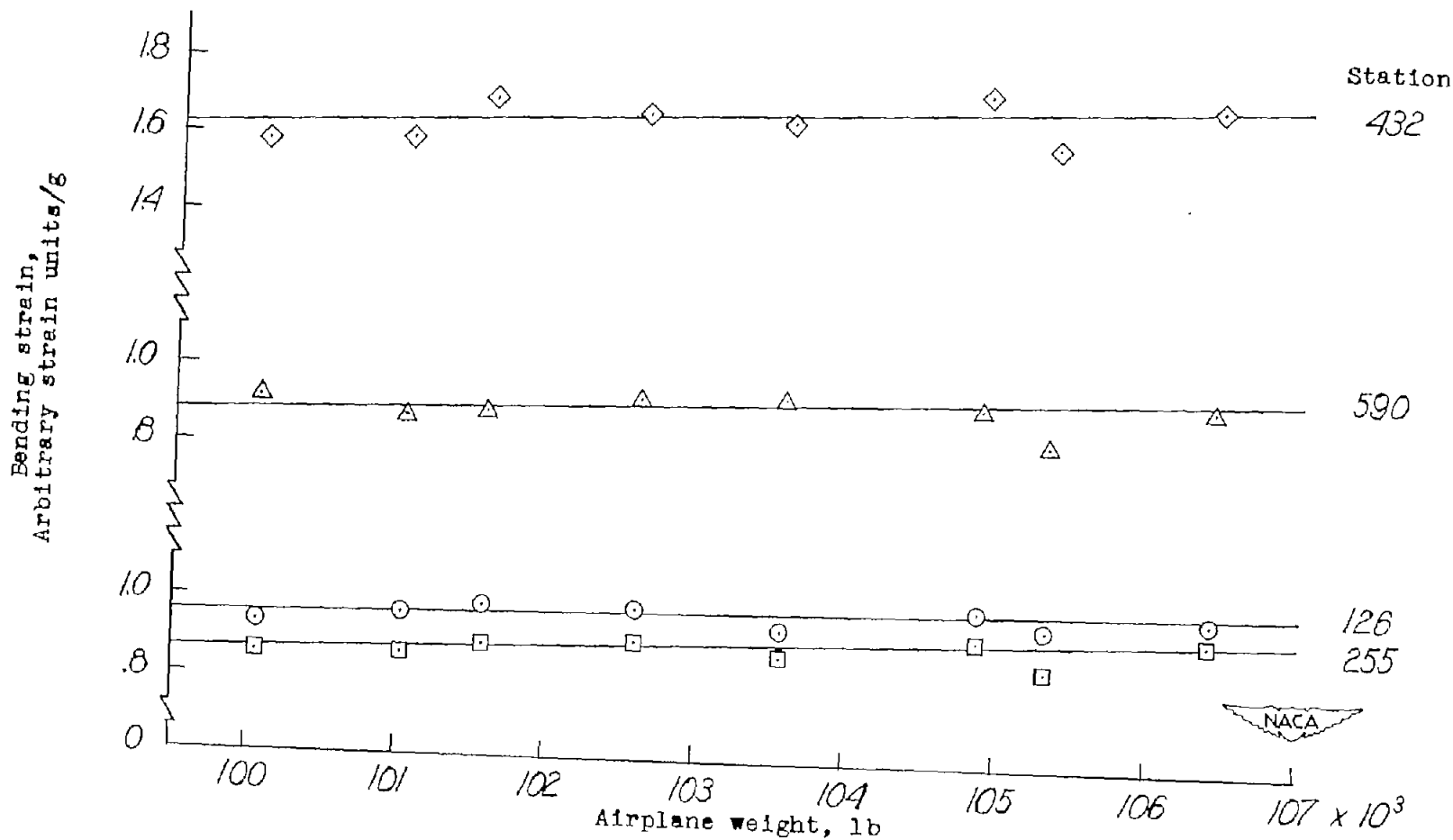
Figure 6.- Variation of bending strains in pull-ups with airplane weight. Left wing; front spar.
