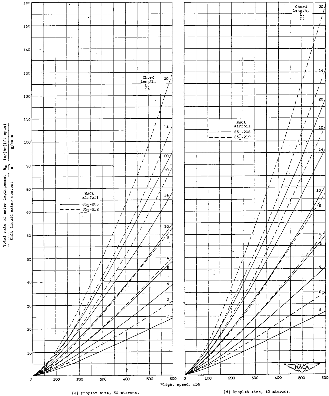
Figure 3. - Concluded. Rate of water impingement. Angle of attack, 4^\circ ; altitude, 20,000 feet; most probable icing temperature, -11^\circ F.
