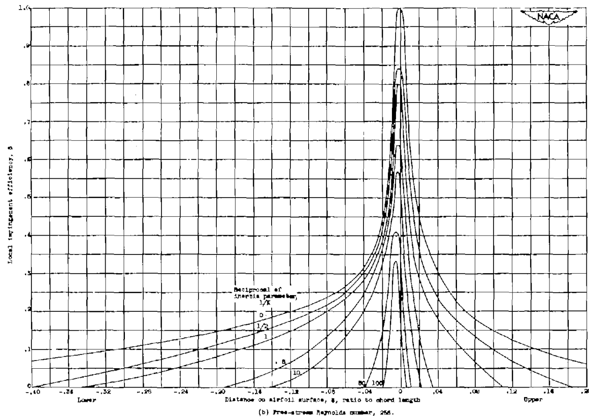
Figure 10. - Continued. Local impingement efficiency. NACA 851-212 airfoil; angle of attack, 4^\circ . (Reproduced from fig. 10, ref. 10.)
