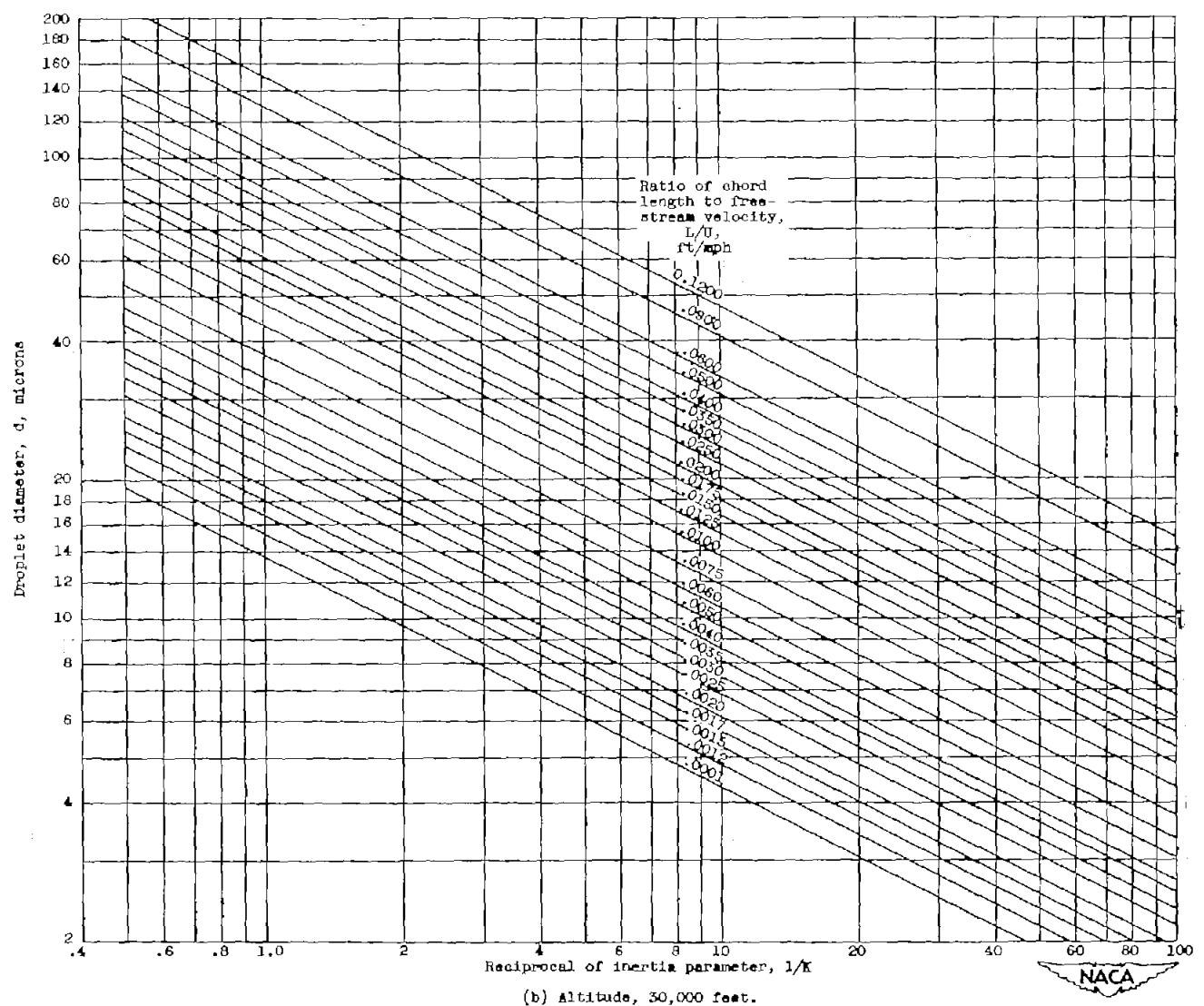
Figure 13. - Concluded. Droplet diameter as function of reciprocal of inertia parameter.
