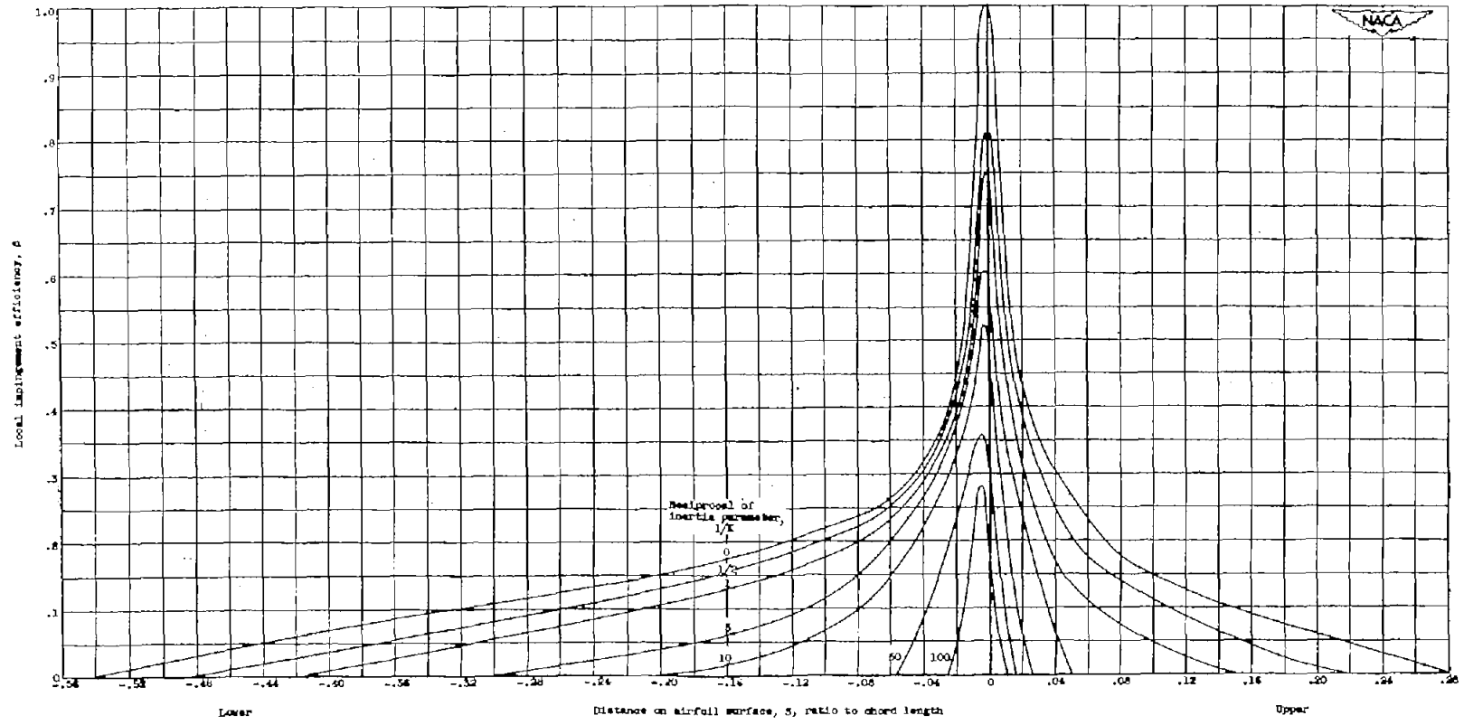
(a) Free-stream Reynolds number, 16. Figure 10. - Local impingement efficiency. NACA 651-212 airfoil; angle of attack, 4°. (Reproduced from fig. 10, ref. 10.)
