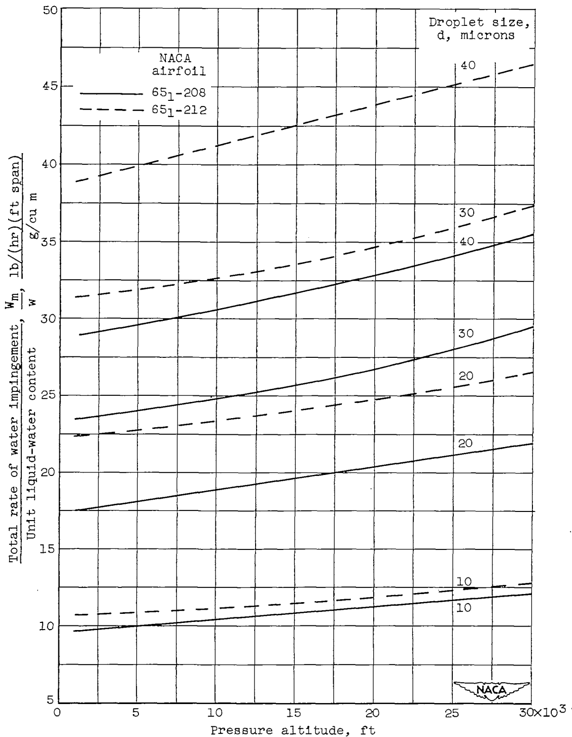
Figure 4. - Effect of altitude on rate of water impingement. Chord length, 10 feet; airplane speed, 300 miles per hour; most probable icing temperature, (see appendix B).
