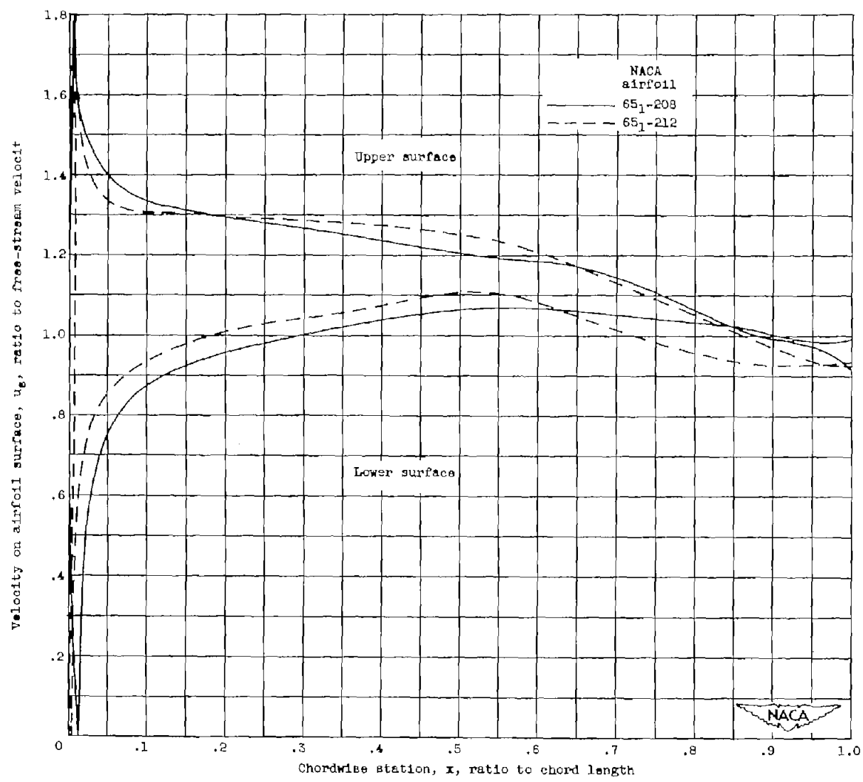
Figure 11. - Velocities on surface of two NACA 65-series airfoils. Angle of attack, 4°; free-stream Mach number, 0.2.
