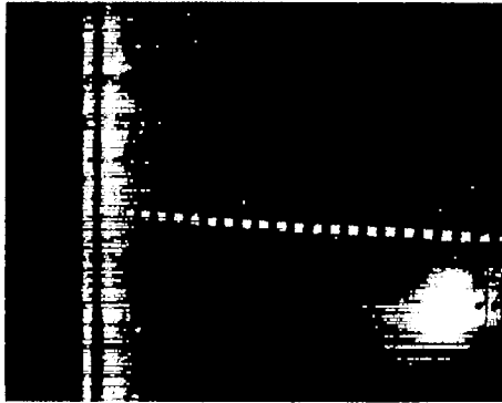
(a) Icing time, 4 minutes. Drag coefficient, 0.0133.
