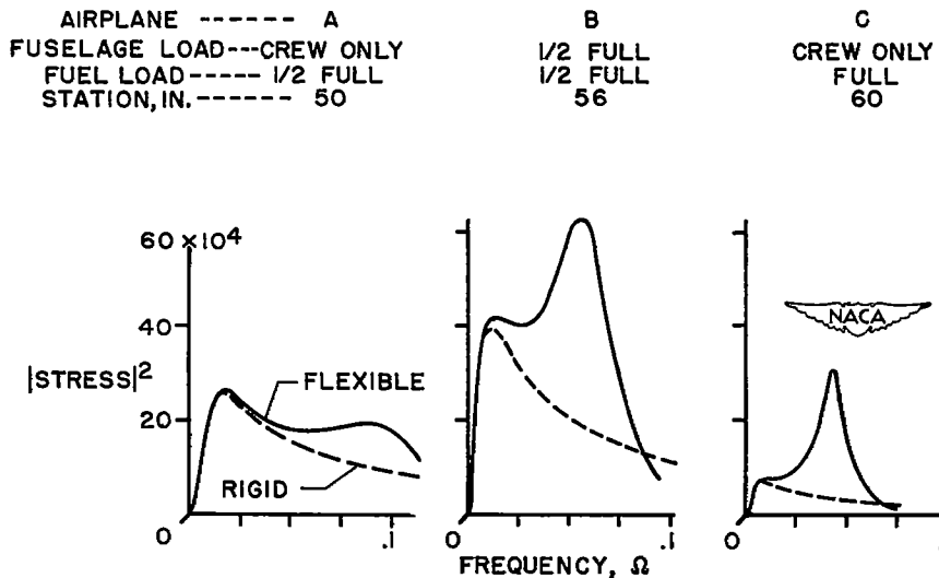
Figure 7.- Transfer functions.
