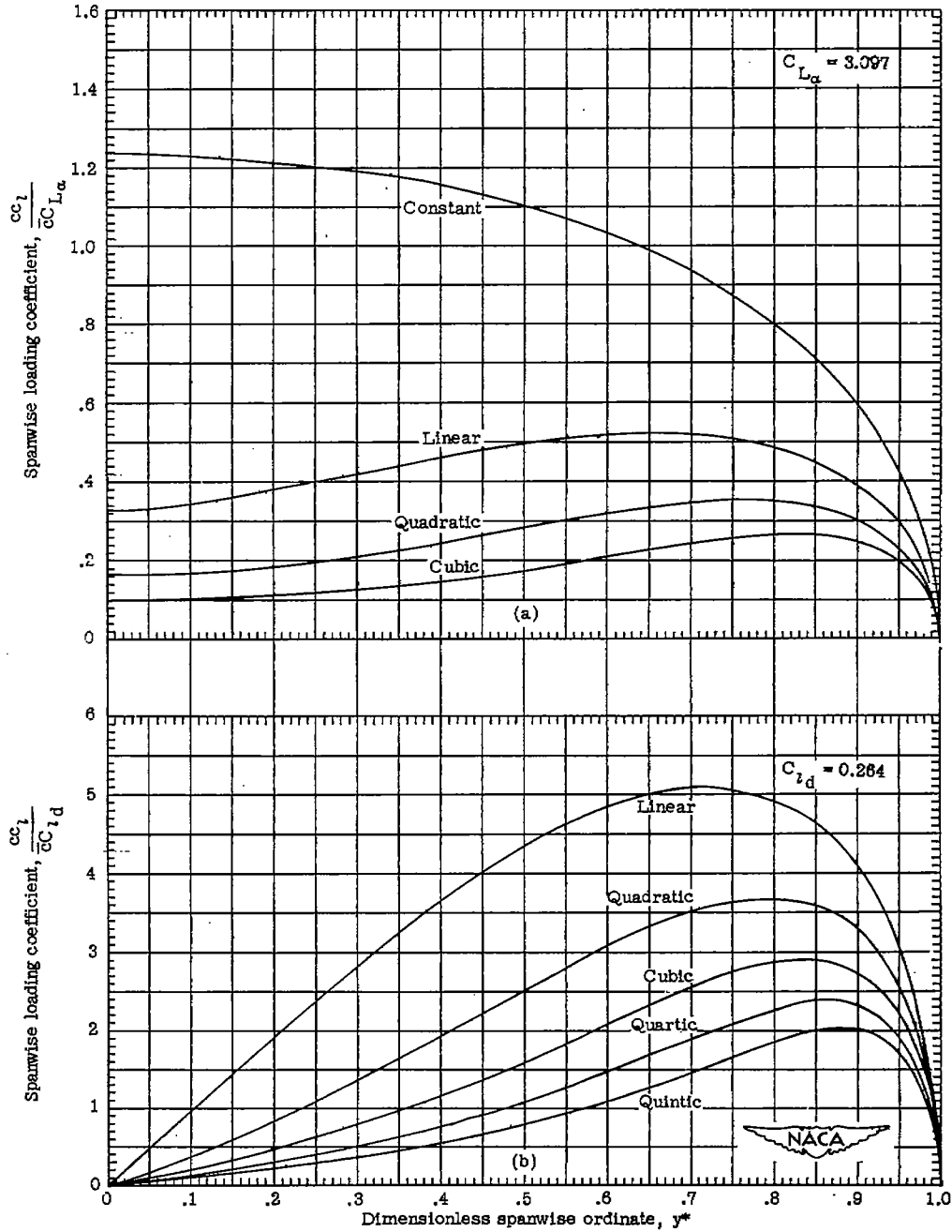
(a) Symmetrical lift distributions.
