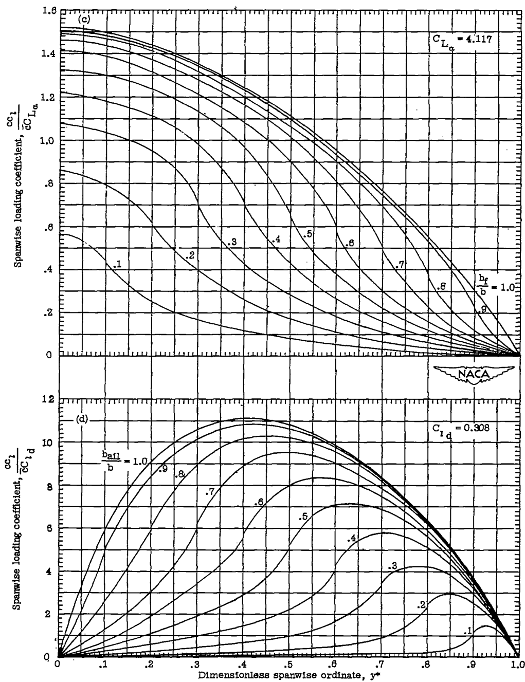
(c) Lift distribution for inboard flap.
