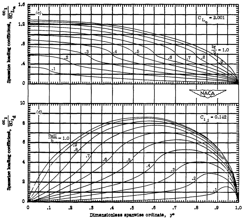
(c) Lift distribution for inboard flap.
