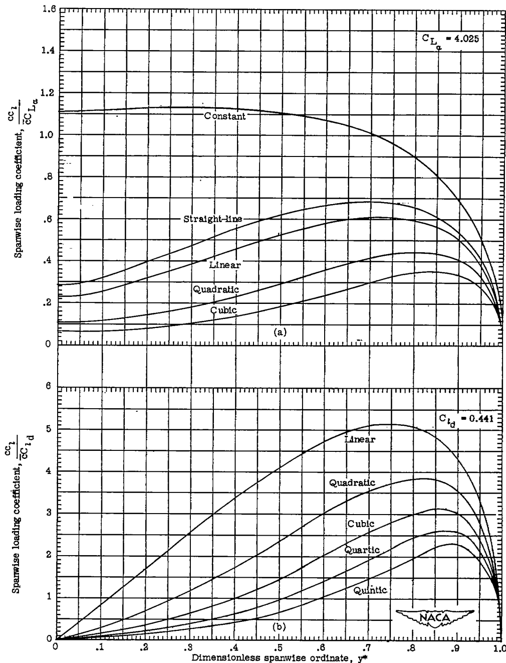
(a) Symmetrical lift distributions.
