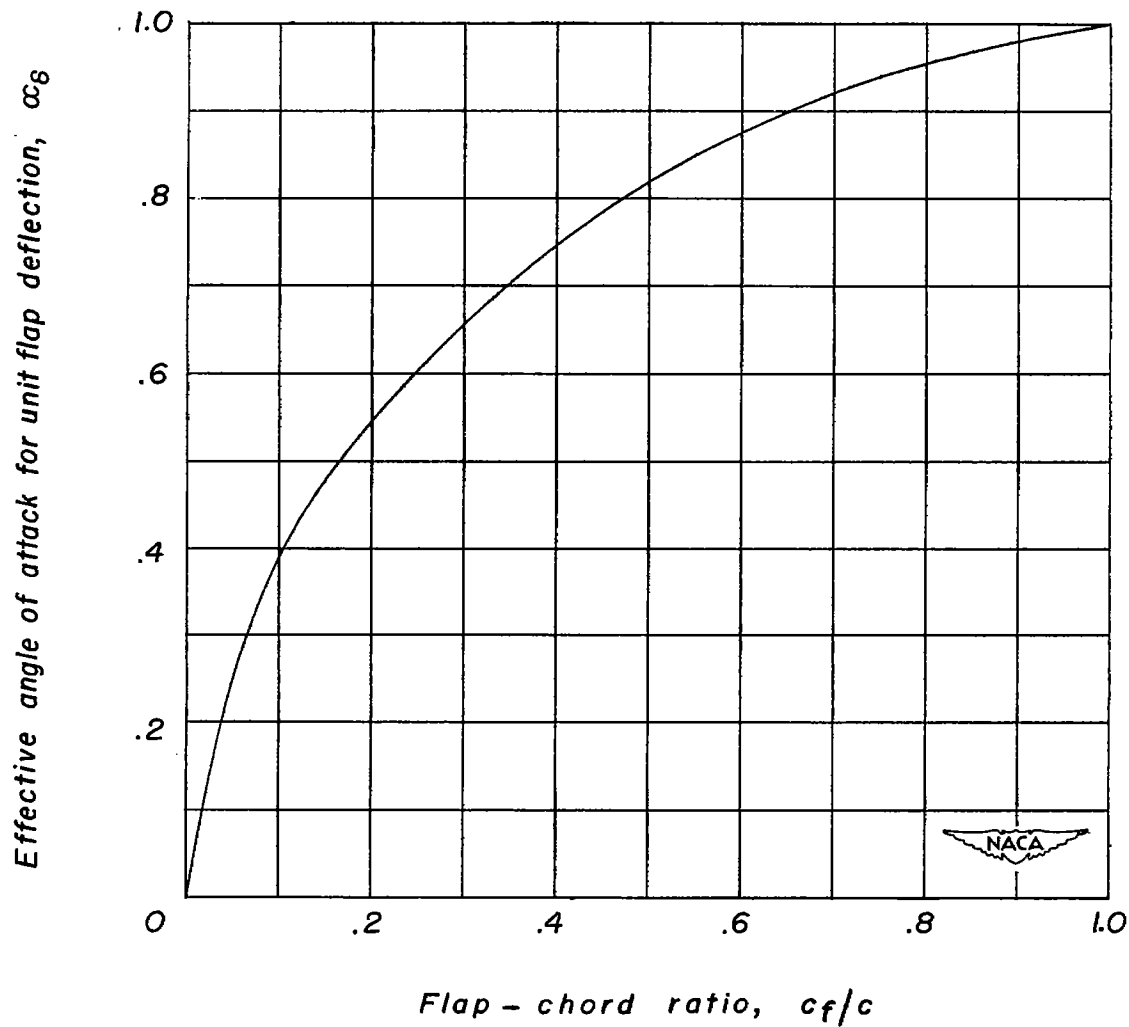
Figure 21.- Variation of flap effectiveness with flap-chord ratio.
