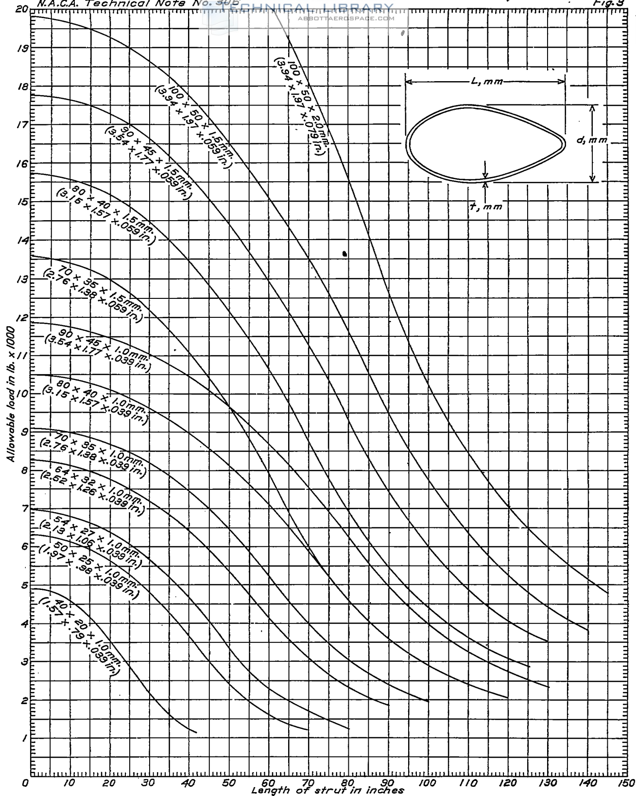
Fig. 3 Strength curves for carbon steel streamline tubes as columns. Y.P. in compression = 36,000 lb./sq.in. Fixity coef. = C=1 E=28,000,000 lb./sq.in.
