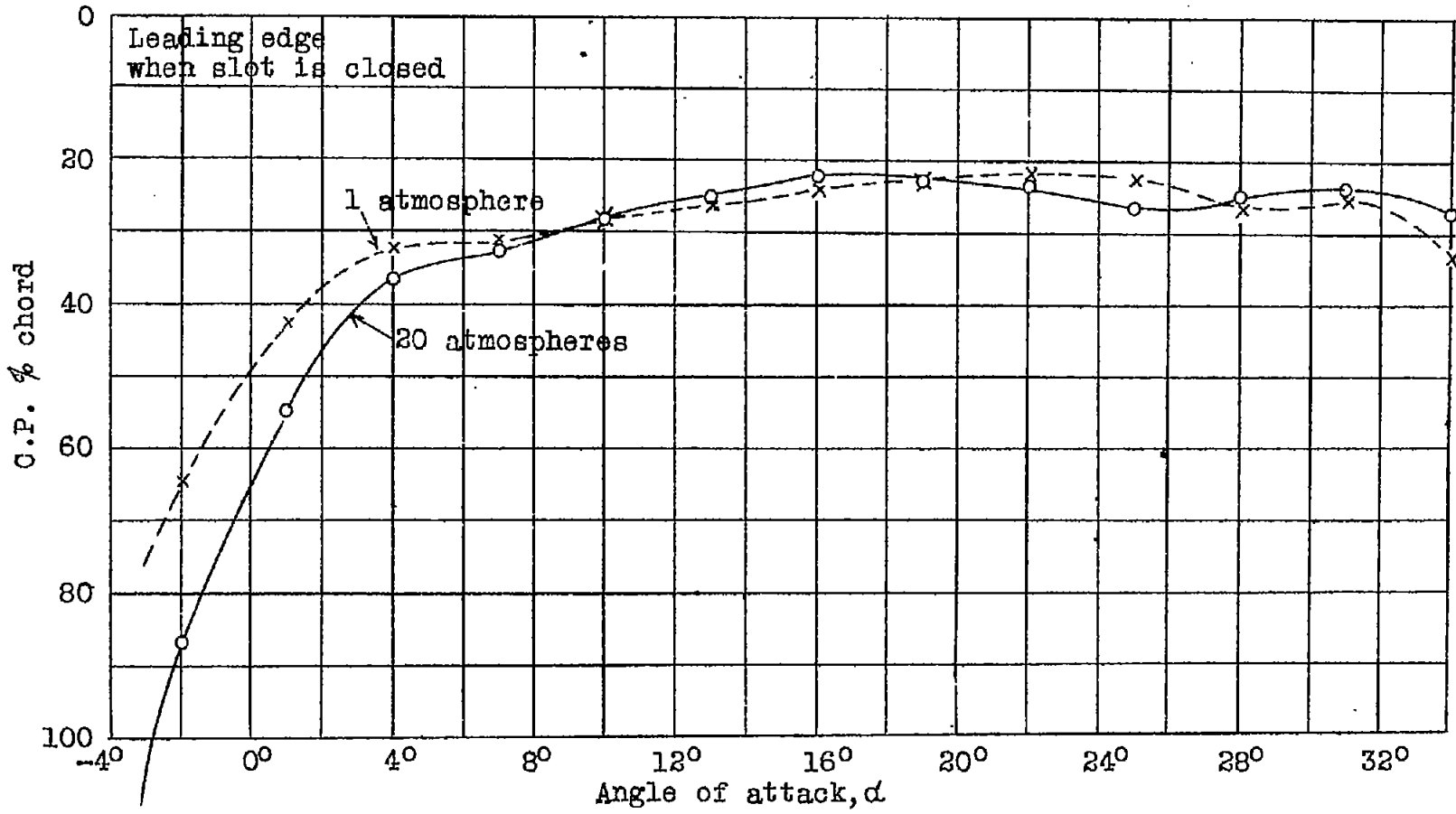
Fig.11 Center of pressure. Slotted R.A.F. 31 airfoil.
