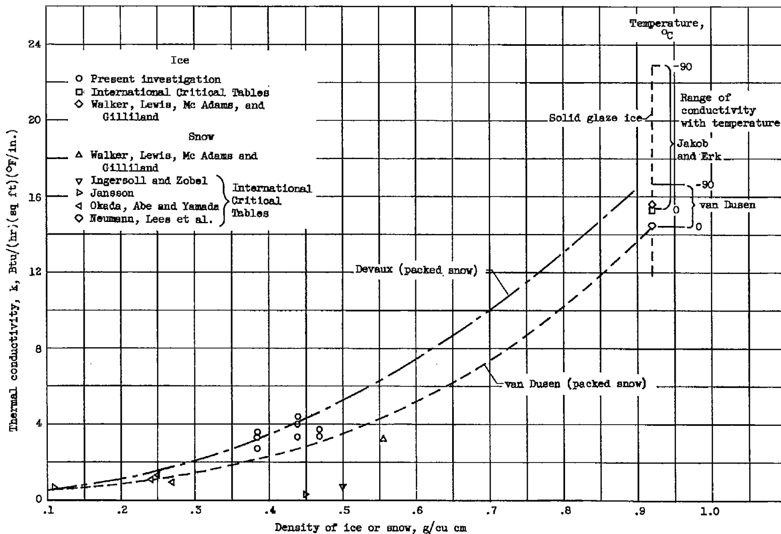
Figure 4. - Thermal conductivity of ice and packed snow as function of density.
