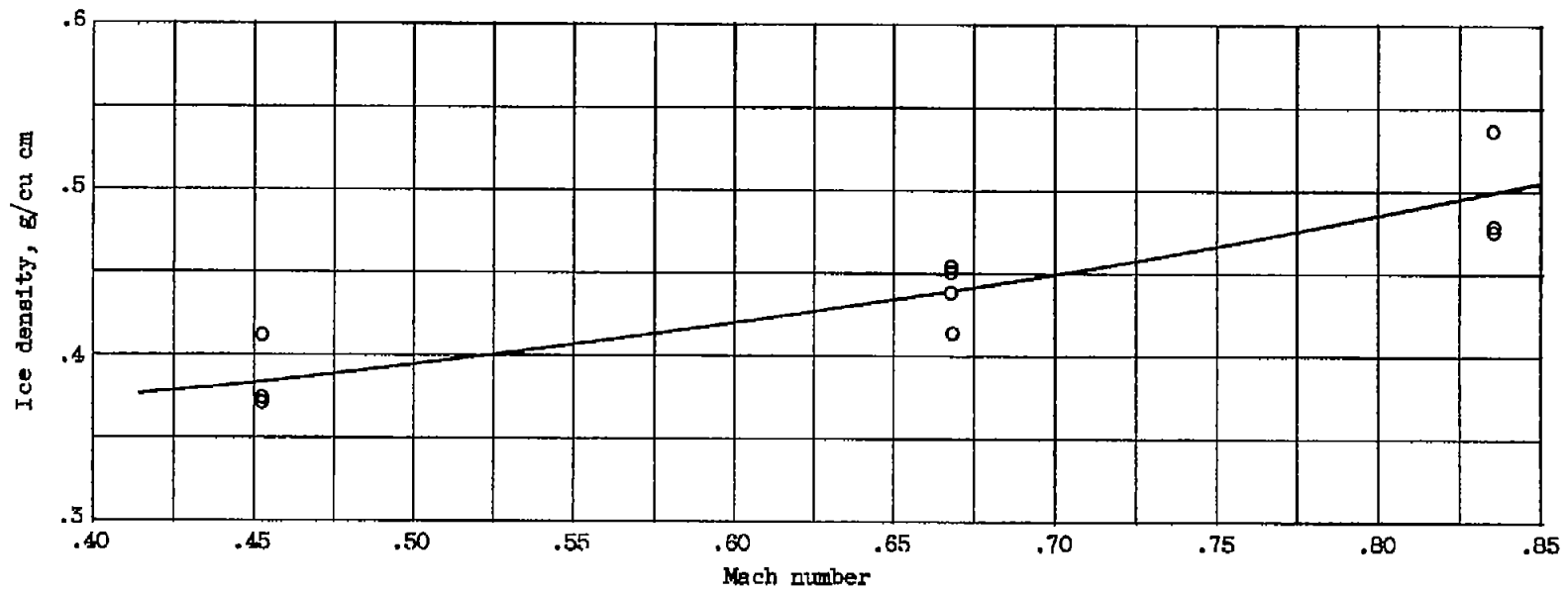
Figure 3. - Density of ice formed by condensation from air stream as a function of Mach number.
