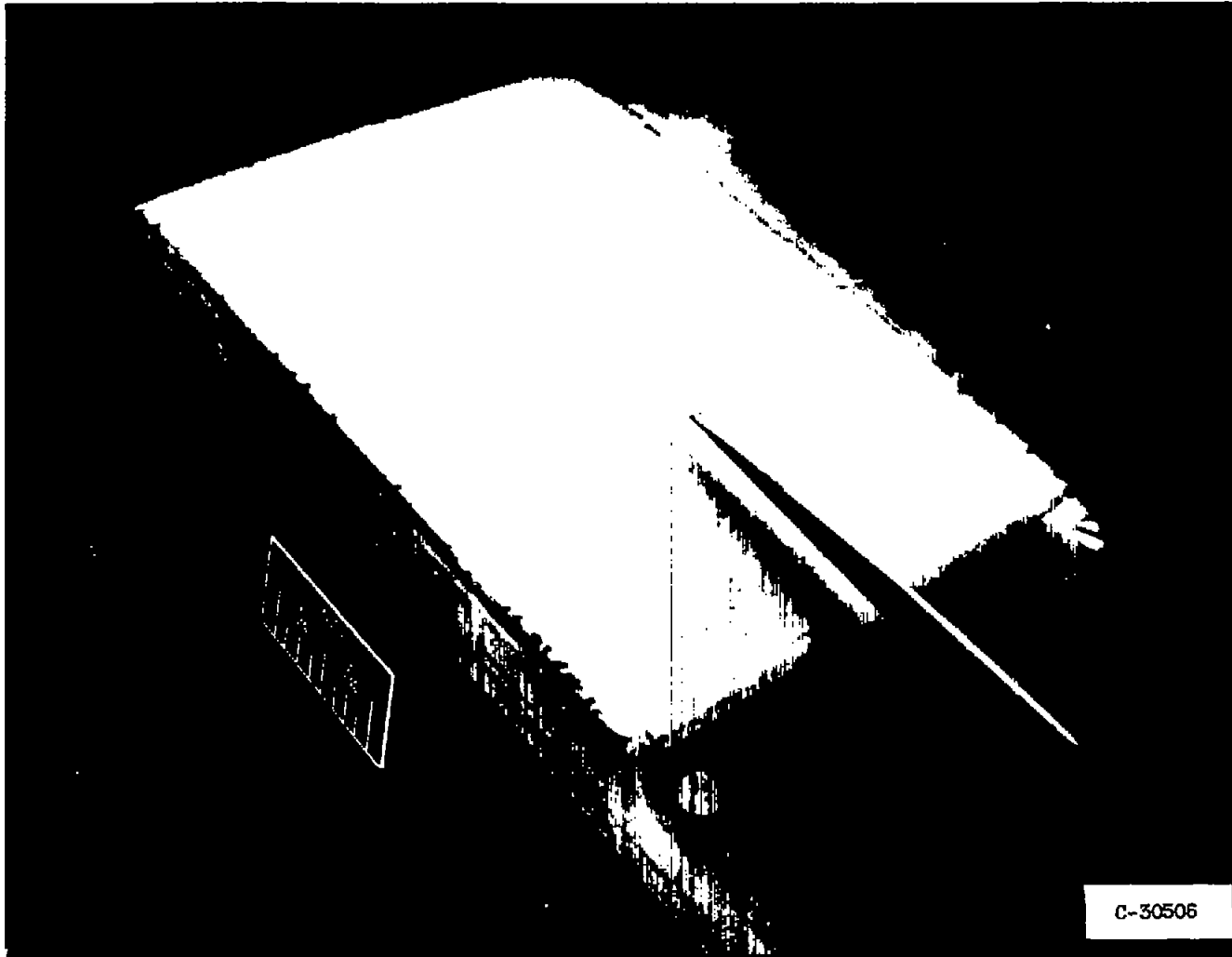
Figure 2. - Ice formation deposited on flat-plate model by condensation of water vapor from air stream.
