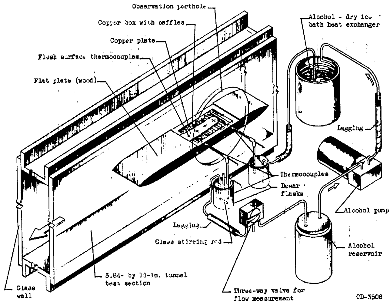
Figure 1. - Schematic diagram of flat-plate model and alcohol system.
