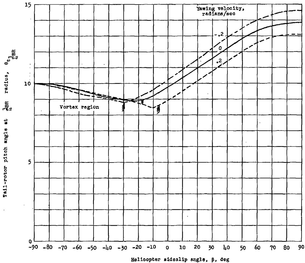
Figure 6.- Effect of helicopter rate of yaw on tail-rotor pitch required for trim at different sideslip angles ( V = 20 knots). Vortex region for each curve is to the left of the flag.
