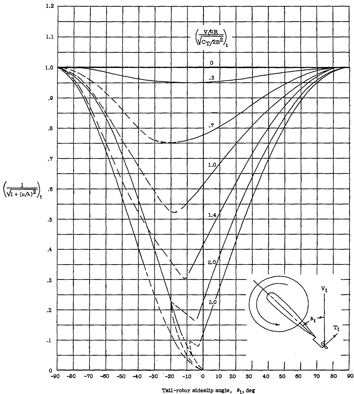
Figure 3.- Chart for determining \left(\frac{1}{\sqrt{1 + (\mu/\lambda)^2}}\right)_t . Dashed lines indicate vortex region.
