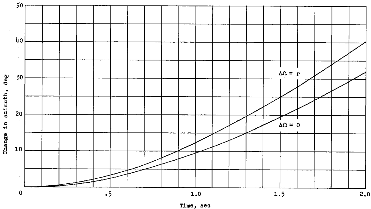
Figure 7.- Response of sample helicopter in hovering to a 1-inch step displacement of pedals.
