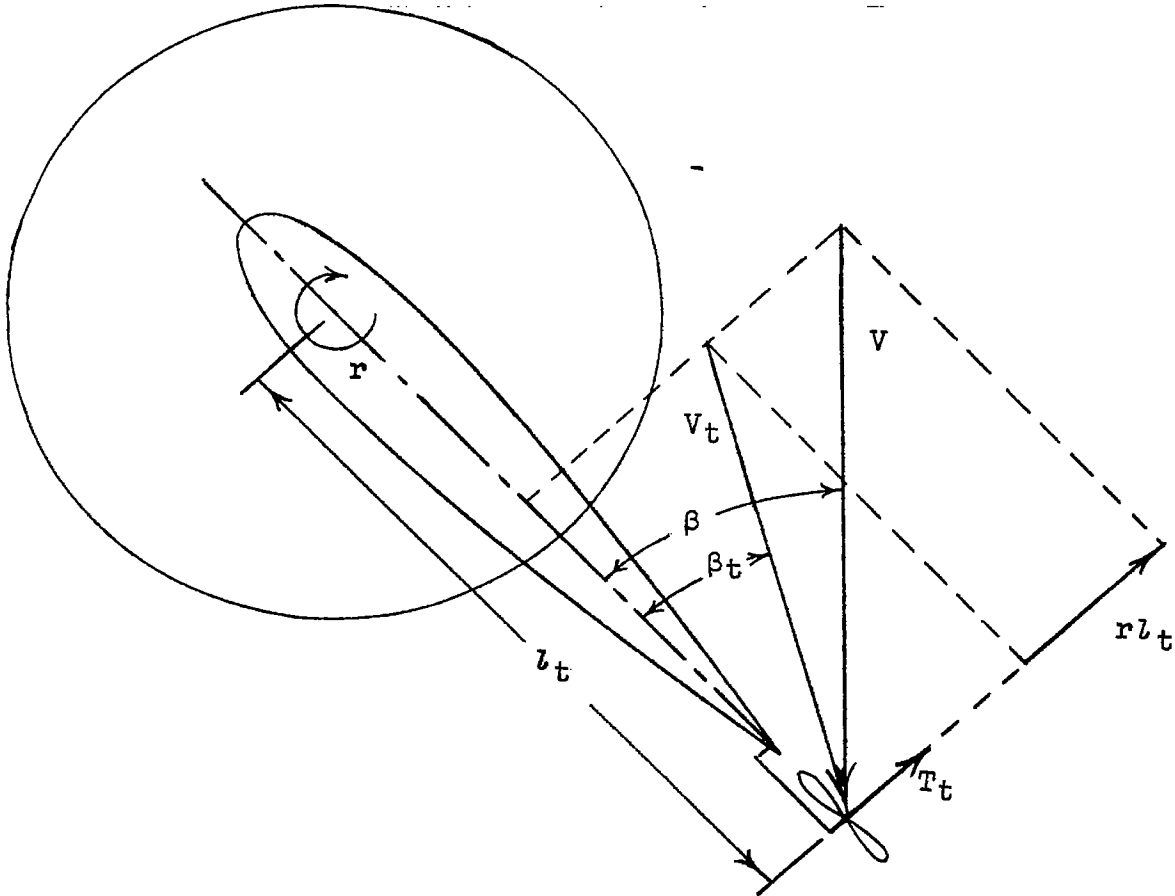
Figure 10.- Sketch showing geometry for converting from V , \beta , and r
