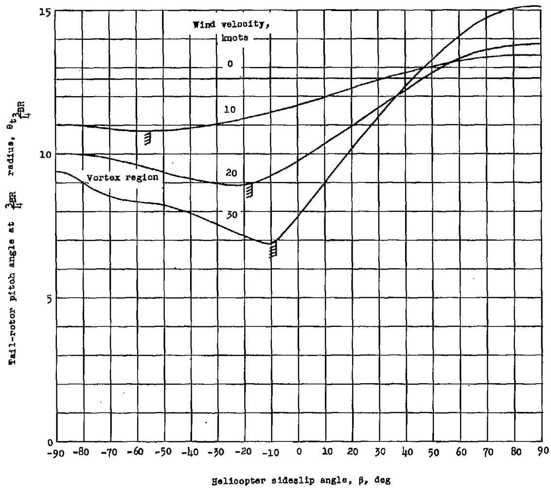
Figure 5.- Effect of forward speed and sideslip angle on tail-rotor pitch required for sample helicopter to hover over a spot. Vortex region for each curve is to the left of the flag.
