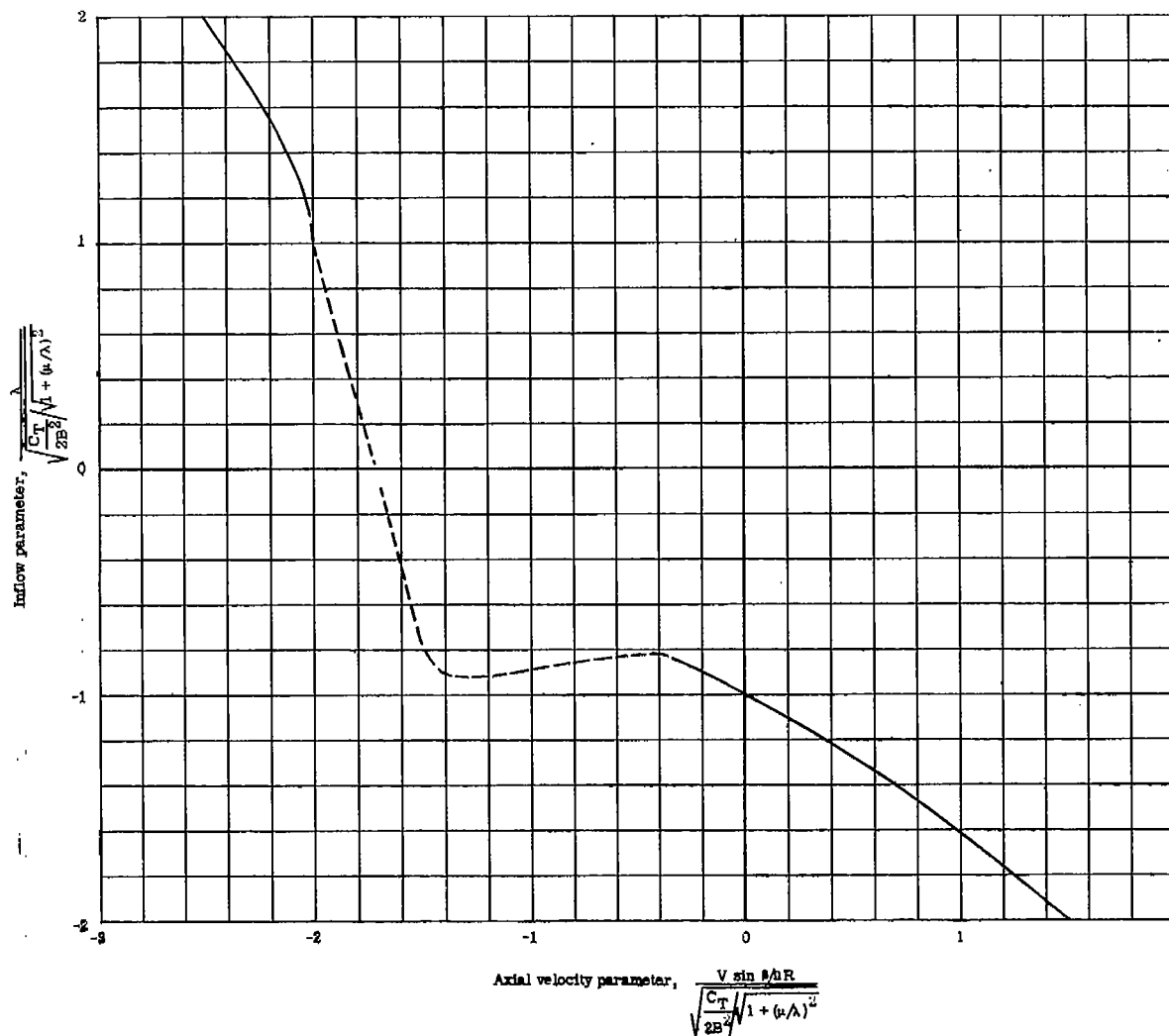
Figure 2.- Relation between inflow parameter and axial velocity parameter used in this paper. Dashed line indicates vortex region.
