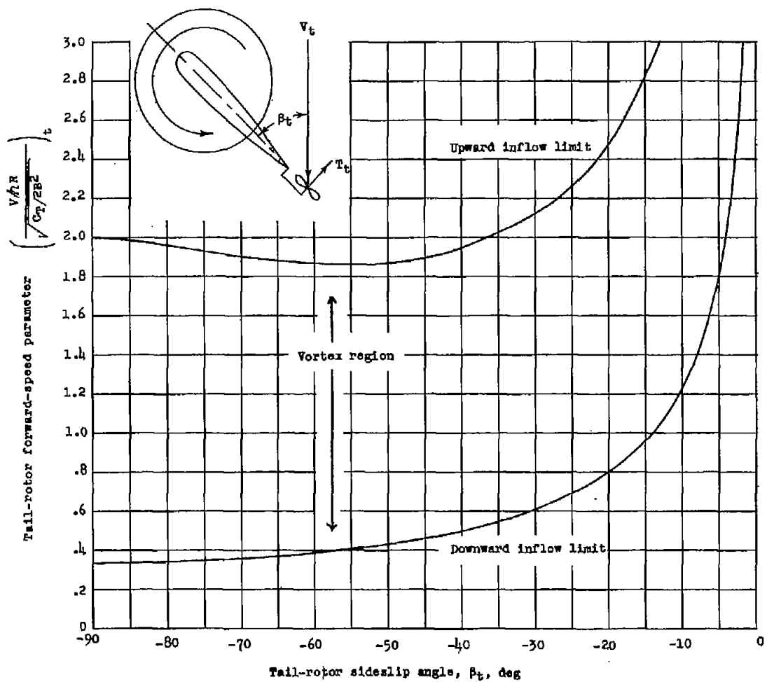
Figure 4.- Chart showing extent of vortex region in terms of tail-rotor forward-speed parameter \left(\frac{V/\Omega R}{C_t/2B^2}\right)_t and tail-rotor sideslip angle \beta_t .
