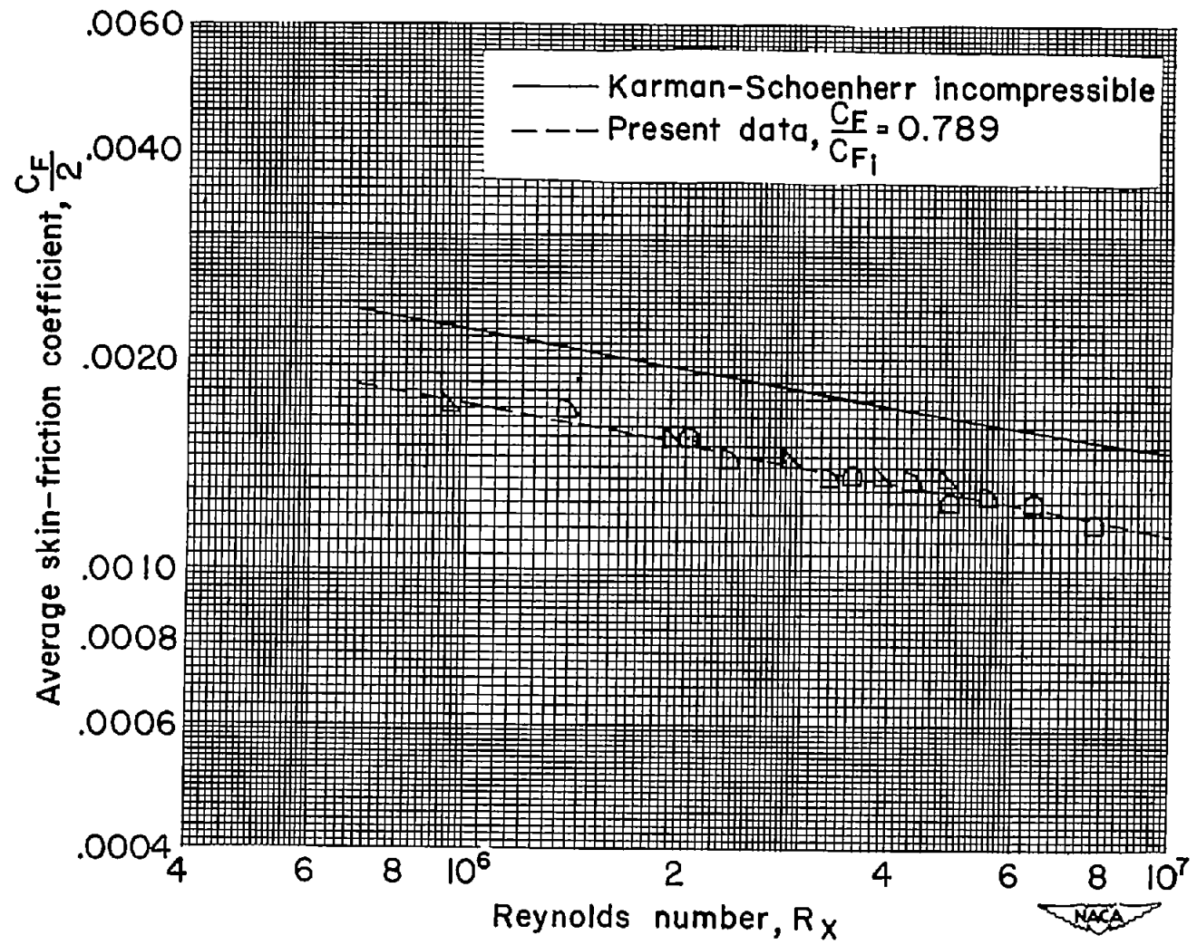
(b) Mach number 2.27.
