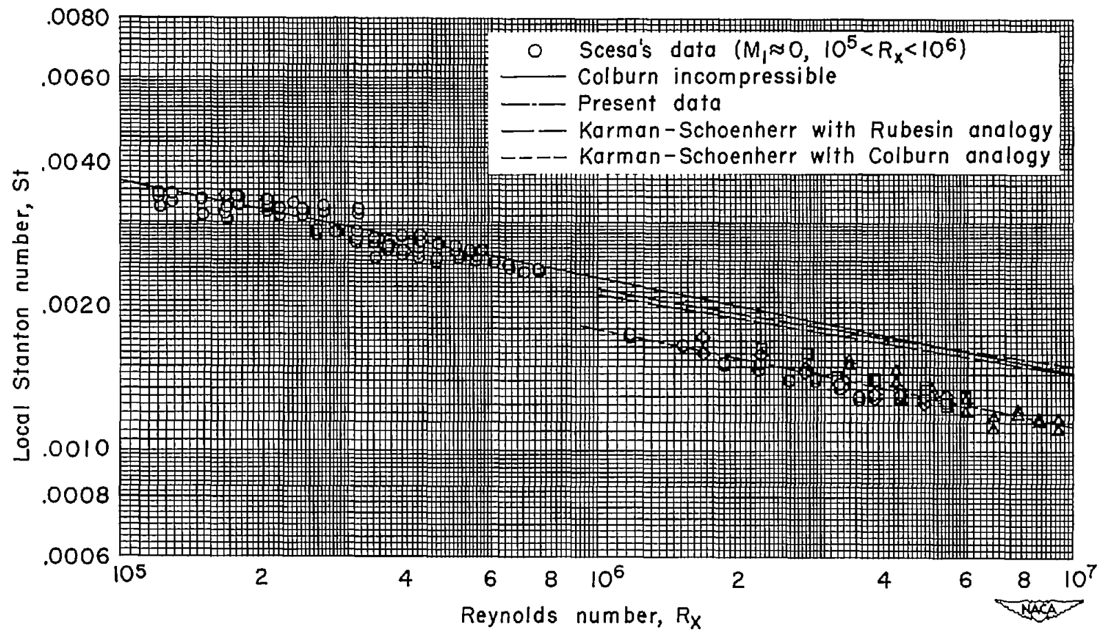
(a) Mach number 1.69, T_w/T_1 = 1.65 .
