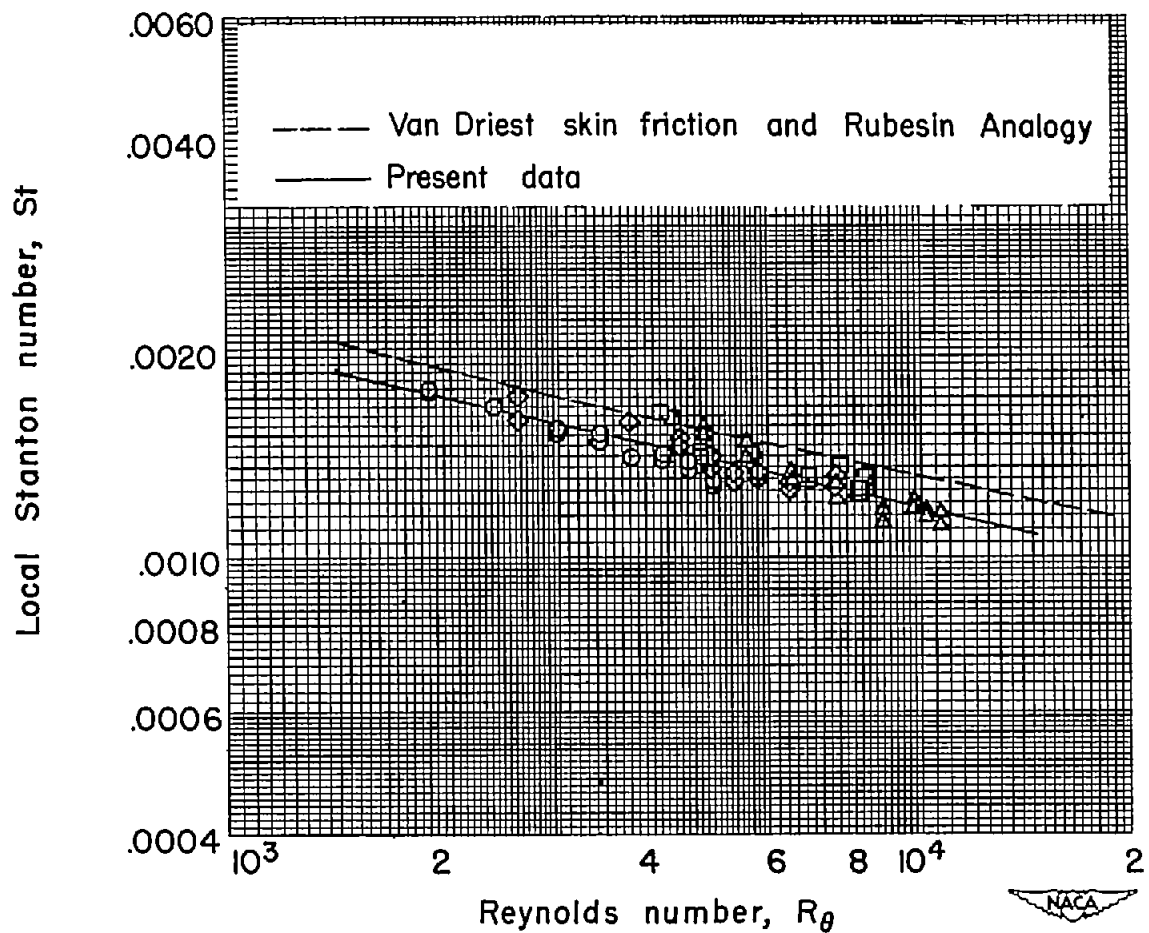
(a) Mach number 1.69, T_w/T_1 = 1.65 .
