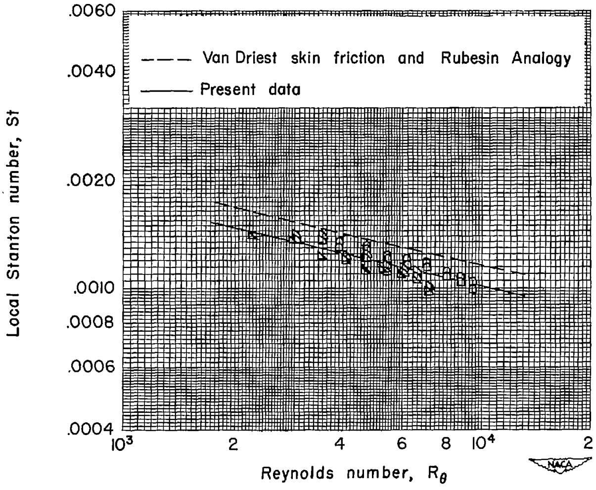
(b) Mach number 2.27, T_w/T_1 = 2.16 .
