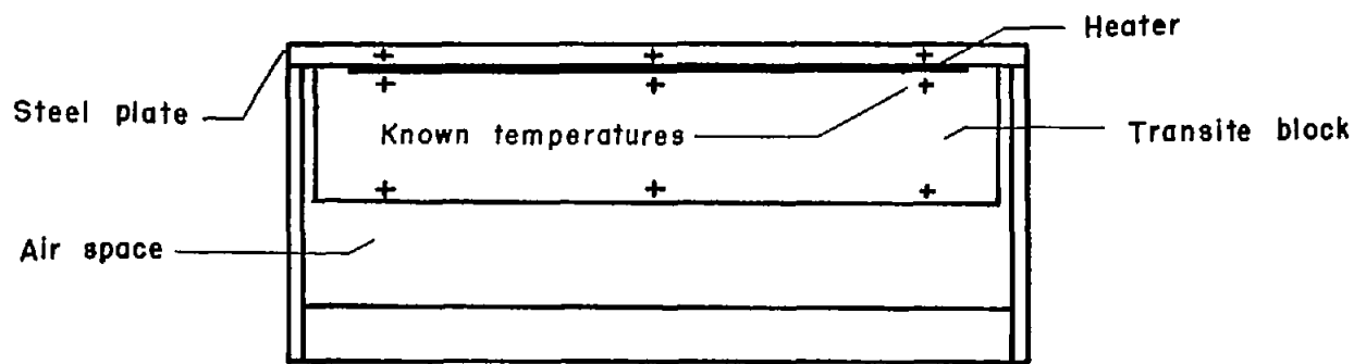
(b) Cross section A-A of flat-plate model. Figure 1.- Sketch of test section and model.
