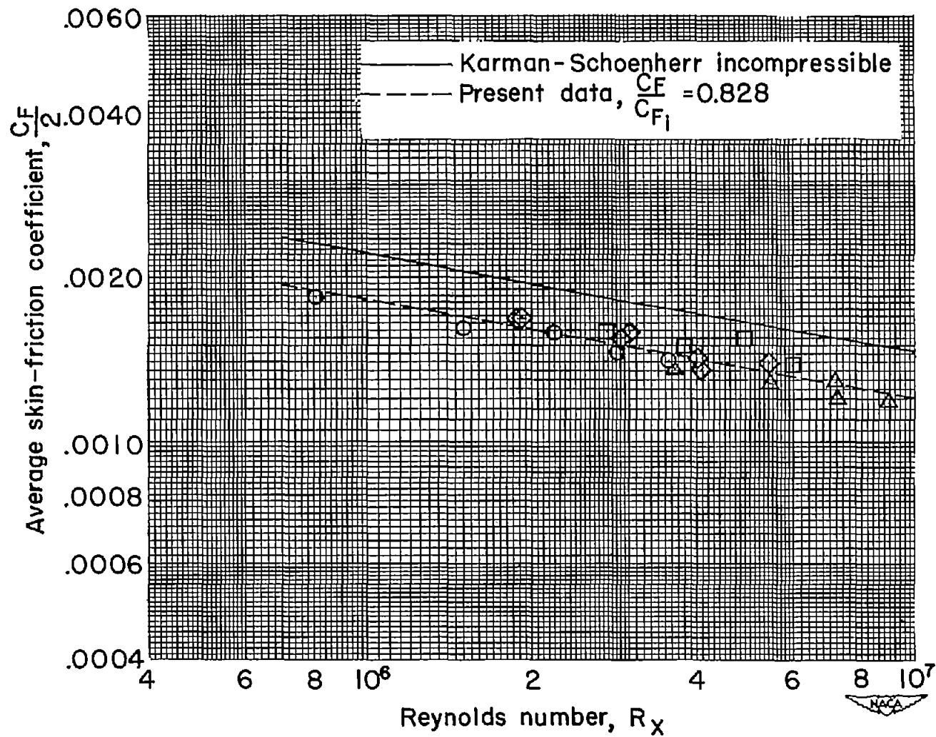
(a) Mach number 1.69.
