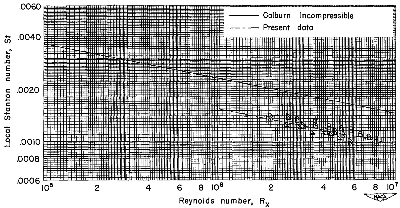
(b) Mach number 2.27, T_w/T_1 = 2.16 .
