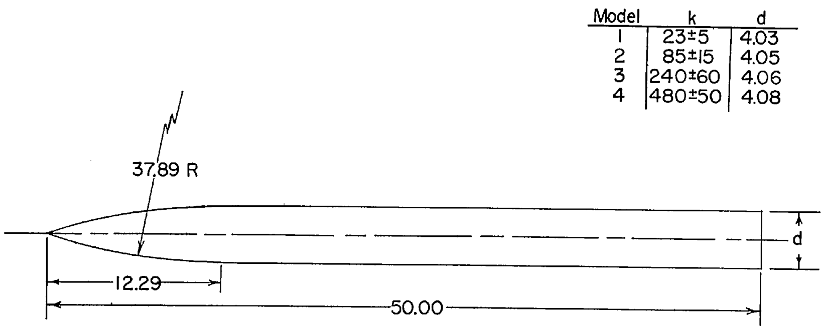
Figure 1.- Drawing of test model. All dimensions are in inches except as noted. k is rms roughness in microinches.
