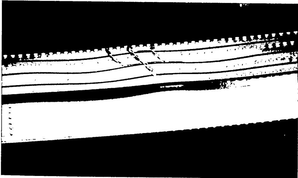
(a) Buckling.
