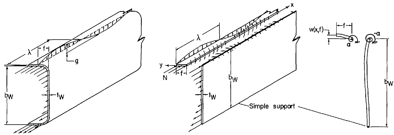
(a) Loads on channel. (b) Idealized channel. (c) Distortion of idealized channel.
