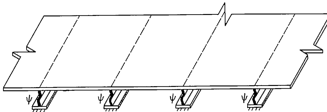
Figure 1.- Multiweb wing and structural idealization.
