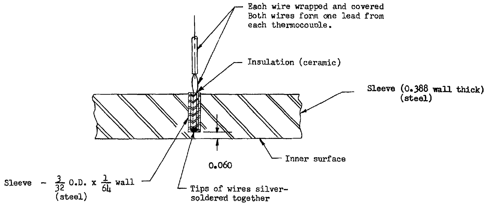
Figure 2.- Thermocouple installation.
