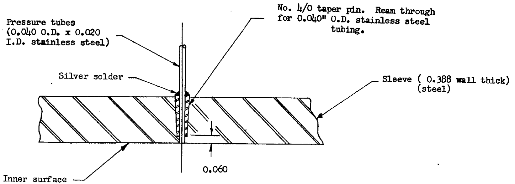
Figure 3.- Pressure tubes installation.
