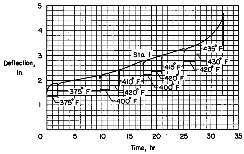
(e) Beam 7; test temperature varied; tip load, 4,175 lb. Beam temperature reduced to room temperature for 16 hours at each discontinuity. Tensile failure.
