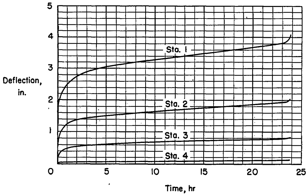
(b) Beam 4; test temperature, 375° F; tip load, 5,400 lb (85 percent of load required to produce immediate failure at 375° F). Tensile failure.
