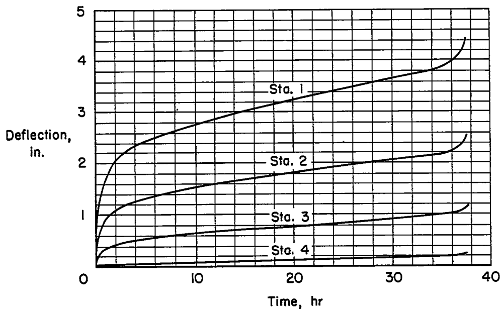
(c) Beam 5; test temperature, 425° F; tip load, 3,750 lb (61 percent of load required to produce immediate failure at 425° F). Tensile failure.
