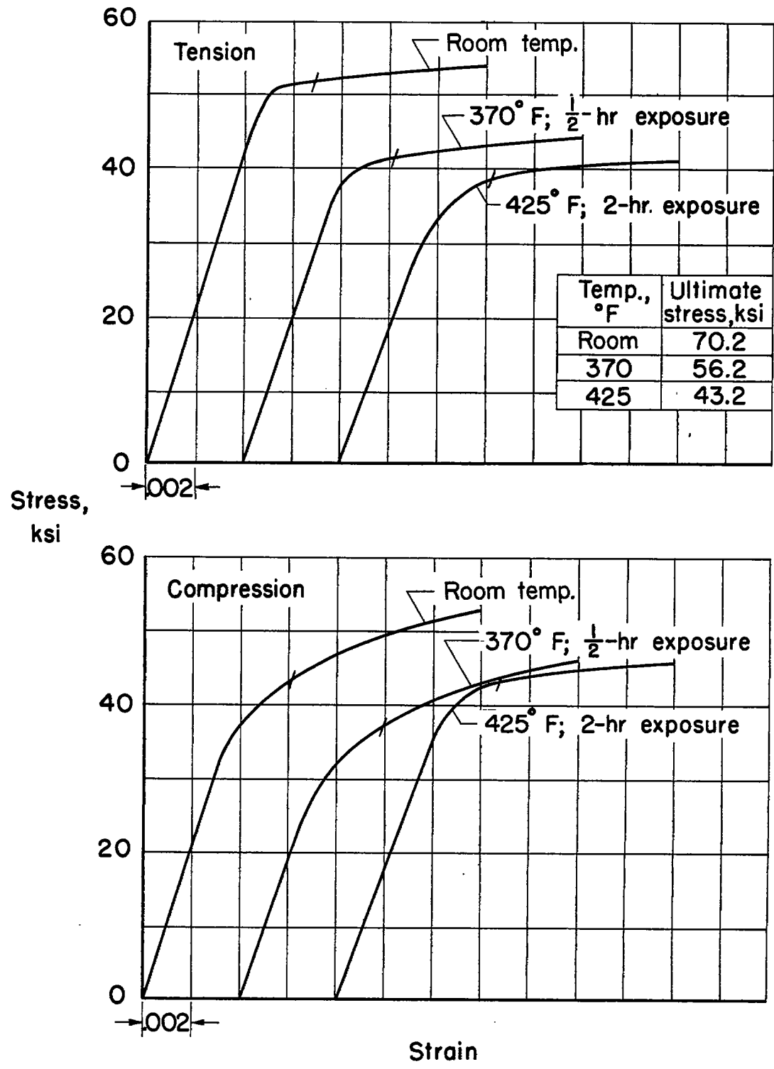
Figure 5.- Tensile and compressive stress-strain curves for 24S-T3 aluminum alloy. Specimen thickness, 1/8 inch; strain rate, 0.002 per minute.
