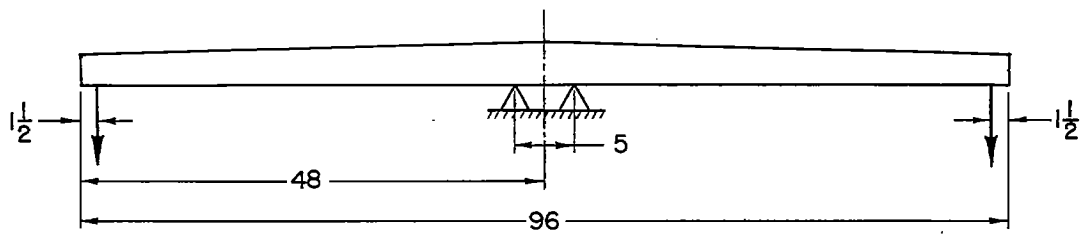
Figure 1.- View of box beam showing support locations and points of application of loads.
