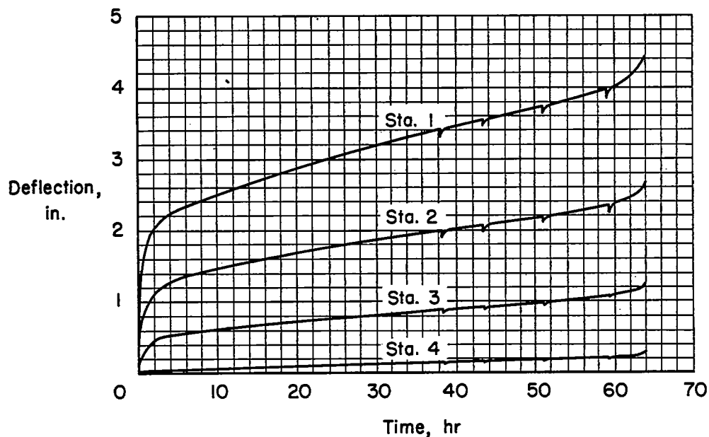
(d) Beam 6; test temperature, 425° F; tip load, 3,400 lb (56 percent of load required to produce immediate failure at 425° F). Beam temperature reduced to room temperature for 16 hours at each discontinuity. Compressive failure.
