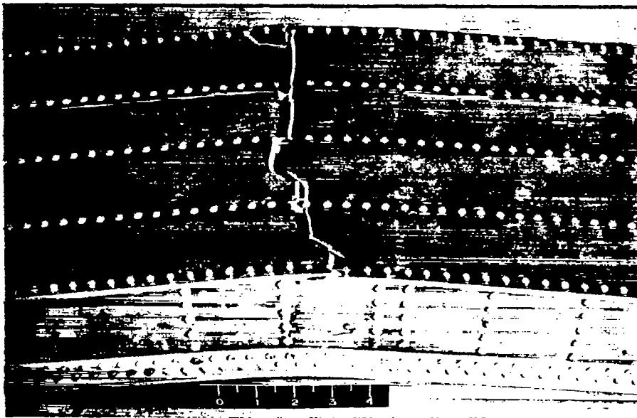
(b) Tensile failure, top cover plate. L-81512
