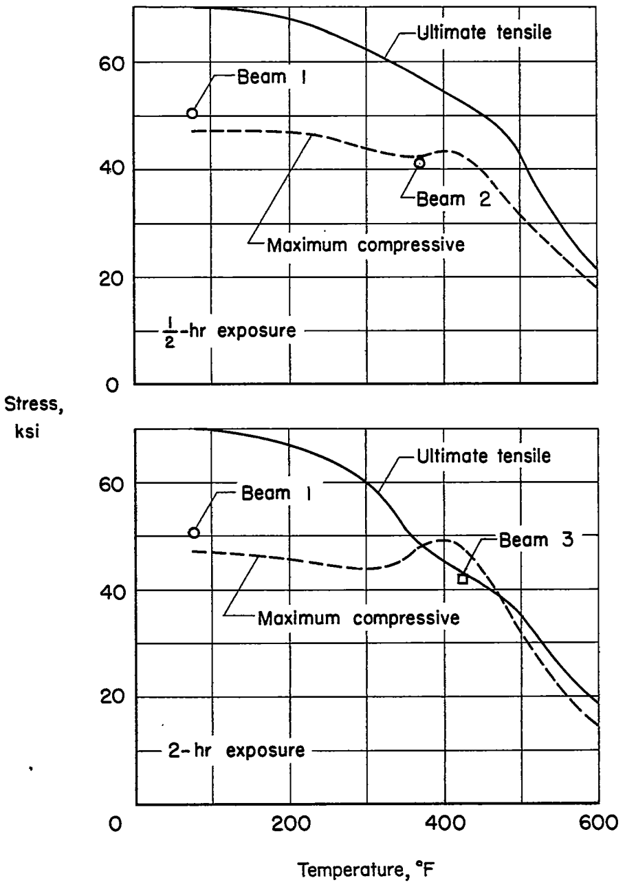
Figure 6.- Variations of ultimate tensile stress and maximum compressive stress with temperature for 24S-T3 aluminum-alloy box beams. (Box-beam static-strength test results included.)
